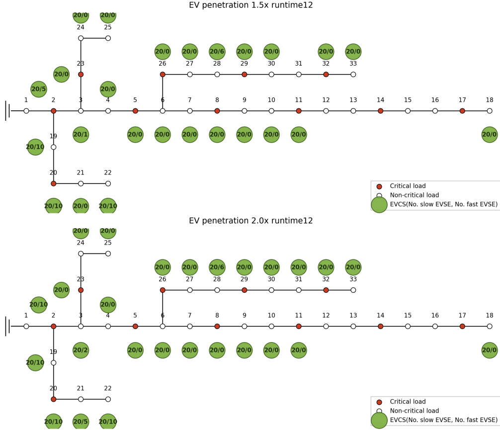
Figure 2: Runtime12 directional topology maps, part 2: EV-penetration runs.
