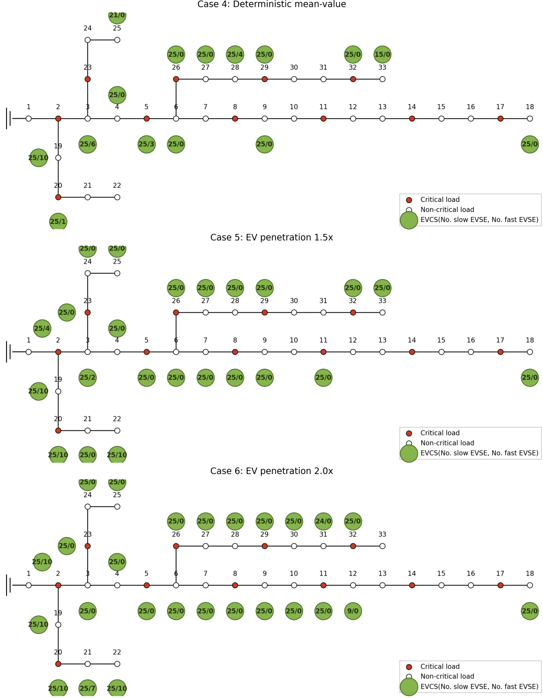
Figure 4: Paper-like case 4/5/6 topology maps: deterministic mean-value and EV-penetration cases.
