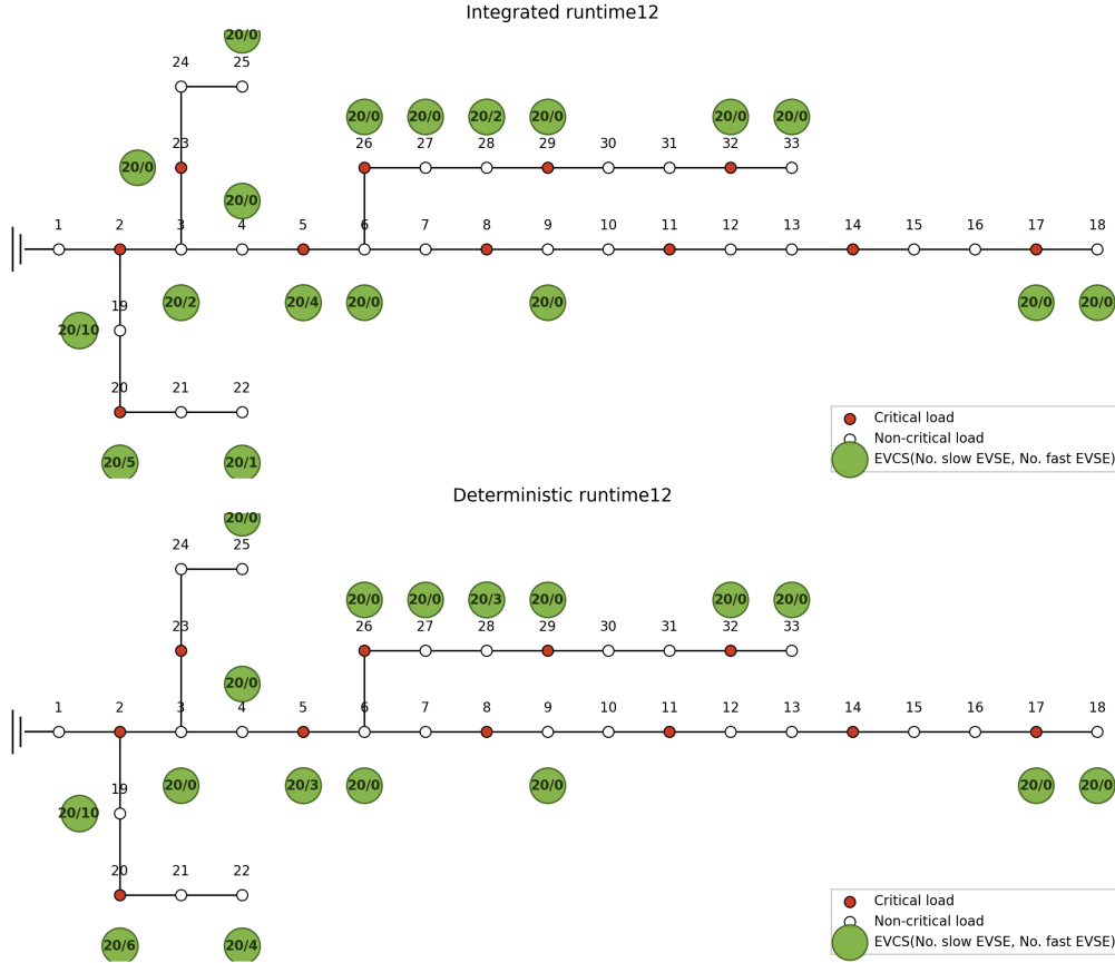
Figure 1: Runtime12 directional topology maps, part 1: integrated and deterministic runs.
