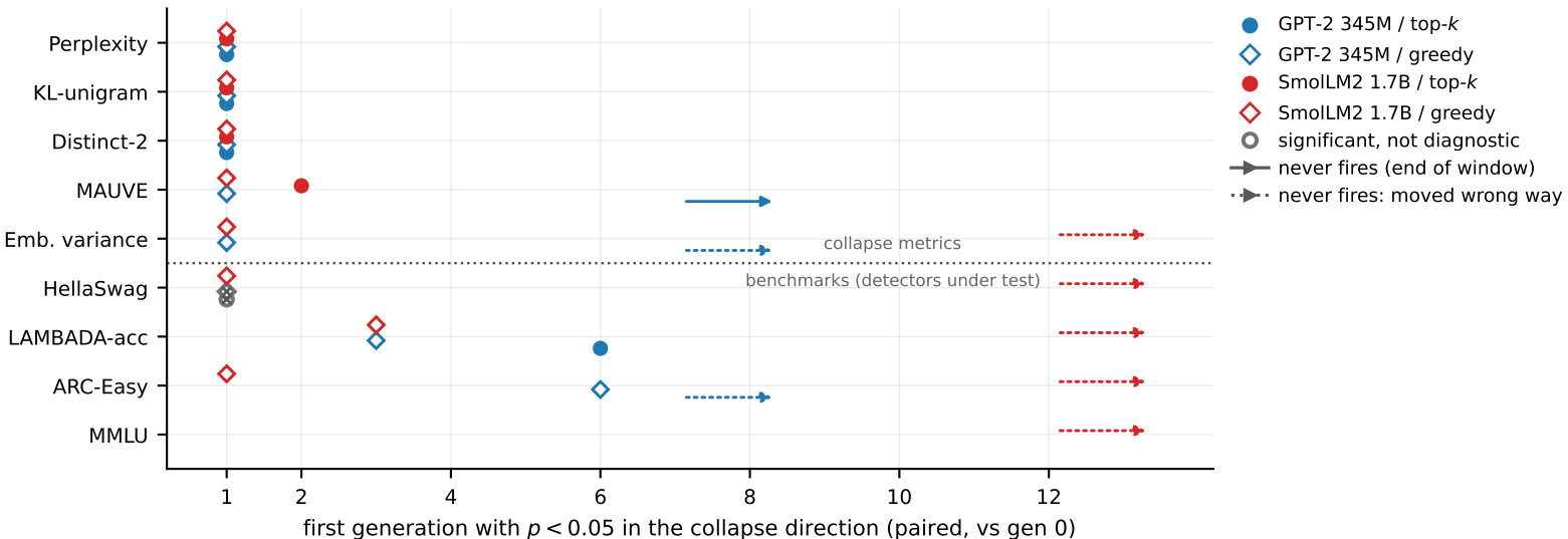
Diversity and distributional metrics fire at generation 1; benchmarks lag or never fire
