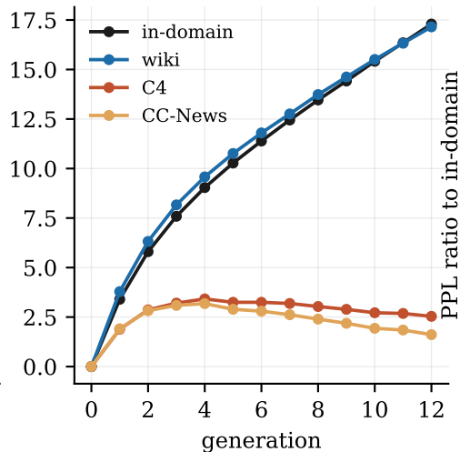
SmolLM2 1.7B / top-k
