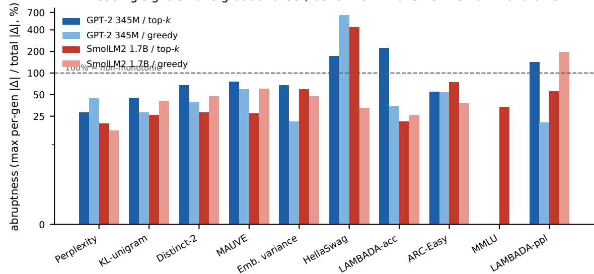
Leading signals have gradual onset; benchmark movement is non-monotonic
