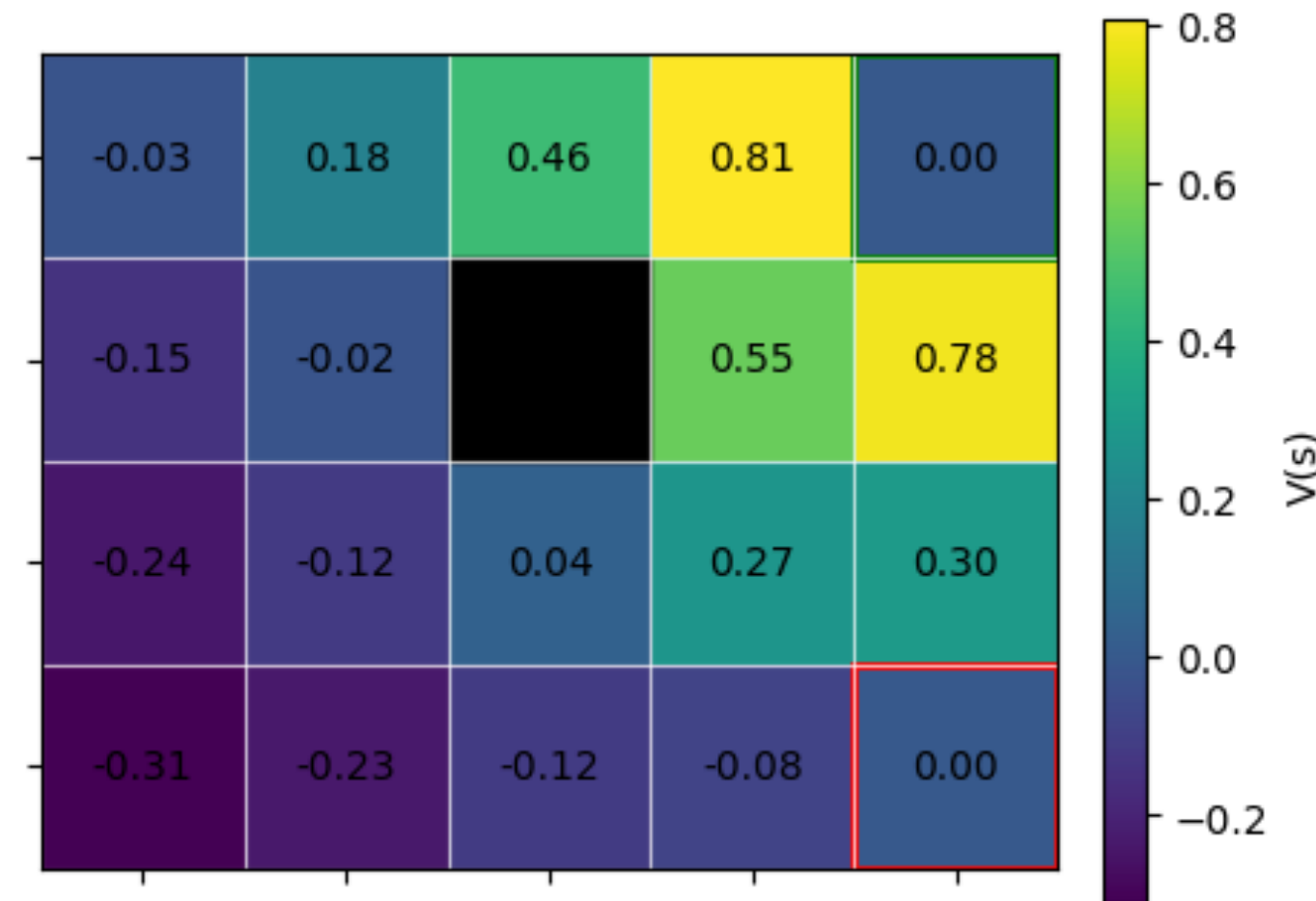
Optimal V^*(s) , calculated with DP
