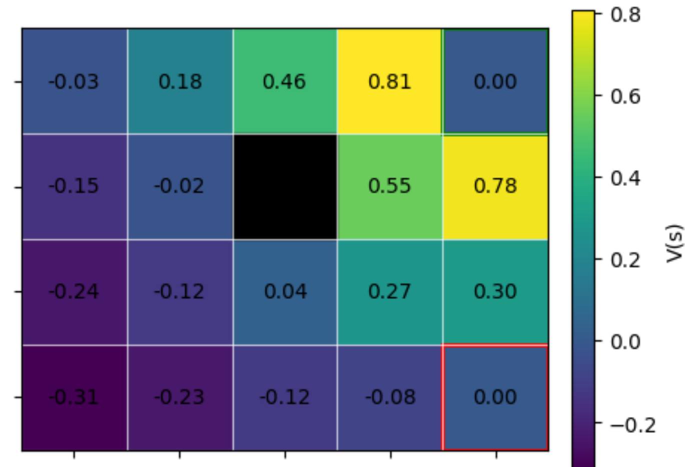
Optimal V^*(s) , calculated with DP
