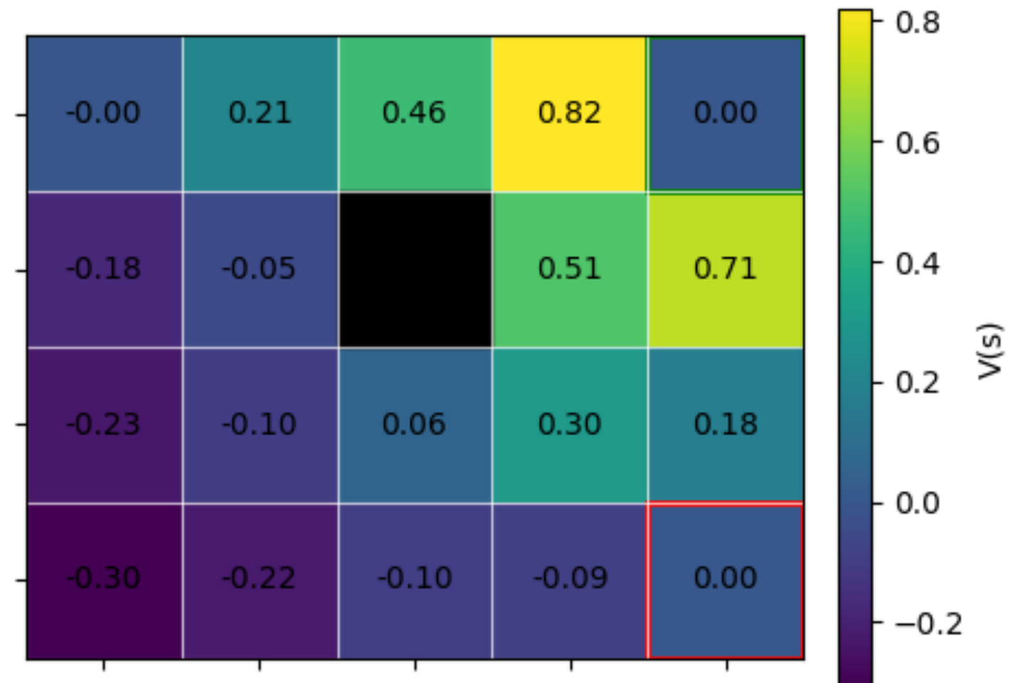
Optimal V^*(s) , calculated with Q-Learning
