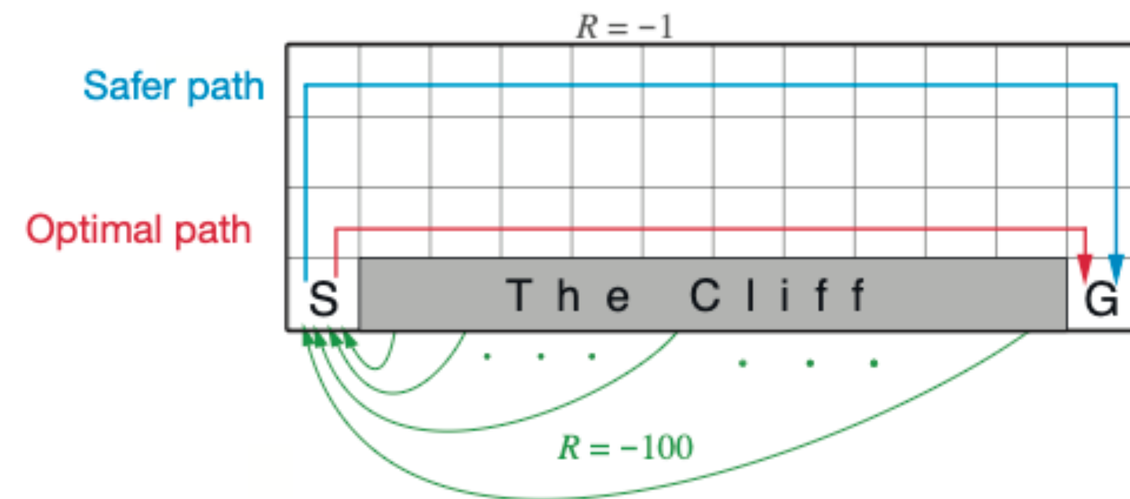
Figure courtesy of Sutton and Barto (2018) pg. 132.
