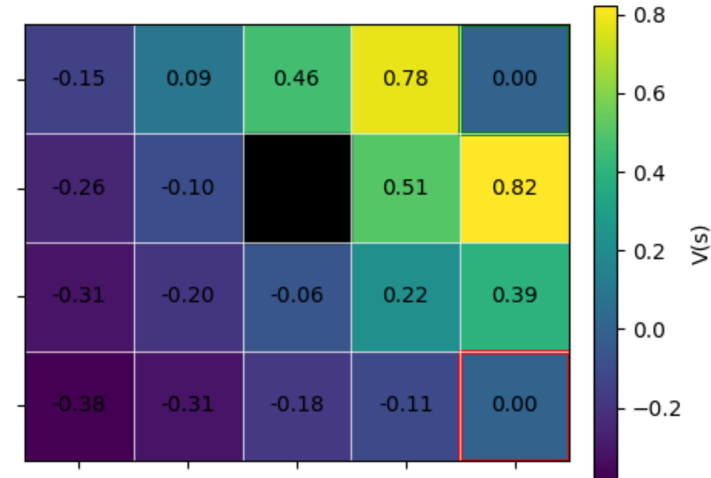
Optimal V^*(s) , calculated with SARSA
