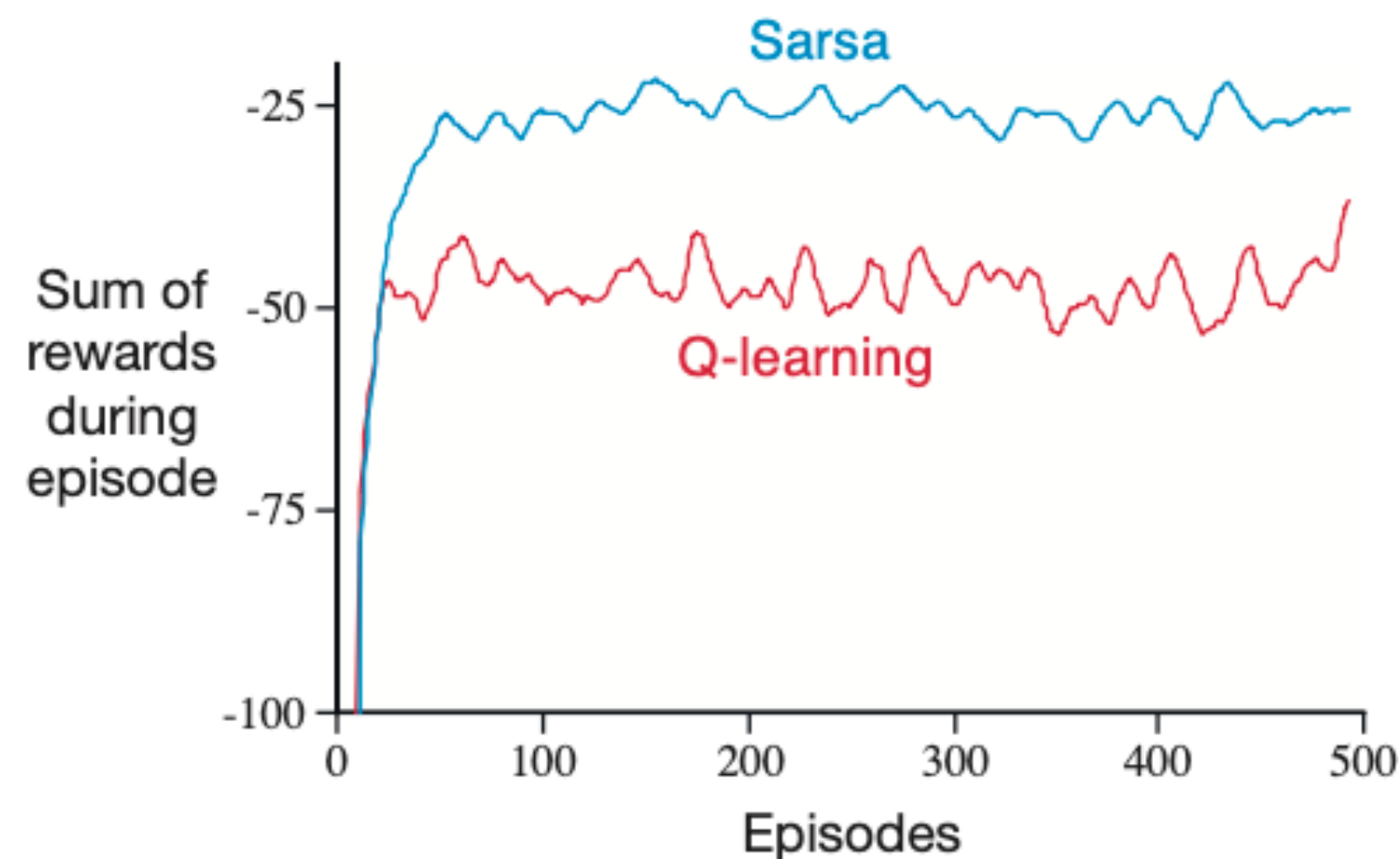
Figure courtesy of Sutton and Barto (2018) pg. 132.
