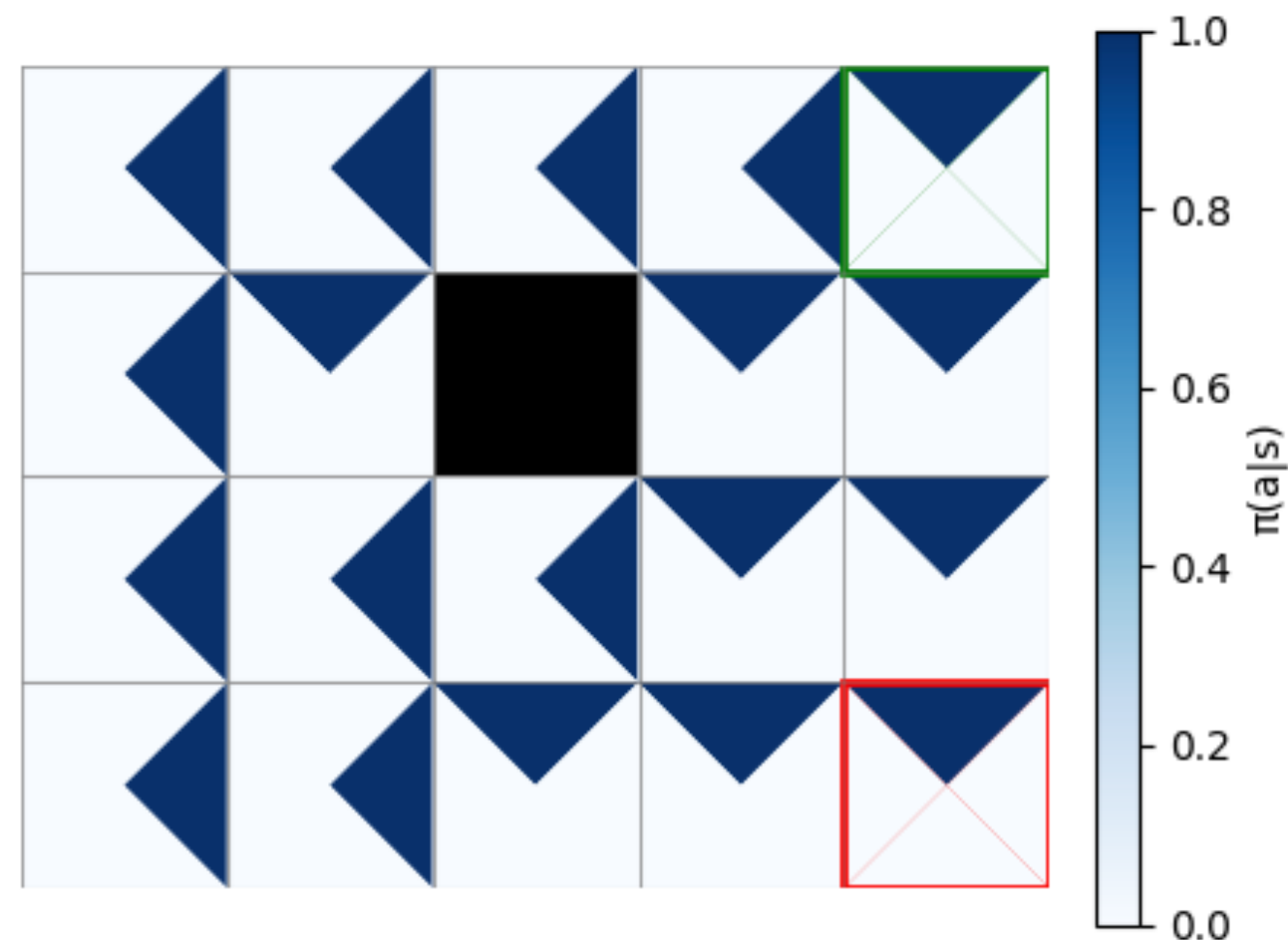
Optimal policy \pi^* , calculated with DP
