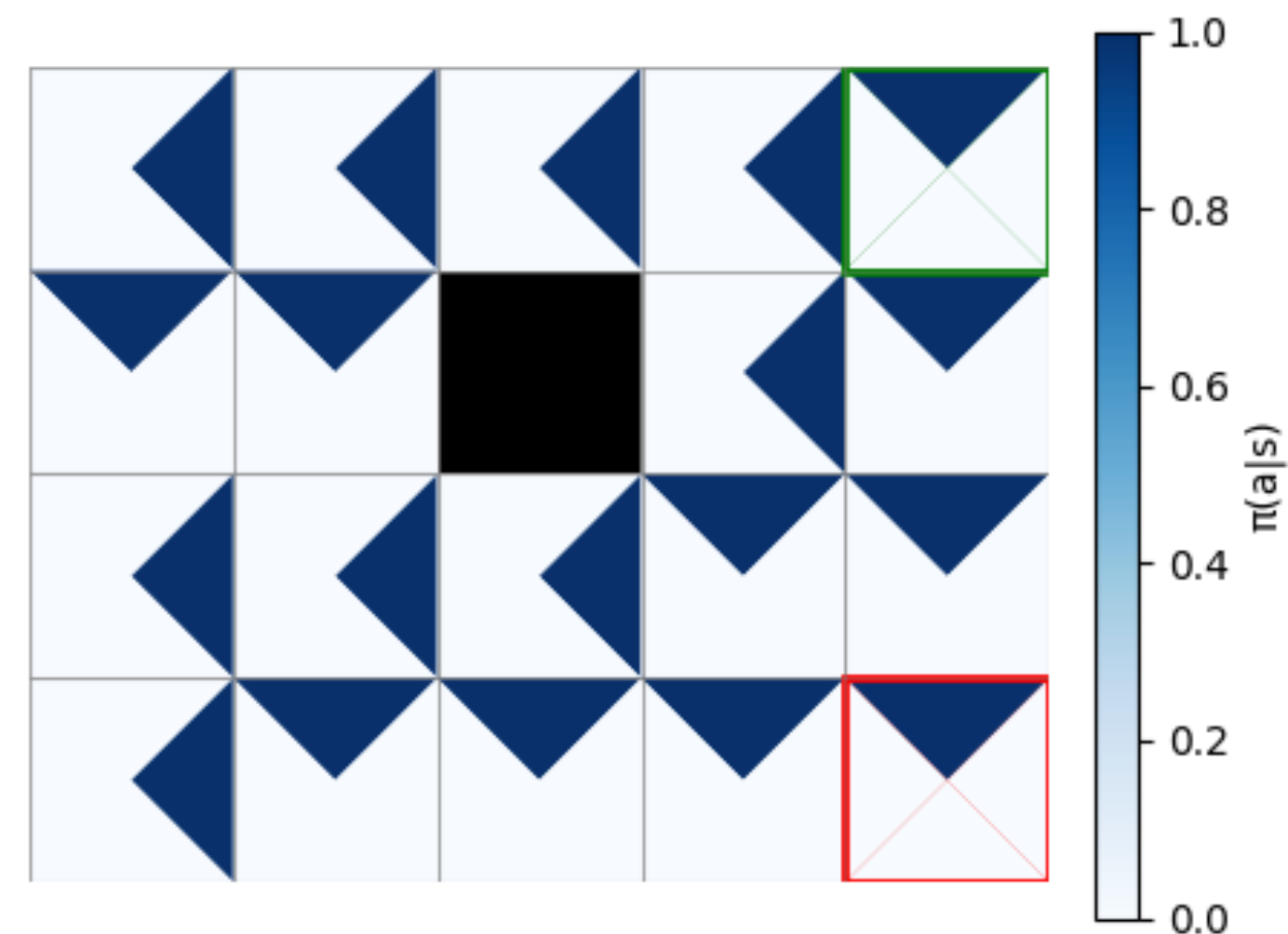
Optimal policy \pi^* , calculated with Q-Learning
