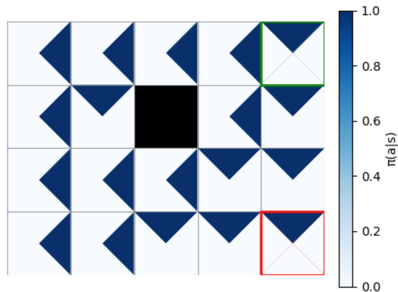
Optimal policy \pi^* , calculated with SARSA
