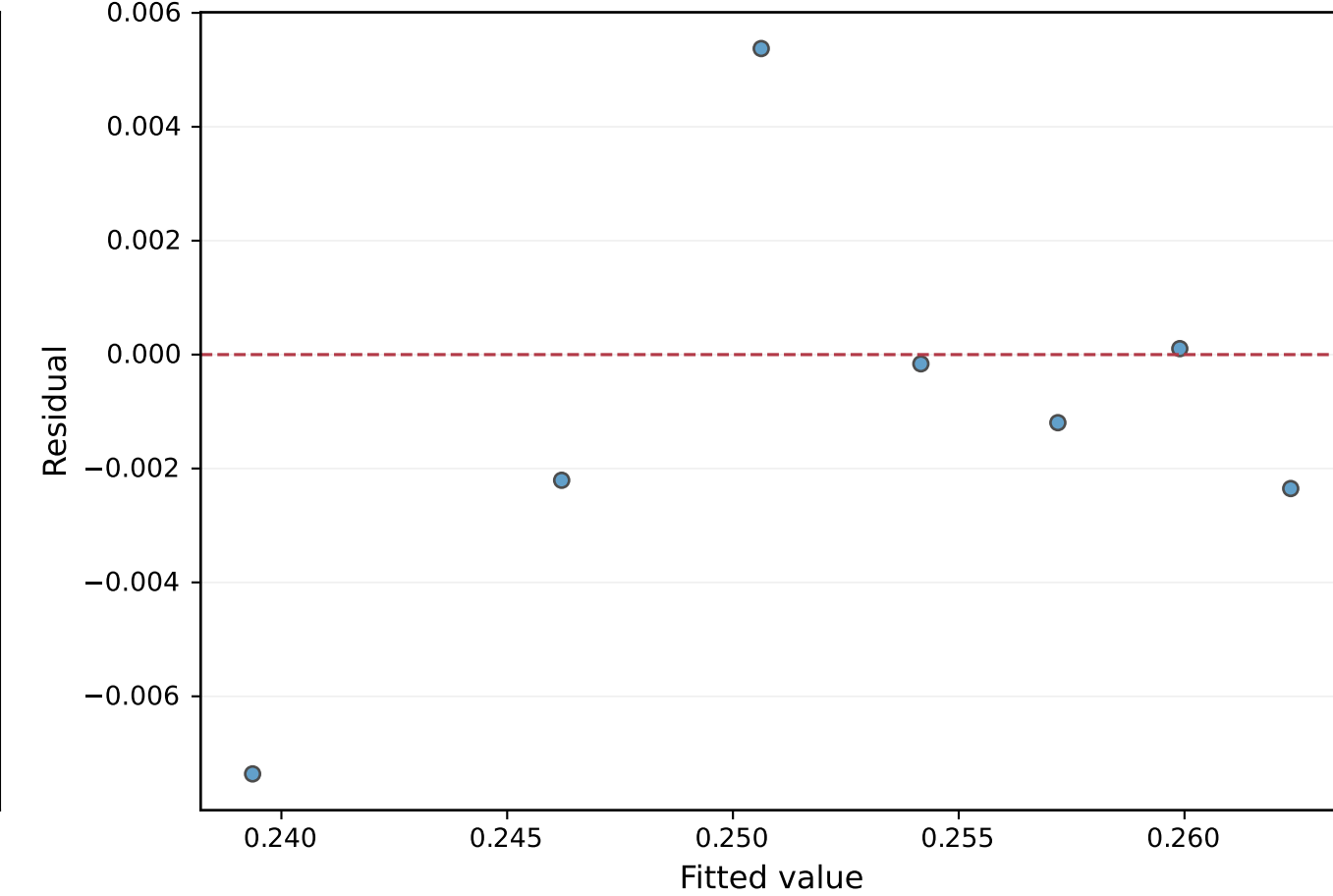
Residuals: Contact Duration - Power-Law
