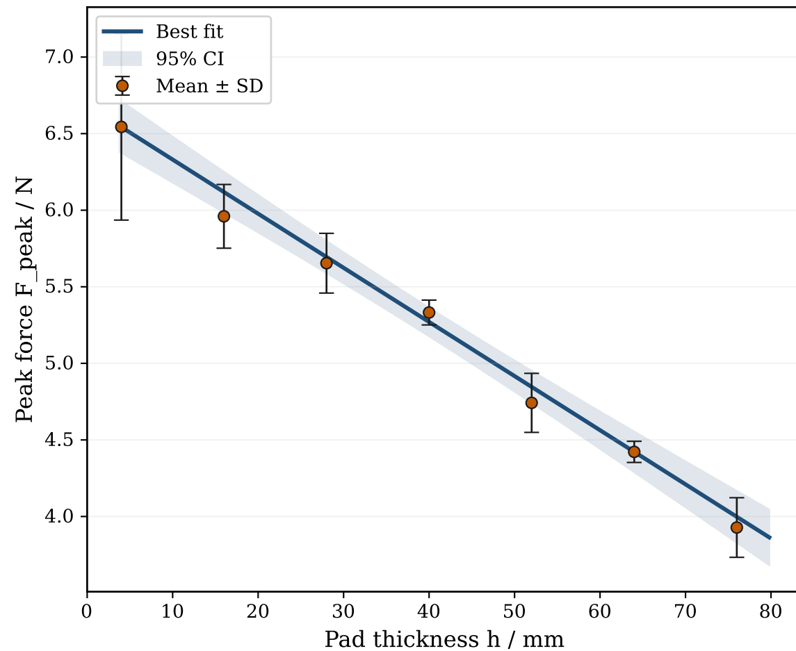
Peak force vs thickness
