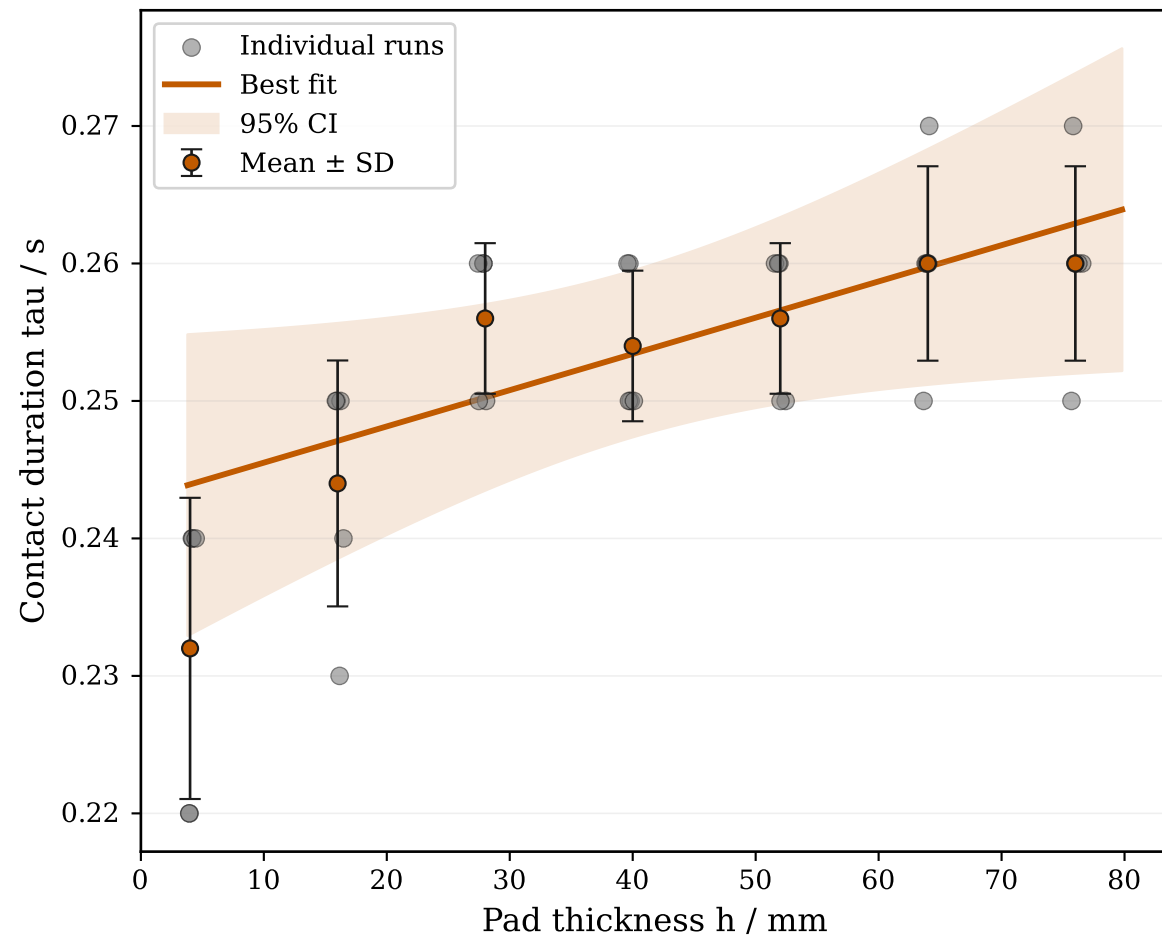
Contact duration vs thickness
