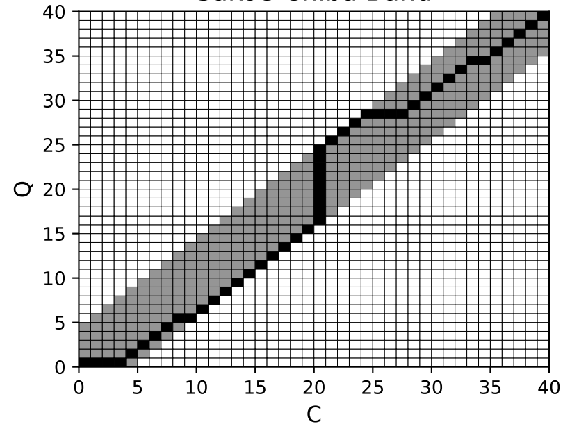
Sakoe-Chiba Band
