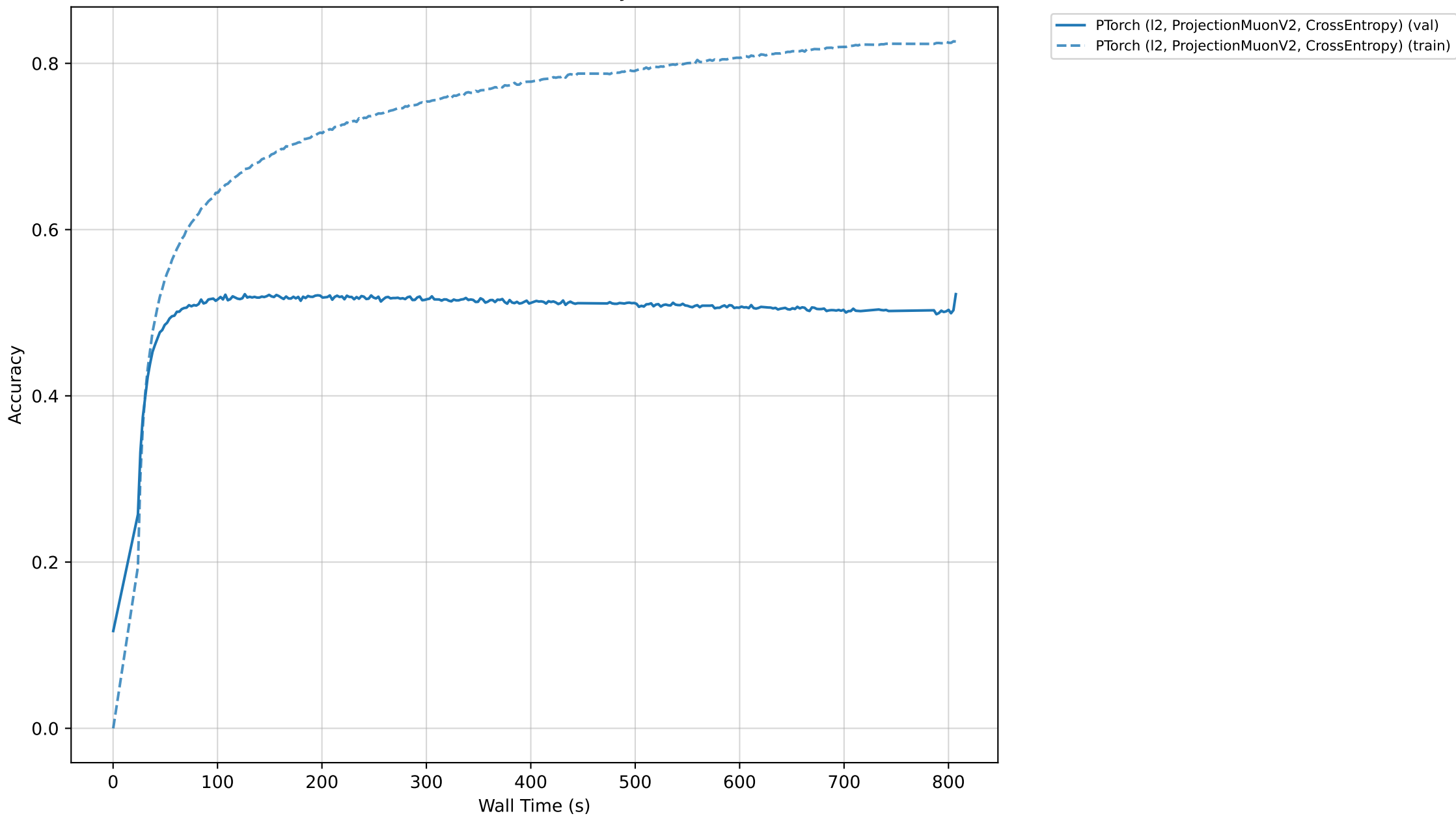
Attention Benchmark: Accuracy vs Wall Time
