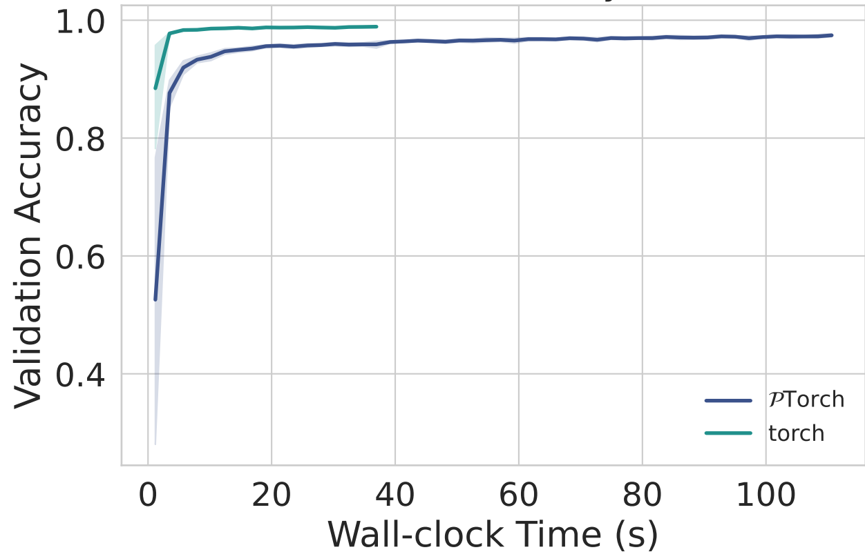
MNIST CNN — Accuracy vs. Time
