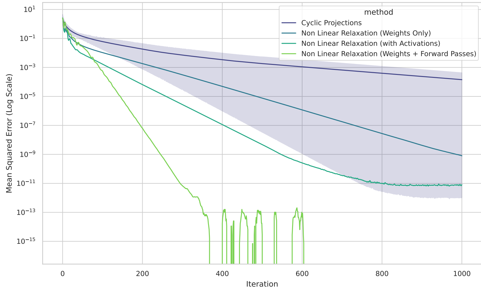
XOR Classification Convergence Analysis
