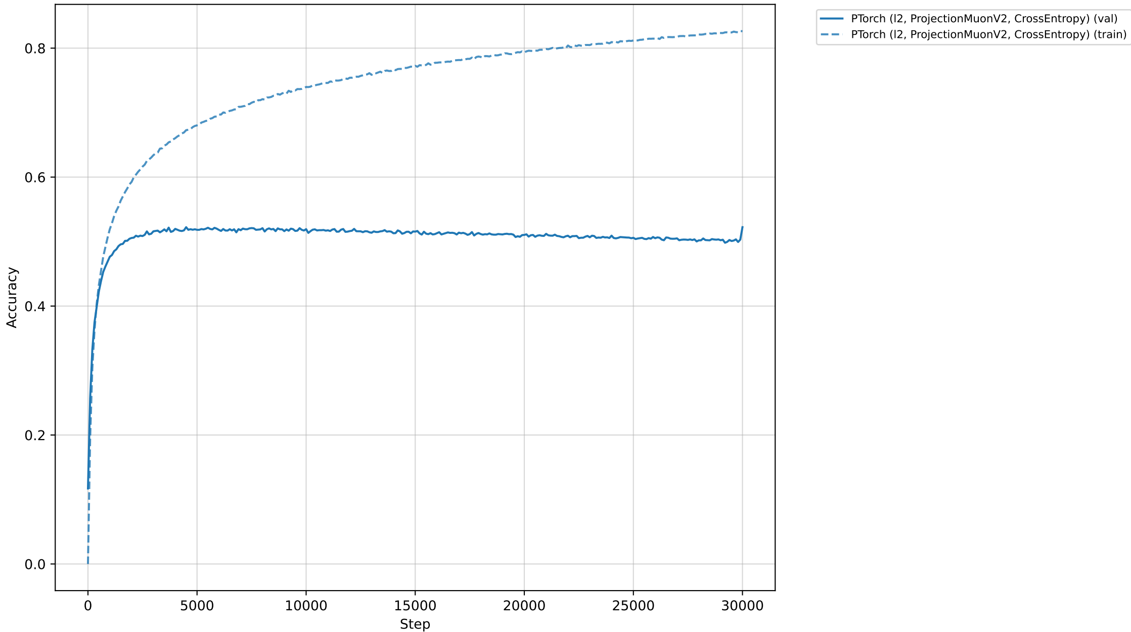
Attention Benchmark: Train vs Validation Accuracy
