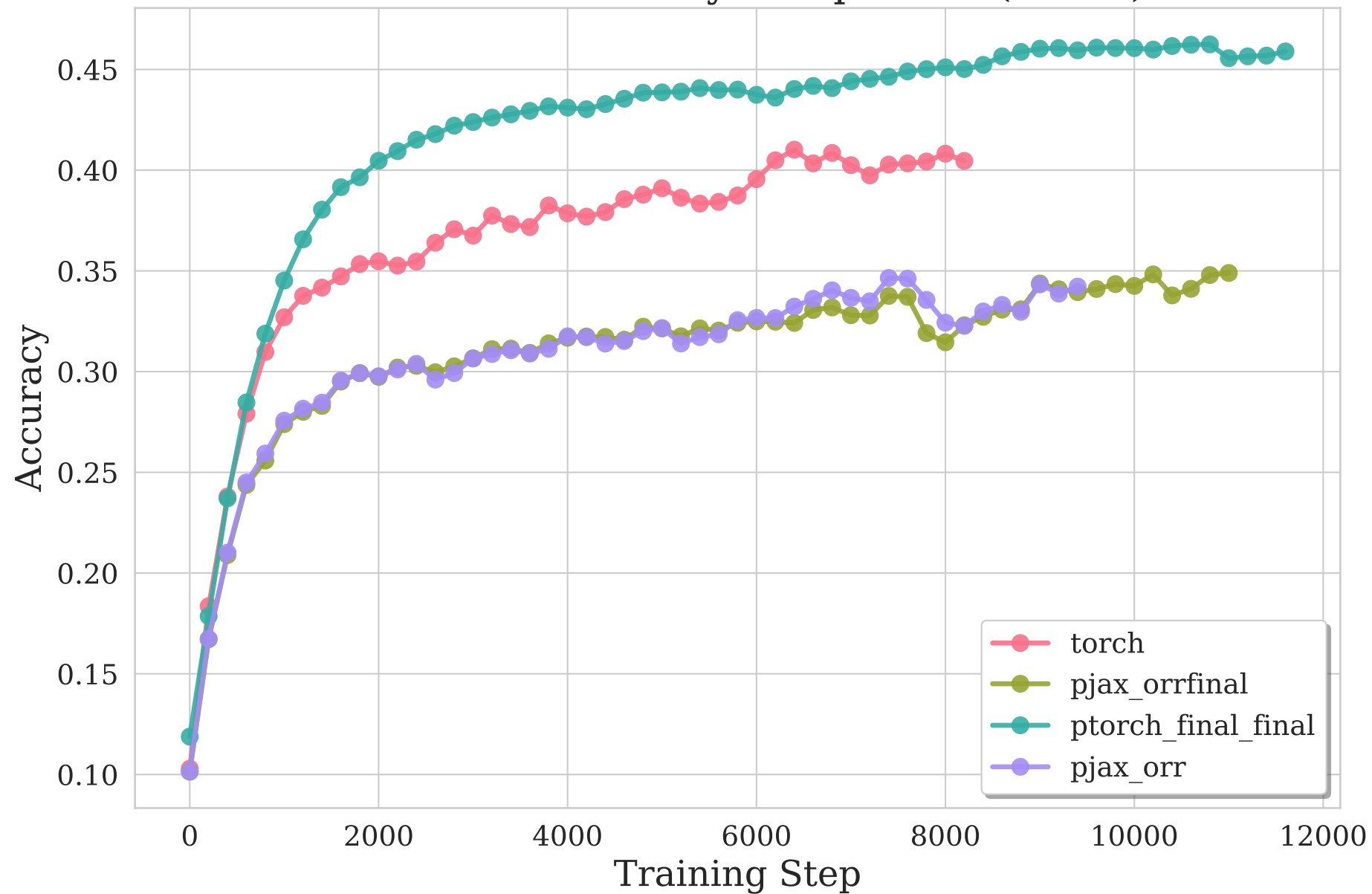
Validation Accuracy Comparison (Run 2)
