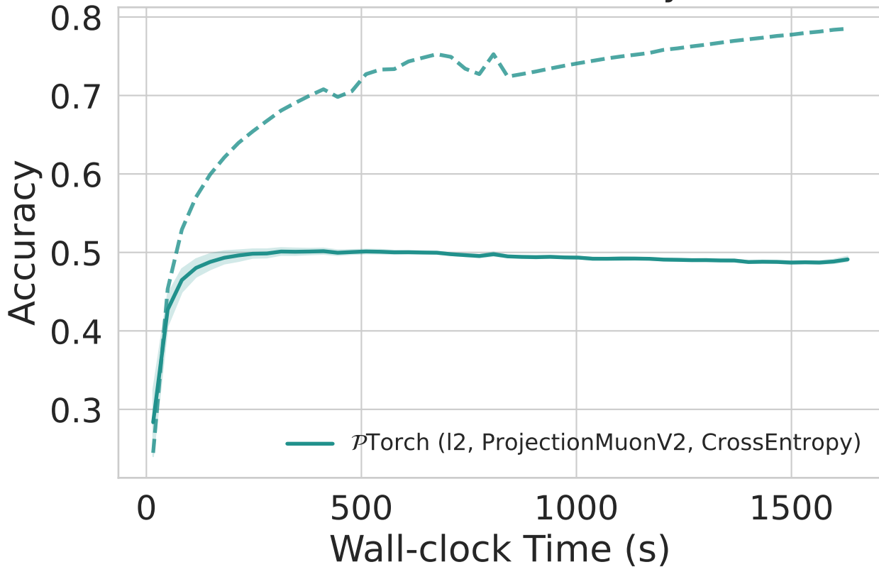
\mathcal{P} Torch Attention — Accuracy vs. Time
