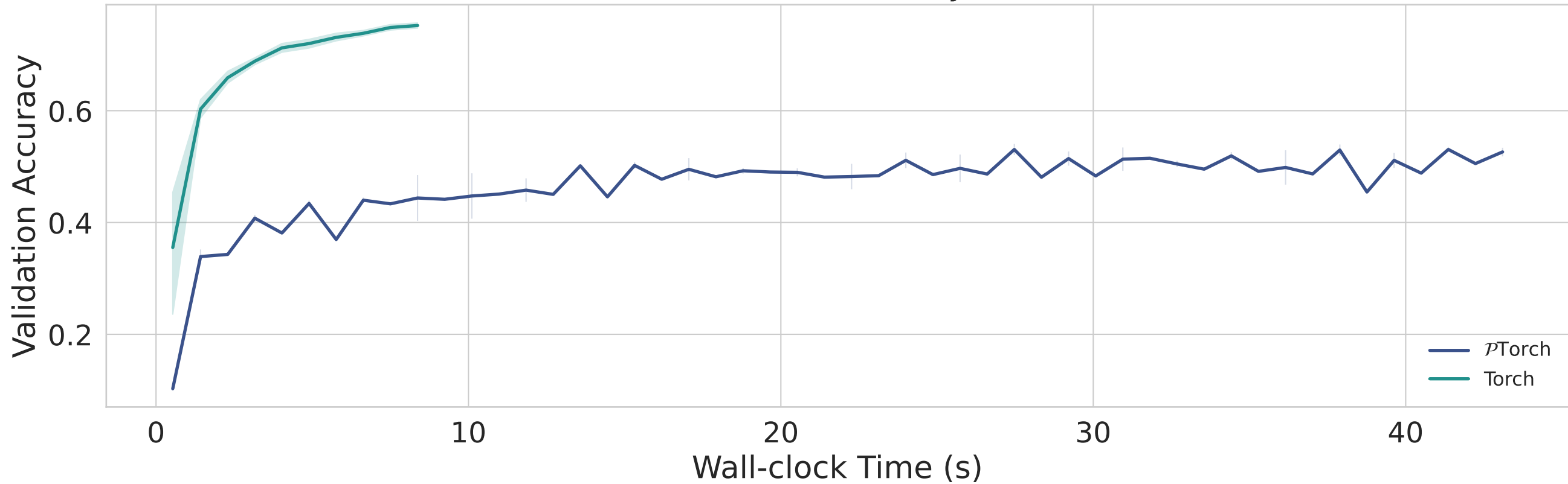
CIFAR10 CNN — Accuracy vs. Time
