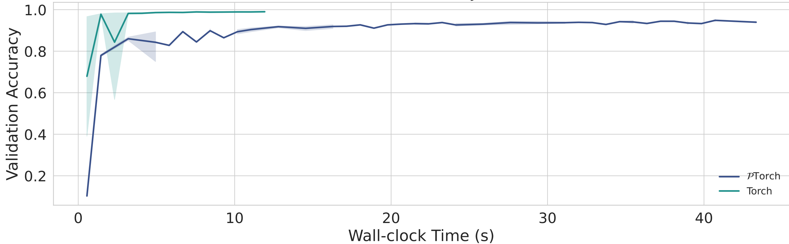
MNIST CNN — Accuracy vs. Time
