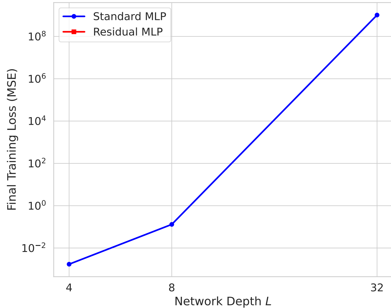
(b) Final Loss vs. Depth L
