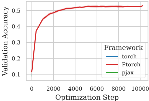
CIFAR10 (Depth: 1L) [BS: unknown]
