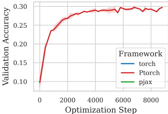
CIFAR10 (Depth: 4L) [BS: unknown]
