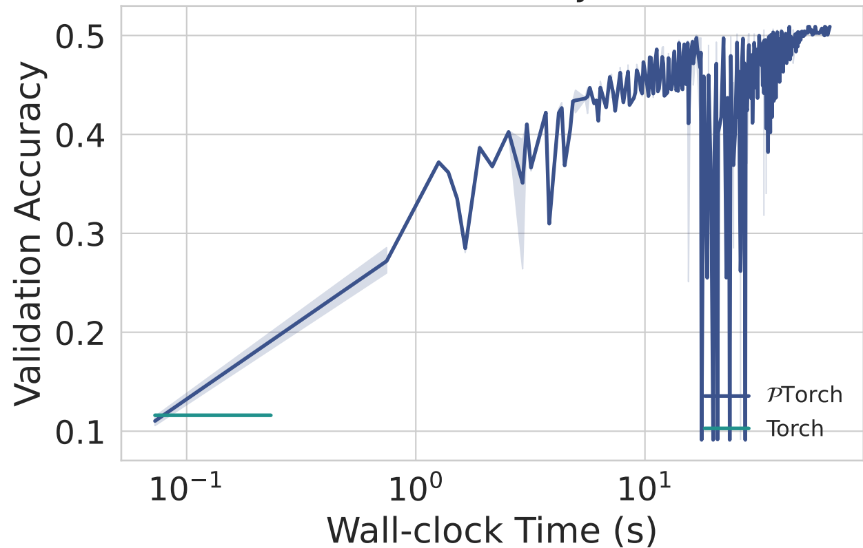
CIFAR10 — Accuracy vs. Time
