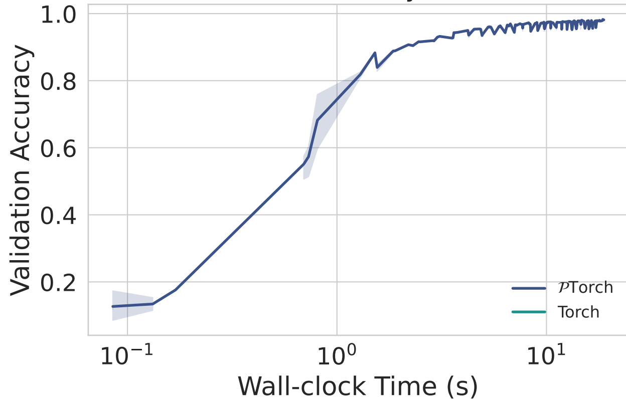
MNIST — Accuracy vs. Time
