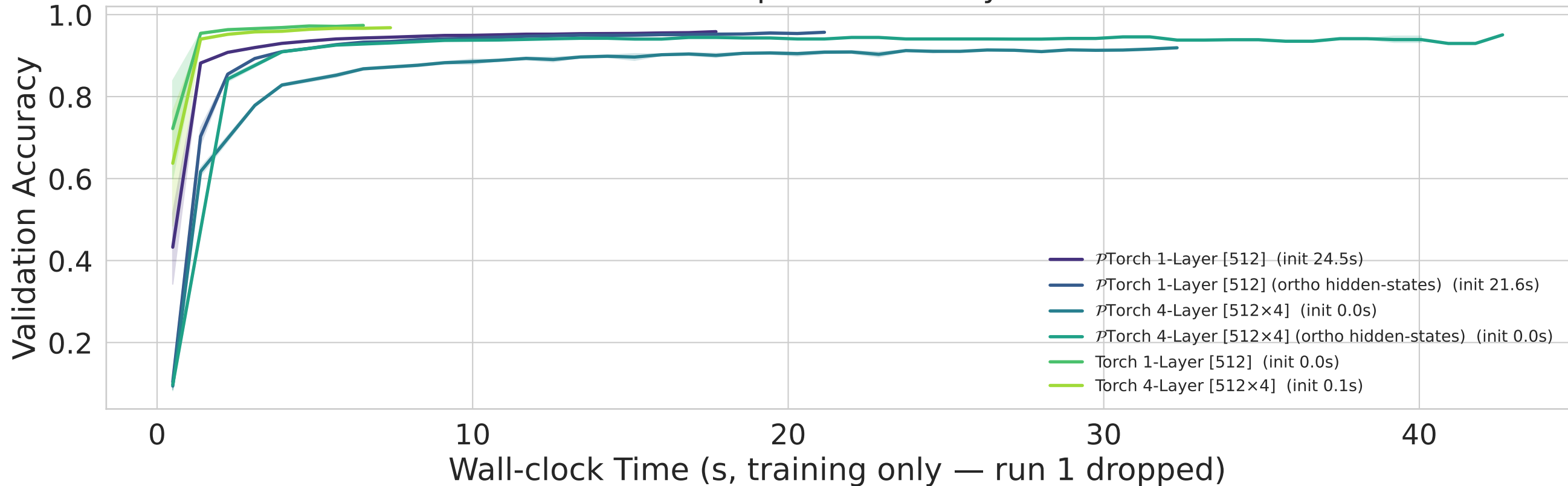
MNIST MLP Depth — Accuracy vs. Time
