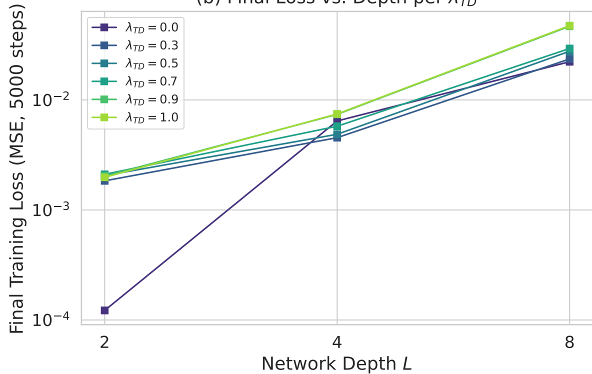
(b) Final Loss vs. Depth per \lambda_{TD}
