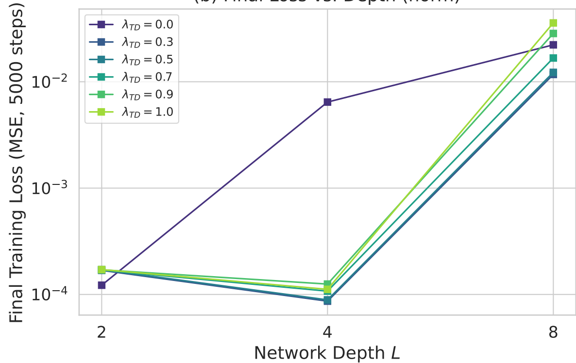
(b) Final Loss vs. Depth (norm)
