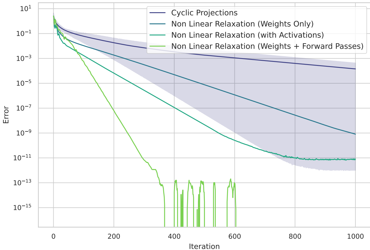
XOR Classification Convergence Analysis
