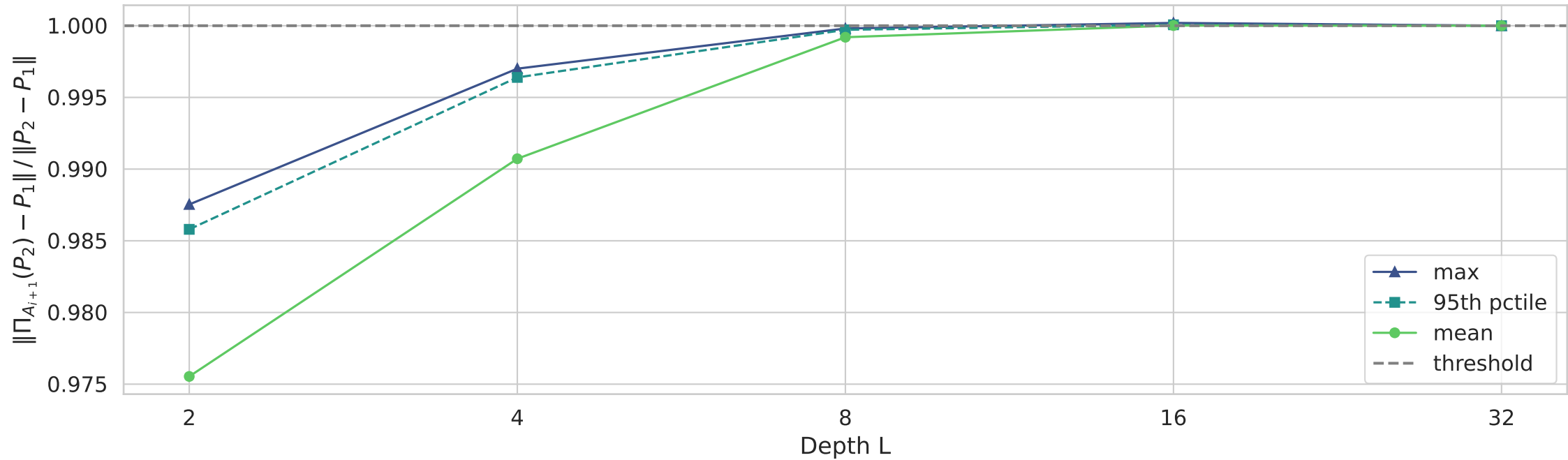
Non-Expansiveness vs Network Depth
