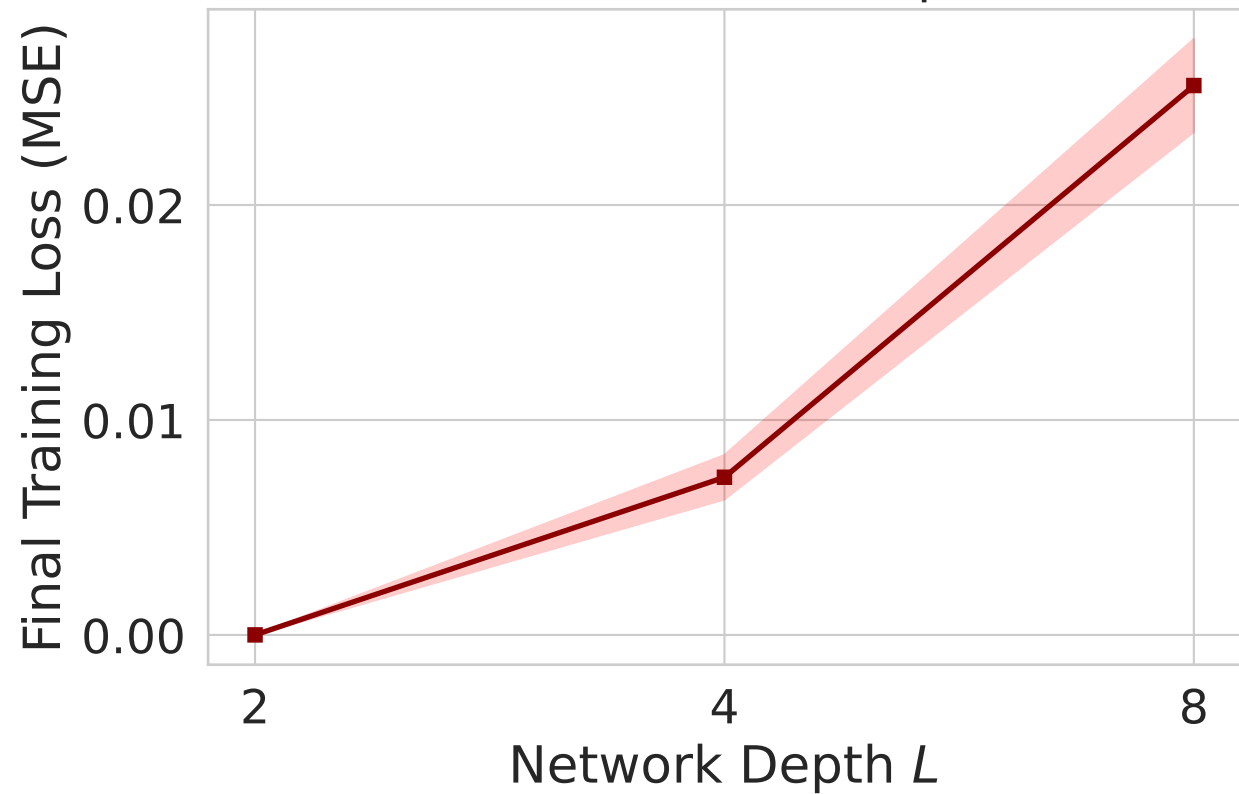
(b) Final Loss vs. Depth L
