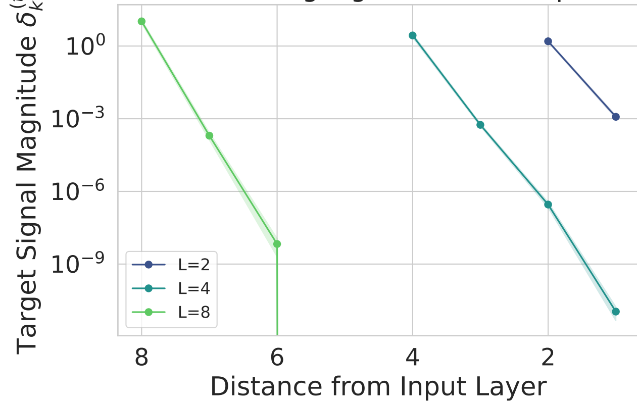
(a) Vanishing Signal Profile (Step 1)
