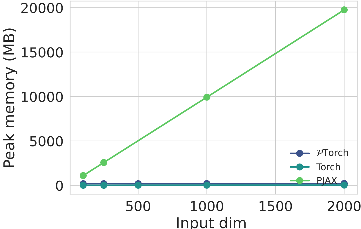
Peak memory vs input neurons (output dim=500, batch size=256)
