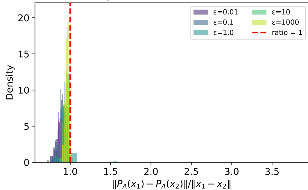
Lipschitz Ratio Distribution
