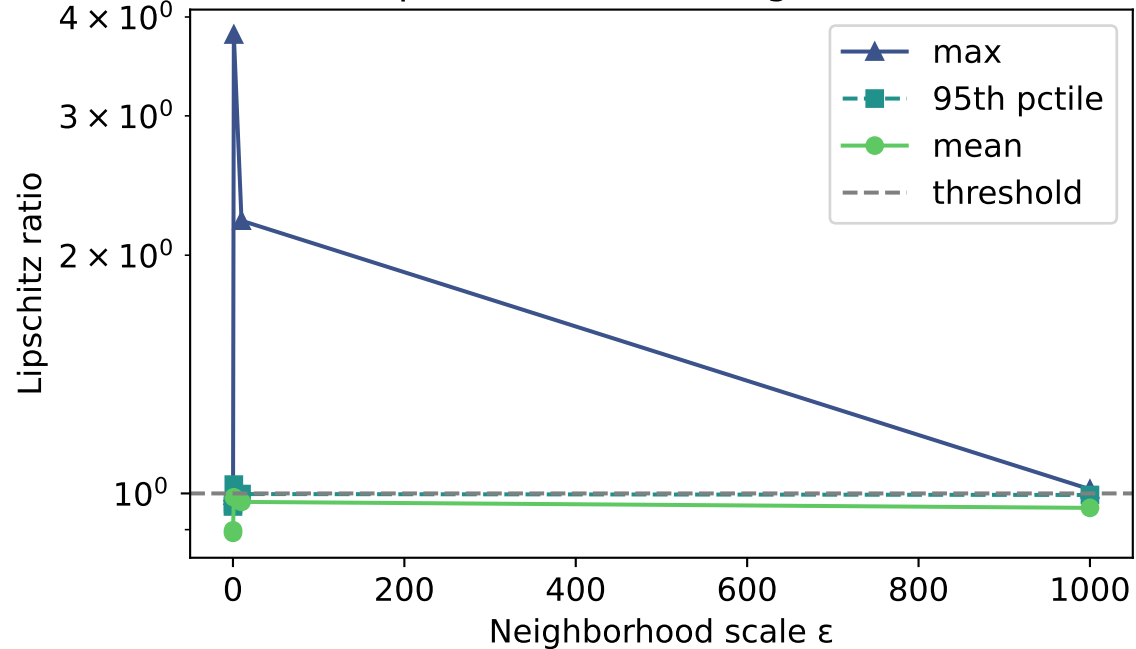
Non-Expansiveness vs Neighborhood Size
