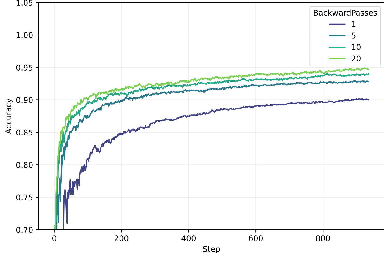
Validation Accuracy by Backward Passes
