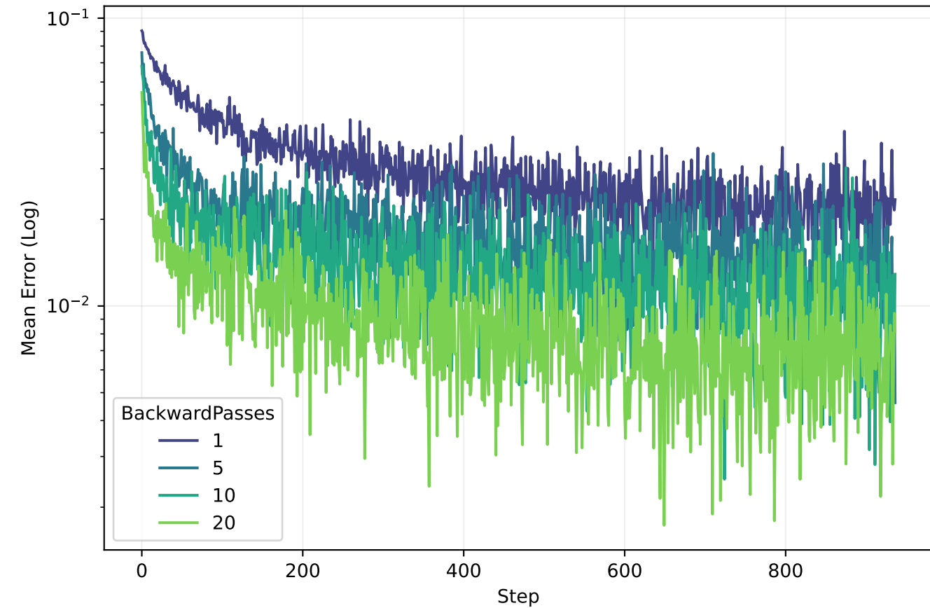
Error Convergence by Backward Passes
