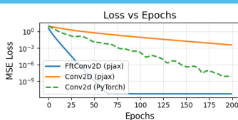
Figure: performance on Synthetic benchmark
