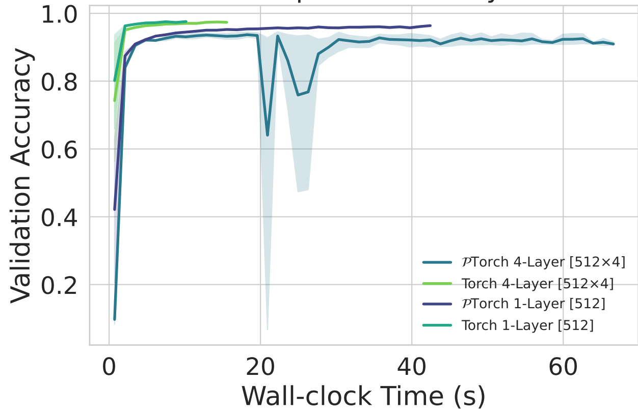
MNIST MLP Depth — Accuracy vs. Time
