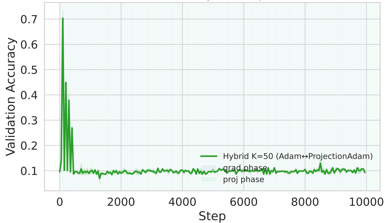
Accuracy vs. Step
