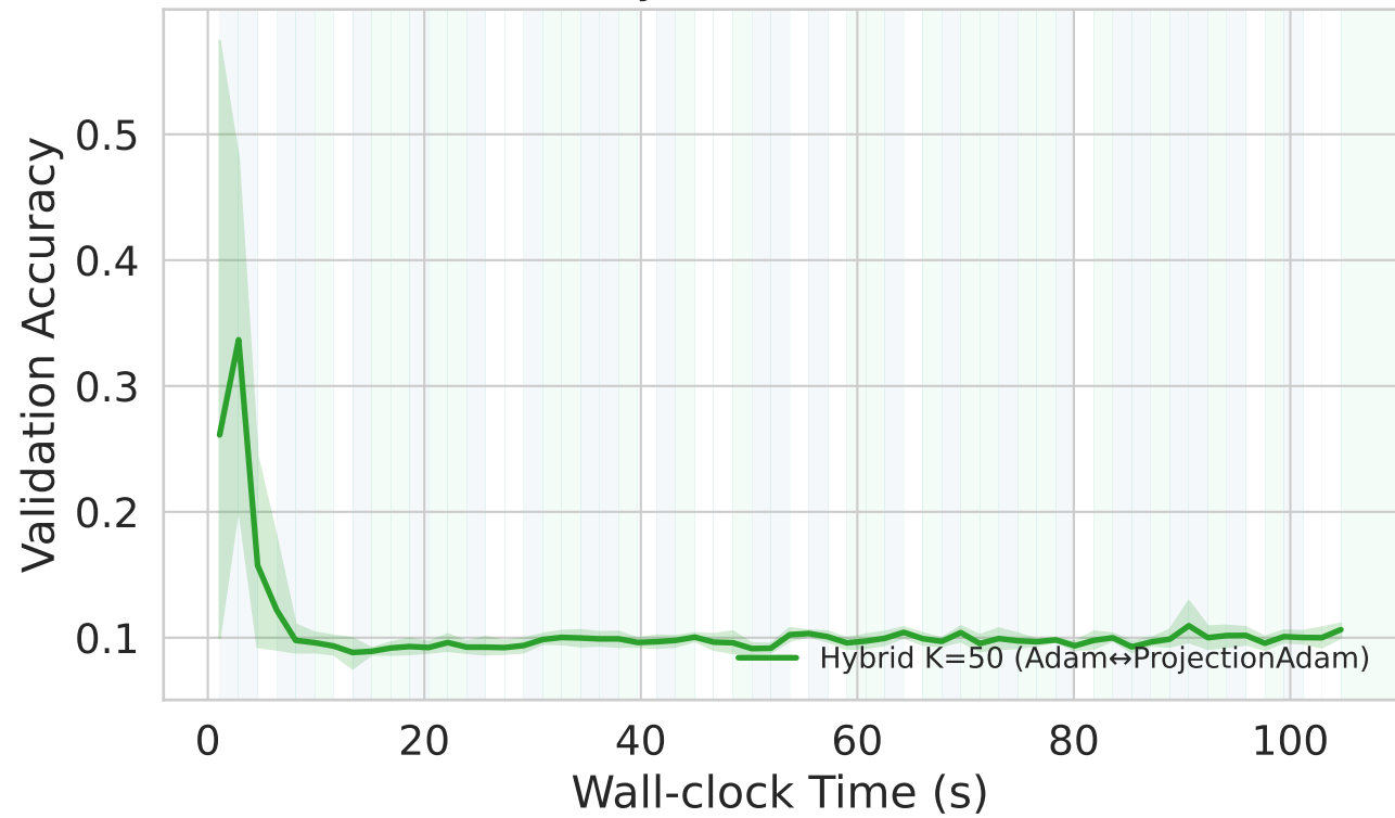
Accuracy vs. Wall-clock Time
