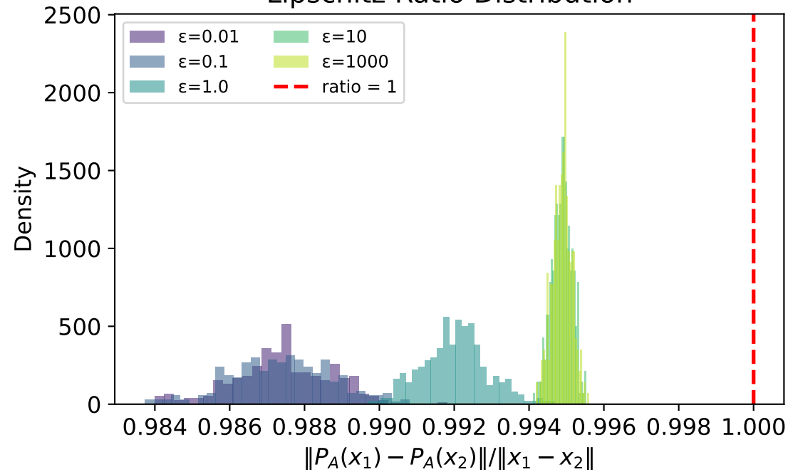
Lipschitz Ratio Distribution
