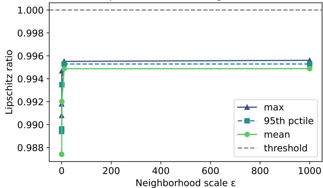
Non-Expansiveness vs Neighborhood Size
