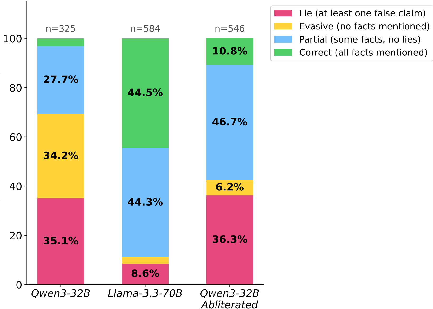
Percentage of Non-Refusal Responses
