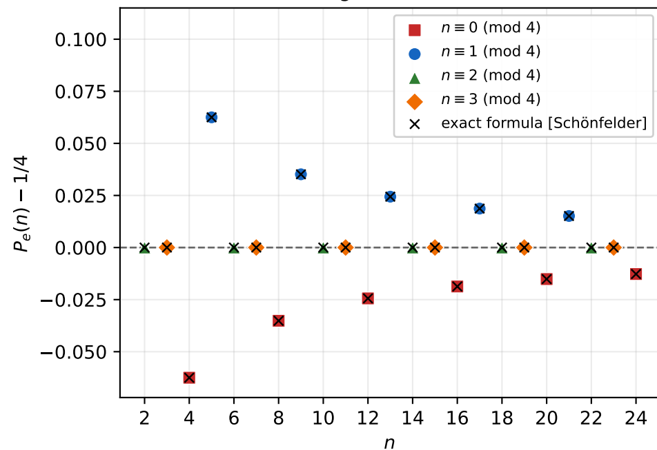
(c) Central edge: the mod-4 structure
