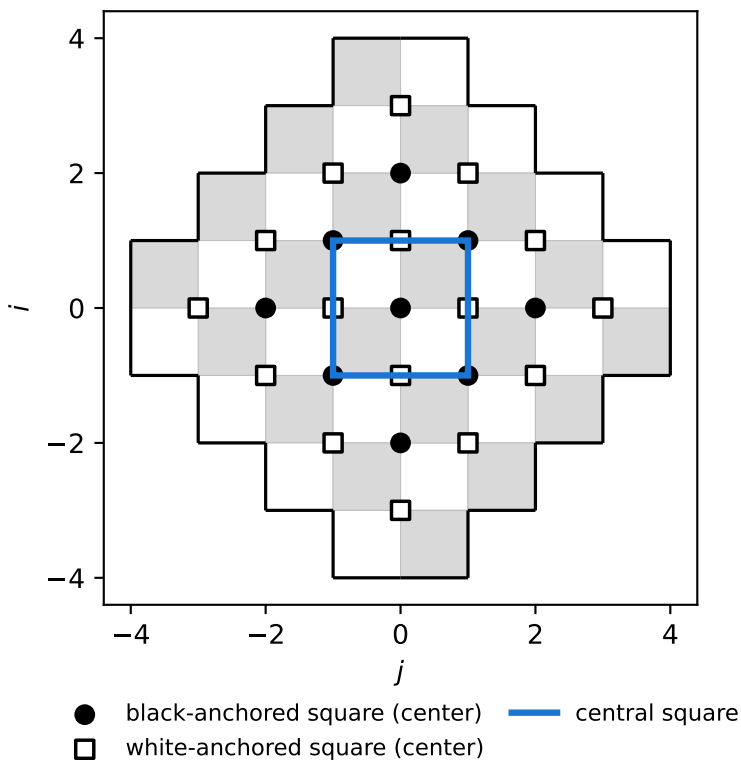
(a) Two sublattices of 2 \times 2 squares, AZ(4)
