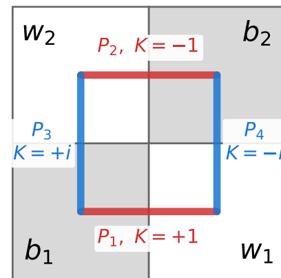
(b) Notation for a black-anchored square
