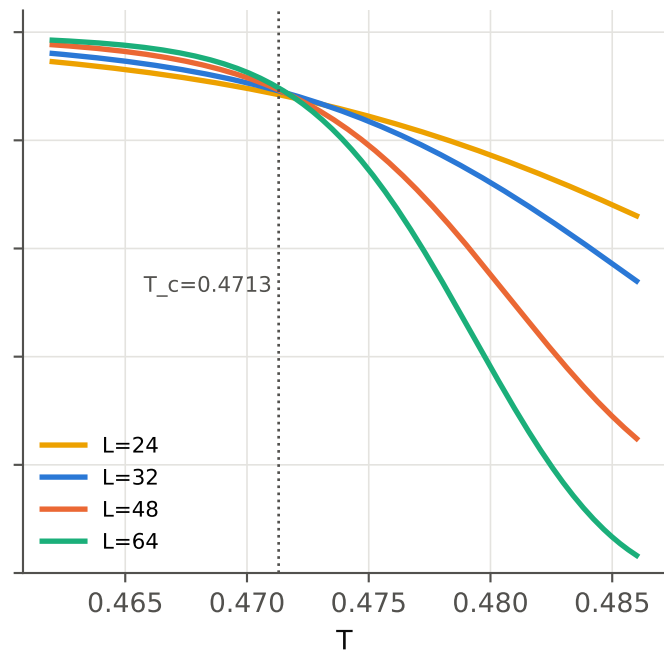
fixed-bond TAFM ( h/J=1 )
