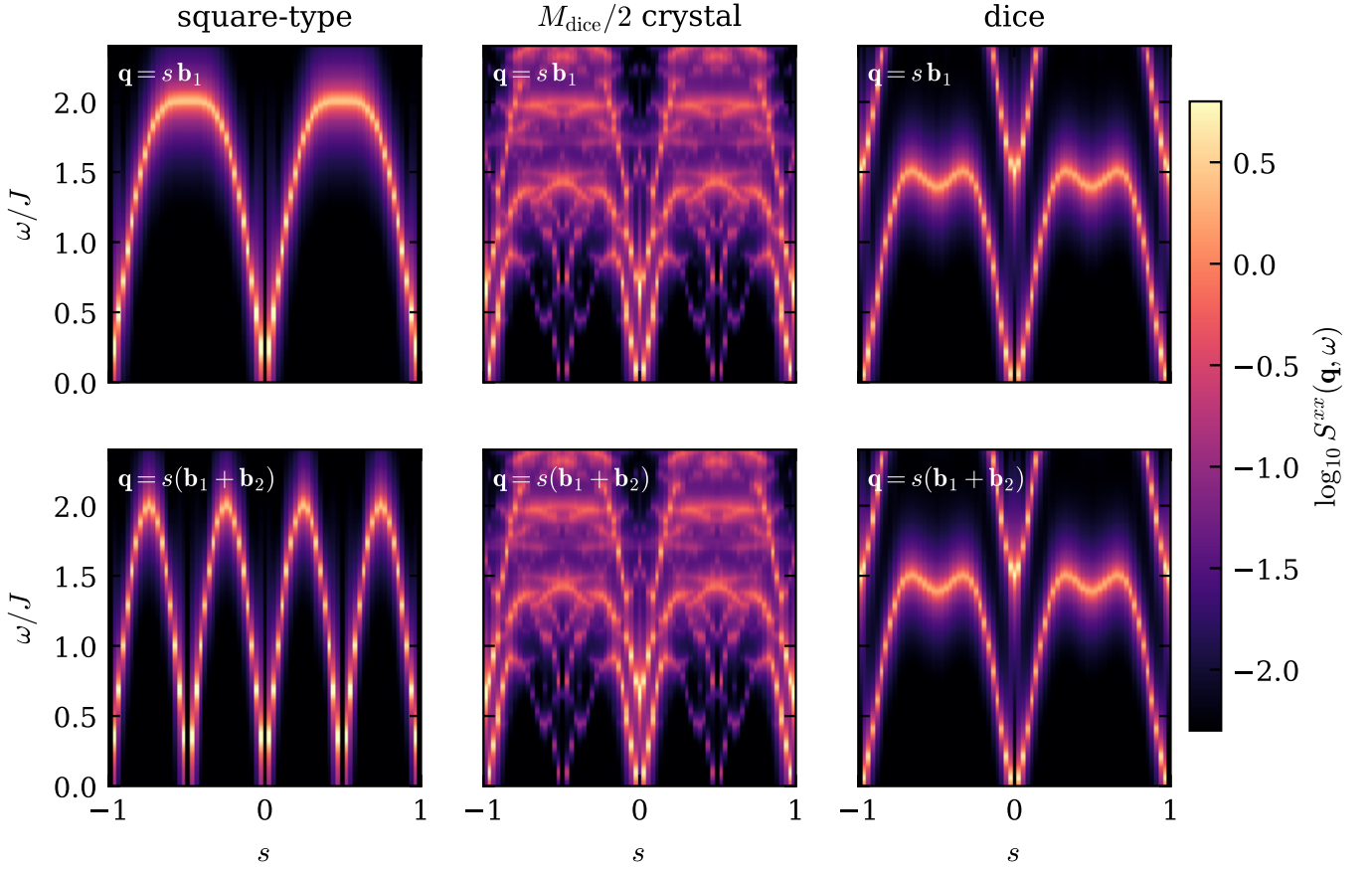
FIG. 7. LSWT transverse dynamical structure factor \log_{10} S^{xx}(\mathbf{q}, \omega) ( S = \frac{1}{2} , L = 36 , Lorentzian broadening 0.03J ) along \mathbf{q} = s \mathbf{b}_1 (top) and \mathbf{q} = s(\mathbf{b}_1 + \mathbf{b}_2) (bottom), where \mathbf{b}_{1,2} are the reciprocal vectors of the triangular lattice. Left: square-type tiling (a single sharp magnon branch). Center: M_{\text{dice}}/2 crystal (backfolded minibands and gaps set by the 6 \times 4 cell). Right: dice (a Goldstone branch plus the dispersionless band near 1.5J that comes from the rim sites).
