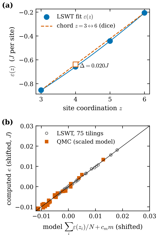
FIG. 2. Coordination mechanism of quantum tiling selection ( S = \frac{1}{2} ). (a) Single-site zero-point energies \varepsilon(z) obtained by fitting LSWT energies of 75 tilings to Eq. (2). \varepsilon(z) is convex, so at fixed \langle z \rangle = 4 the uniform z = 4 tiling lies below the dice combination (open square) by \Delta = 0.020J per site. (b) Energies computed for many tilings vs the coordination model: LSWT (open circles, rms residual 1.4 \times 10^{-4}J ) and QMC with the model rescaled linearly (squares, rms 5 \times 10^{-4} - 8 \times 10^{-4}J ). Both axes are shifted by a common constant.
