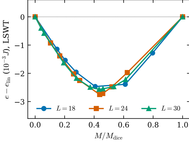
FIG. 11. LSWT energies of annealed tilings relative to the square-to-dice line for L = 18, 24, 30 . The lower envelope is size-independent to within 3 \times 10^{-4} J .
