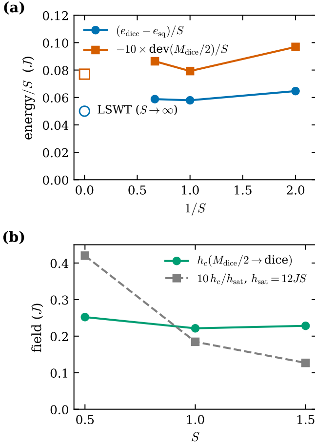
FIG. 8. Spin- S QMC ( L = 12 , \beta JS = 12 ). (a) Selection energies per unit S : dice minus square-type (circles) and the M_{\text{dice}}/2 deviation (squares, \times 10 ). Open symbols: LSWT ( S \rightarrow \infty ). Both approach finite limits, i.e., selection energies scale as JS . (b) The field at which the M_{\text{dice}}/2 crystal gives way to dice at this system size (circles) is S -independent in units of J . Relative to the saturation scale, the intermediate region therefore shrinks as 1/S (squares).
