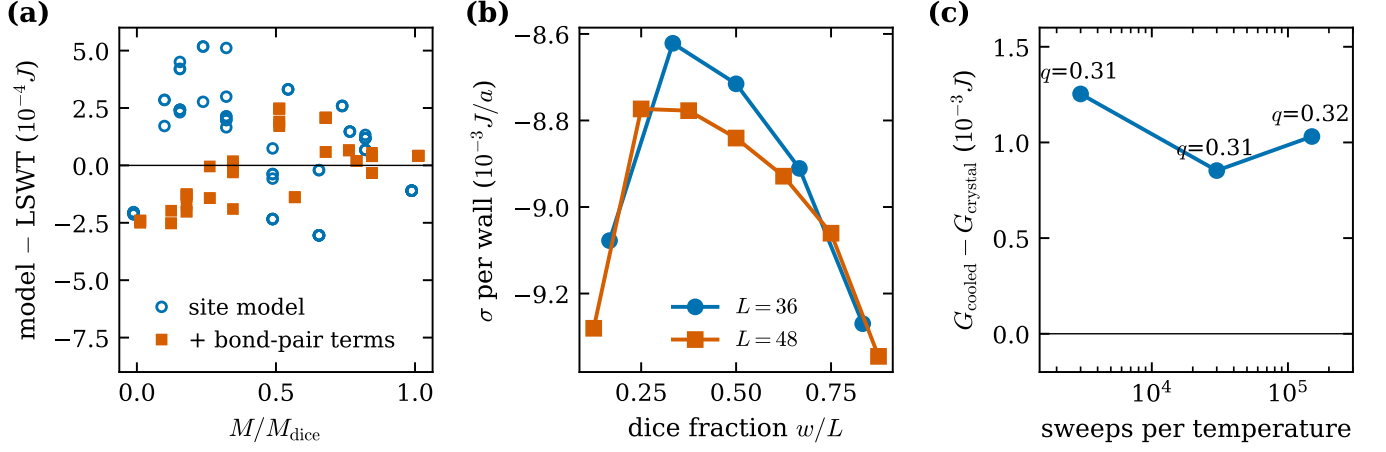
FIG. 12. (a) Out-of-sample test of Eq. (2) on 71 periodic crystals, relative to thermodynamic-limit LSWT: site model (circles) and site model with bond-pair terms (squares). Points are offset horizontally for clarity. (b) LSWT energy per straight dice|square wall for a dice strip of width w in a square background on L = 36 and 48 tori. The walls are w and L - w rows apart, and closely spaced walls ( w/L near 0 or 1) have lower energy. (c) Free energy G = e_0 - hm of the state reached by cooling to T = 0.005J relative to the M_{\text{dice}}/2 crystal, for three cooling rates; labels give the overlap q with the crystal.
