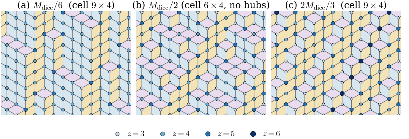
FIG. 4. Periodic tilings on the lower convex hull of e_0(m) (QMC, S = \frac{1}{2} ). (a) M_{\text{dice}}/6 crystal (cell 9 \times 4 , shear s = 5 ): sparse z = 3, 5 pairs in a square-type background. (b) M_{\text{dice}}/2 crystal (cell 6 \times 4 , s = 4 ): z = 3, 4, 5 in equal numbers and no sixfold hubs. (c) 2M_{\text{dice}}/3 crystal (cell 9 \times 4 , s = 7 ): the first appearance of hubs, z_3:z_4:z_5:z_6 = 16:6:12:2 . Color code as in Fig. 1.
