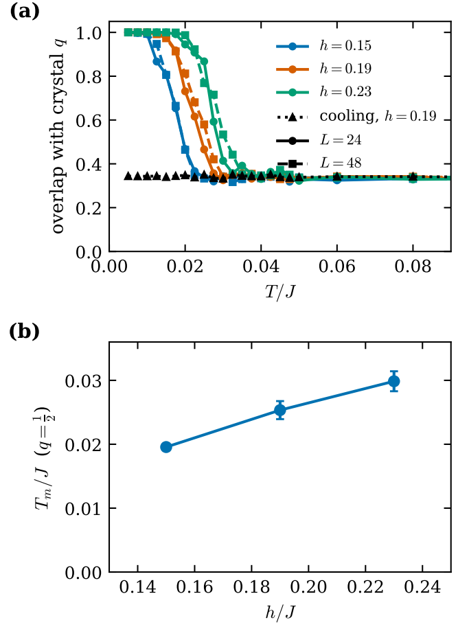
FIG. 9. Thermal stability of the M_{\text{dice}}/2 crystal (tiling Monte Carlo with the QMC-scaled coordination model, local hexagon flips, crystal tilt sector). (a) Overlap q of the tiling with the crystal on heating for three fields and two sizes, and on slow cooling from the disordered state (triangles). q \simeq \frac{1}{3} is the value for an uncorrelated tiling. (b) Melting temperature, defined by q = \frac{1}{2} .
