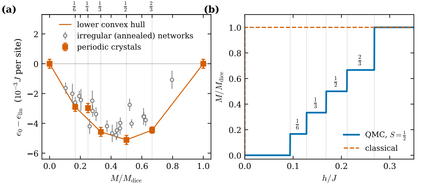
FIG. 5. Magnetization staircase ( S = \frac{1}{2} , QMC). (a) Zero-field energy relative to the straight line between the square-type and dice tilings, e_{\text{lin}}(m) = e_{\text{sq}} + 6m(e_{\text{dice}} - e_{\text{sq}}) . Squares: best periodic crystal at each M/M_{\text{dice}} (cells \leq 36 sites; L = 36 for \frac{1}{6}, \frac{1}{3}, \frac{1}{2}, \frac{2}{3} , L = 24 for \frac{1}{4} ). Circles: irregular networks from LSWT annealing at L = 18, 24, 30 . The line is the lower convex hull. (b) T = 0 magnetization obtained by minimizing e_0 - hm over the hull (solid), compared with the classical jump (dashed). Dotted vertical lines mark the step fields listed in Table I.
