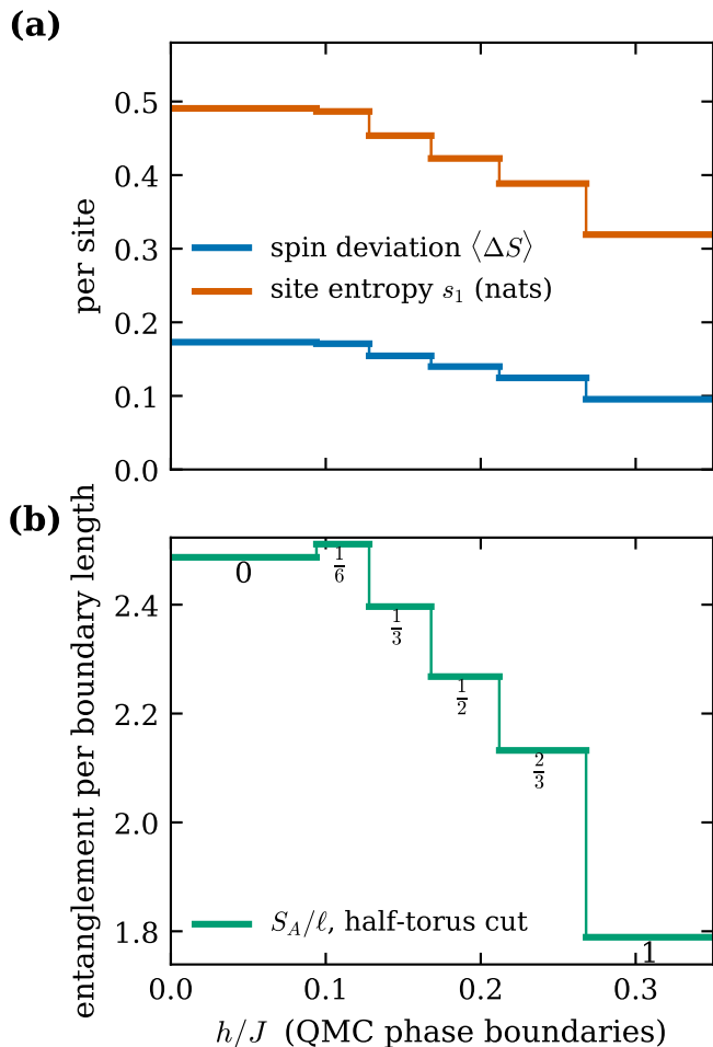
FIG. 6. Quantum-fluctuation measures of the LSWT ground state ( S = \frac{1}{2} , L = 36 ) of the crystal selected at each field, using the QMC phase boundaries. (a) Mean spin deviation \langle \Delta S \rangle = \langle a^\dagger a \rangle and single-site entanglement entropy. (b) Gaussian entanglement entropy of half the torus per unit boundary length. Plateau labels give M/M_{\text{dice}} .
