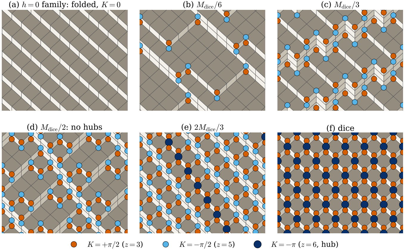
FIG. 10. Tilings lifted to stepped surfaces in \mathbb{Z}^3 (orthographic view, tilted by 12^\circ from [111] ; faces shaded by orientation). Colored dots mark vertices with nonzero discrete Gaussian curvature K_i = 2\pi - \frac{\pi}{2}z_i . (a) A zero-curvature tiling from the degenerate h=0 family: two facets joined by straight folds, K_i=0 everywhere. (b)–(e) The plateau crystals. Positive curvature ( z=3 ) sits only on the majority sublattice and negative curvature ( z=5,6 ) only on the minority sublattice. The M_{\text{dice}}/2 crystal (d) uses only \pm\pi/2 vertices. (f) Dice: +\pi/2 cones and -\pi hubs.
