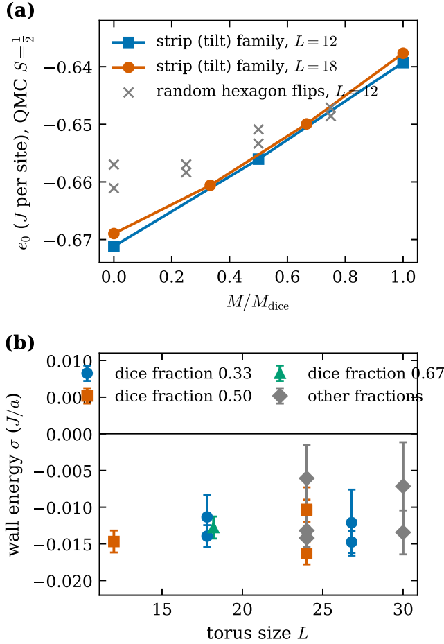
FIG. 3. (a) QMC ground-state energies ( S = \frac{1}{2} ) of the tilt family (parallel strips of dice and square tiling) for L = 12 and 18 , together with tilings obtained from random hexagon flips (crosses). Random flips cost energy at fixed M ; the classical energy is -0.5J for all points. (b) Energy per unit length of a dice|square wall extracted from the strips, for several dice fractions and torus sizes. All values are negative.
