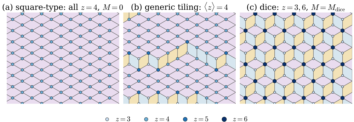
FIG. 1. Lozenge tilings of the triangular lattice and the bipartite networks they define. Rhombi are shaded by orientation, and sites are colored and sized by coordination z . (a) Square-type tiling: all z = 4 , compensated ( M = 0 ). (b) A generic tiling, with z varying from site to site; every tiling has \langle z \rangle = 4 . (c) Dice lattice: sixfold hubs and threefold rims, Lieb moment M_{\text{dice}} = SN/3 . All tilings have the same classical energy -2JS^2N .
