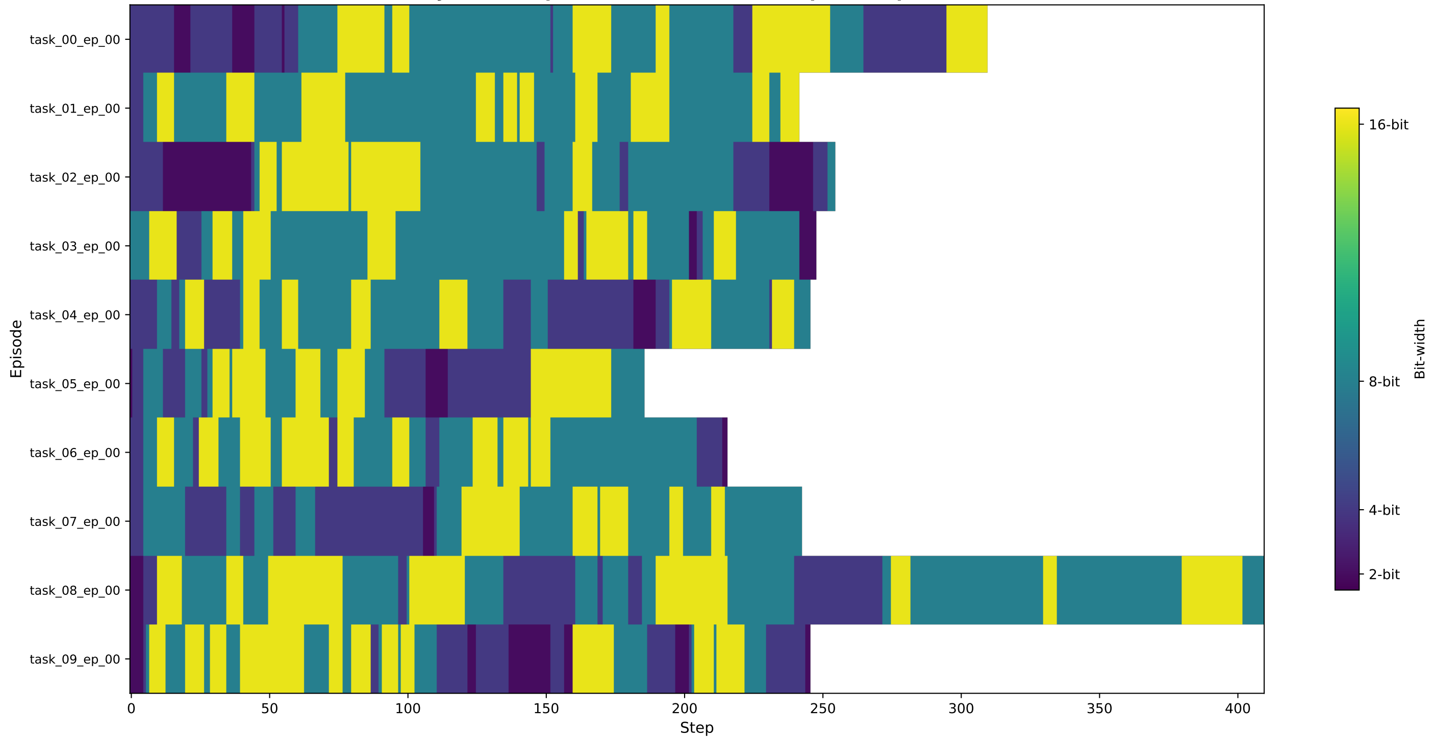
DyQ-VLA Dispatched Bit-Width Heatmap — All Episodes
