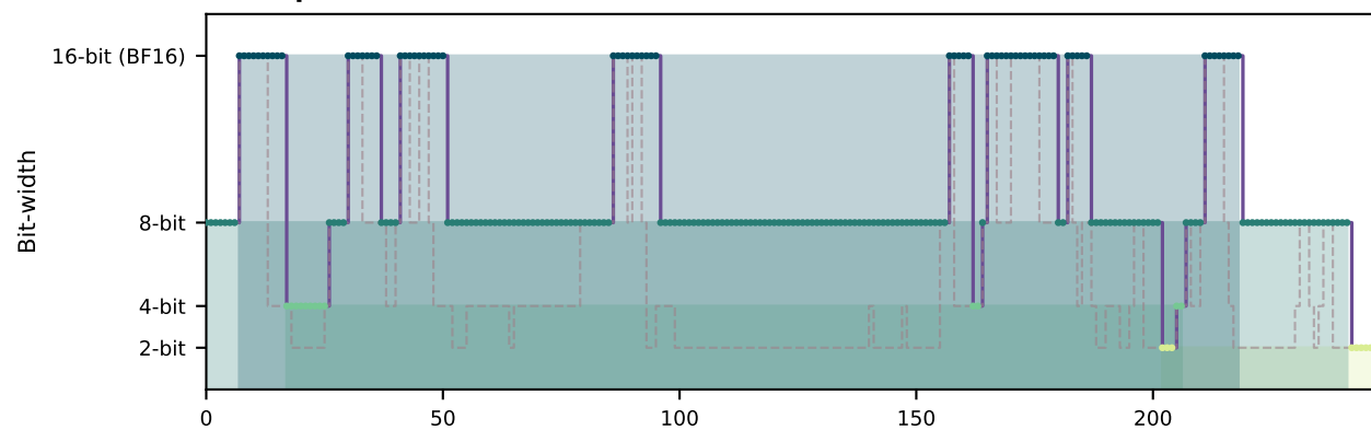
task_03_ep_00 put the black bowl in the bottom drawer of the cabinet and close it
