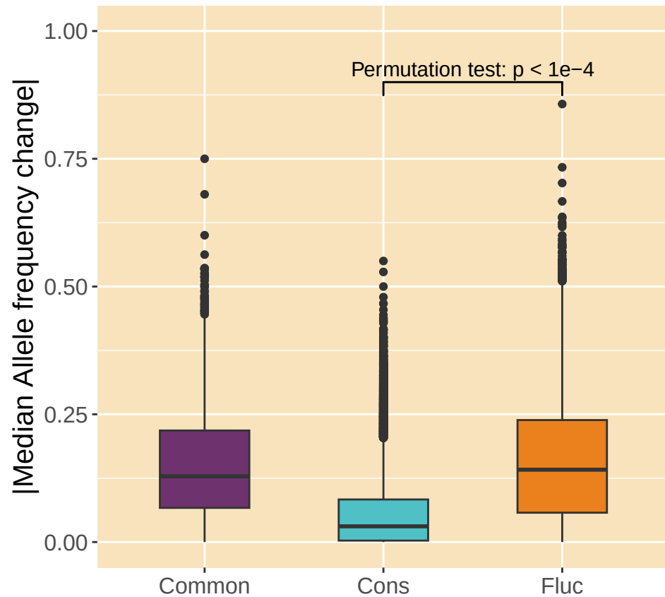
Evolution in 28/18
