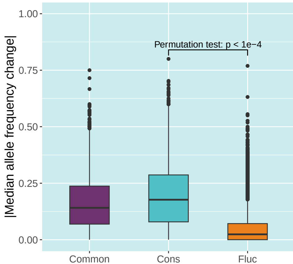
Evolution in 23
