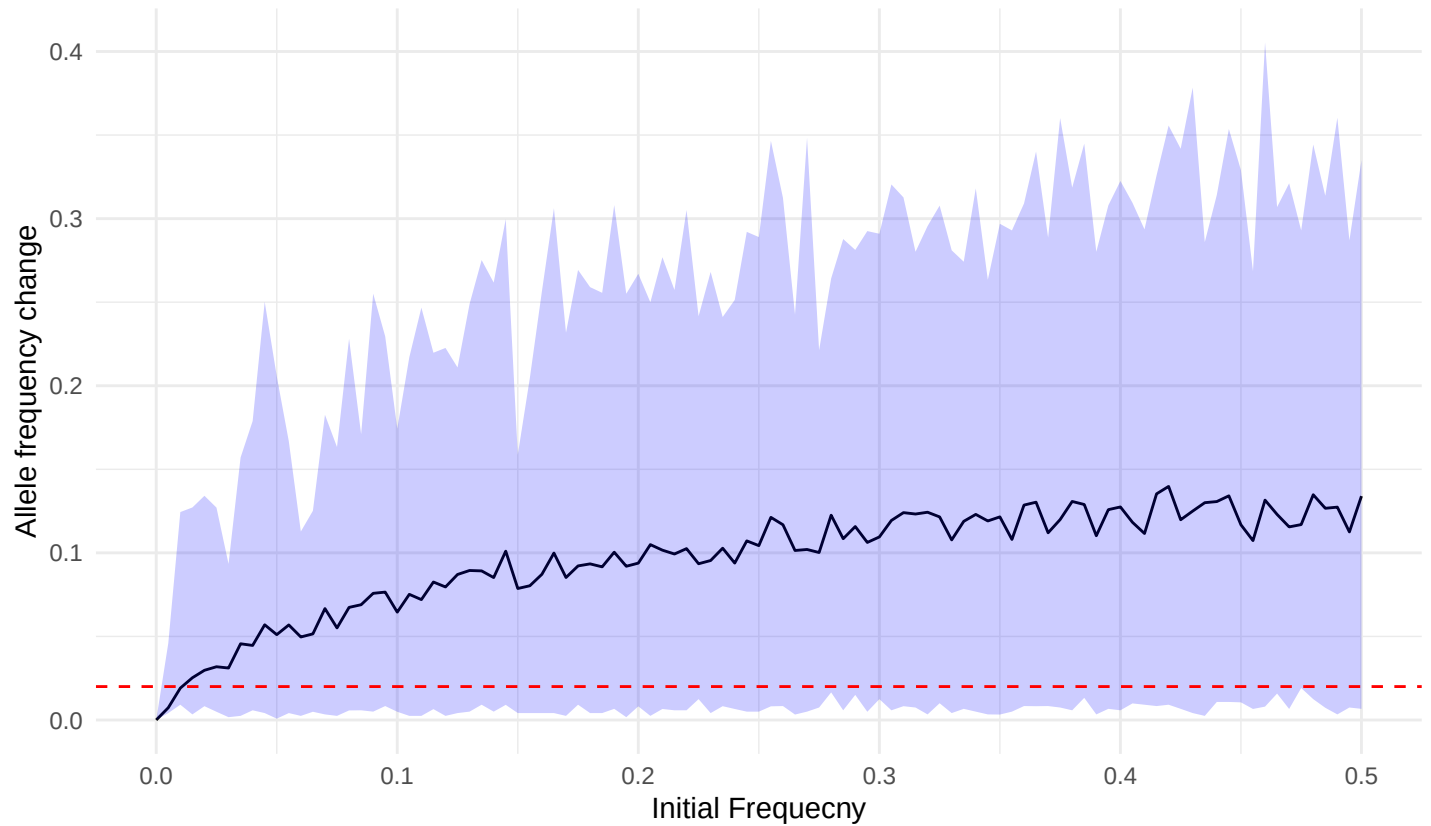
Expected AFC under Neutrality_Ne300_Gen60
