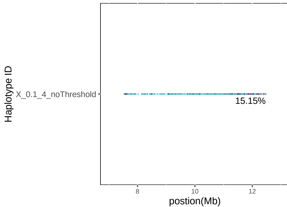
Constant haplotypes
