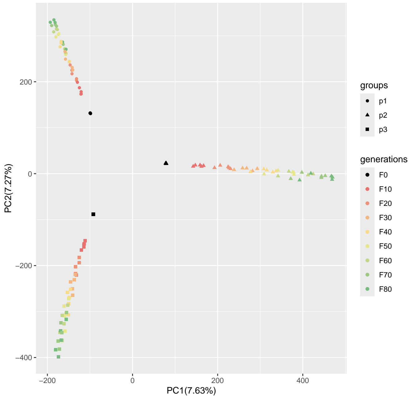
Run4_popsiz1250_n400_20000loci_s100
