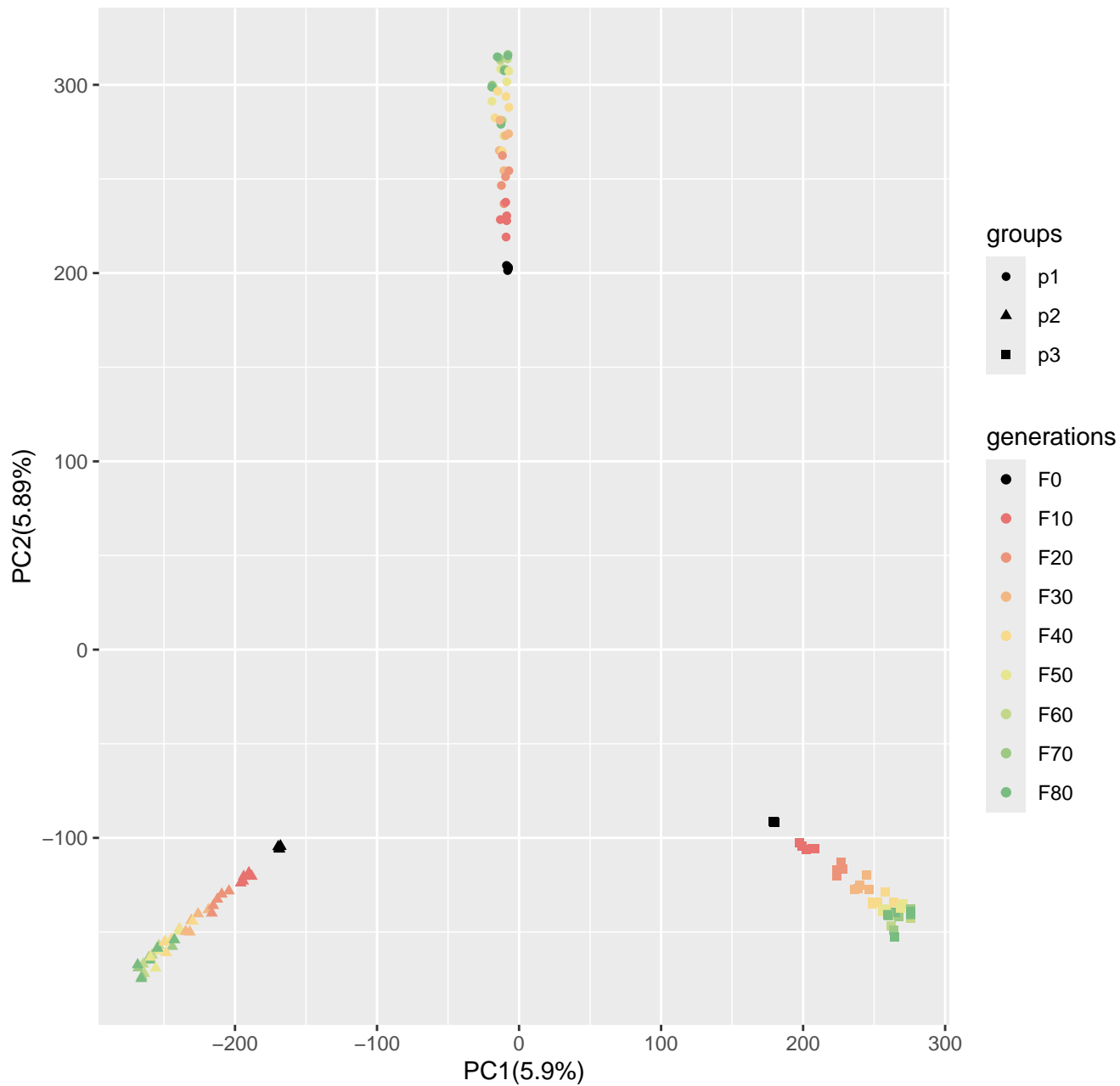
Run2_popsizel250_n400_20000loci_s10
