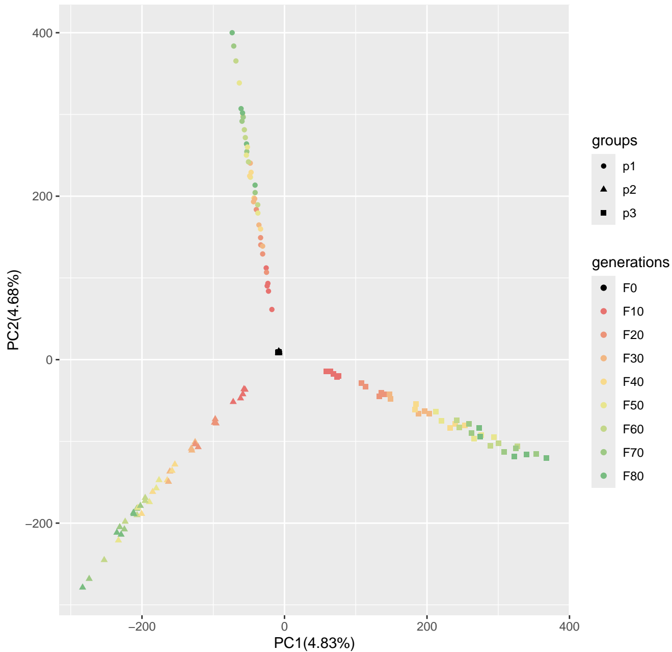
Run8_popsizel250_n400_20000loci_s50
