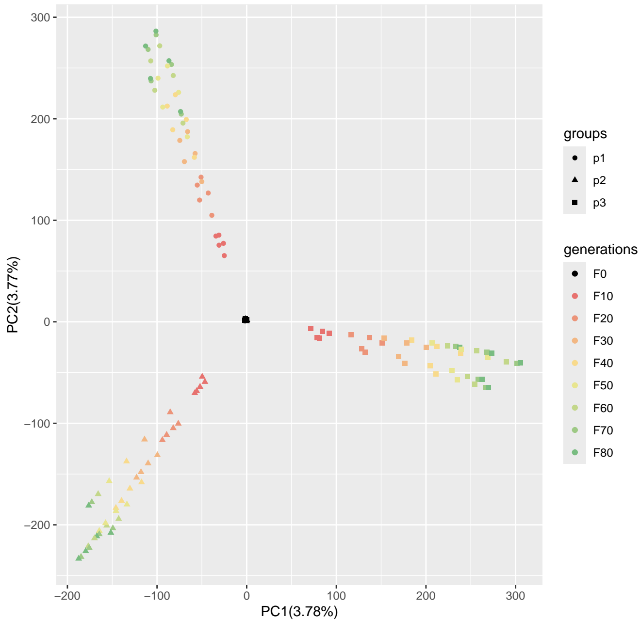
Run5_popsizel250_n400_5000loci_s50
