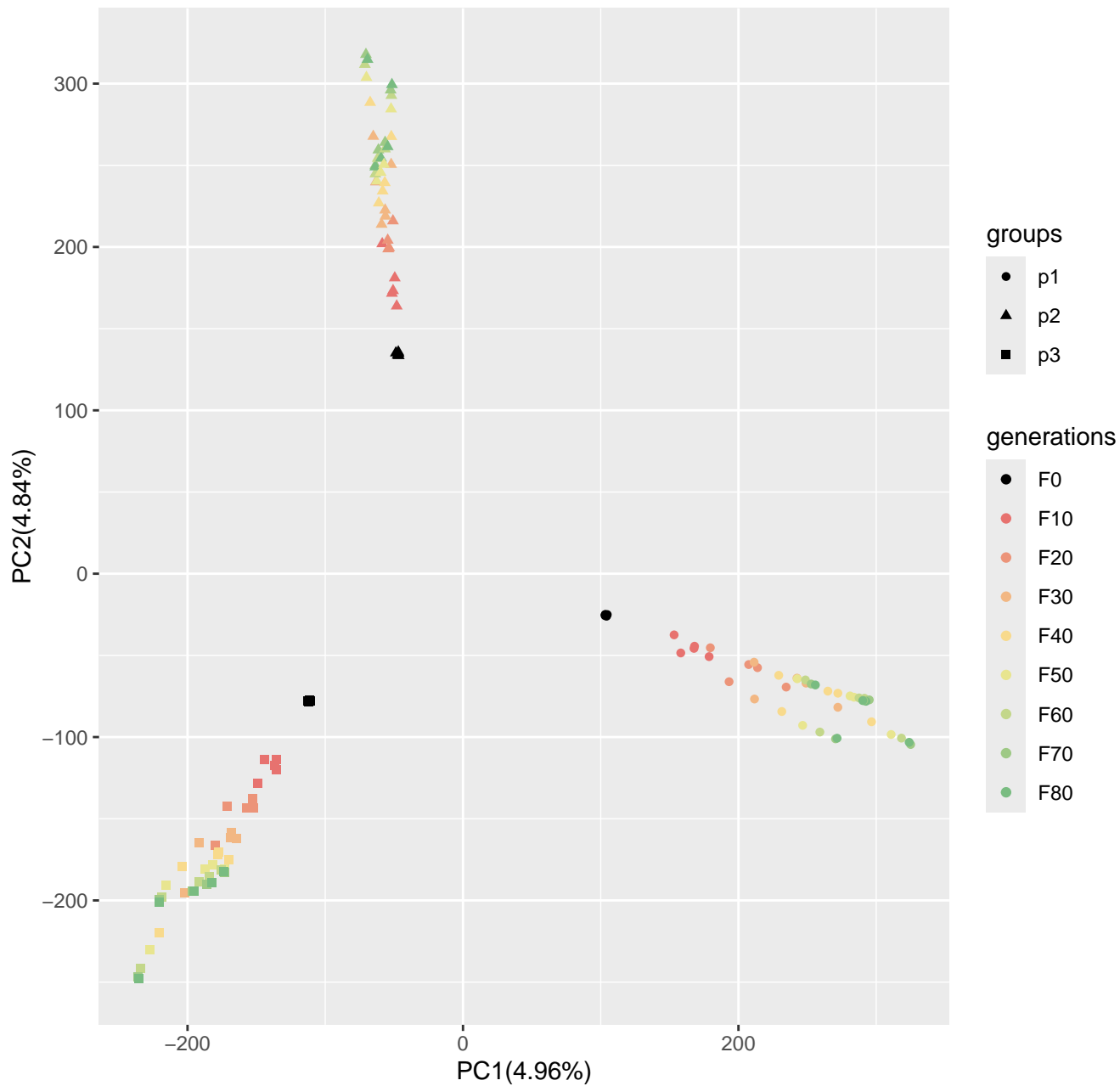
Run7_popsiz300_n400_10loci_s0
