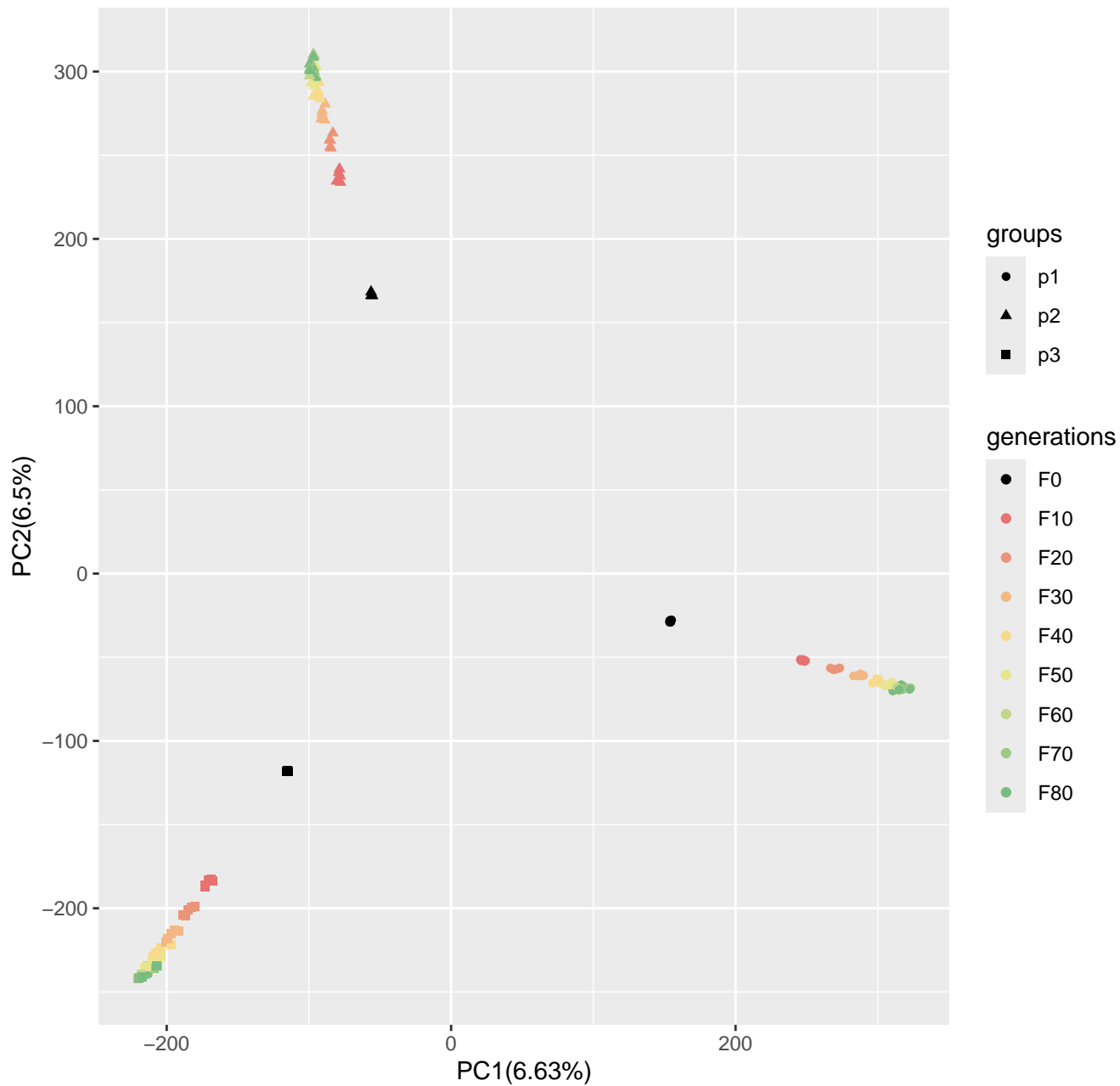
Run8_popsizel250_n400_1000loci_s50
