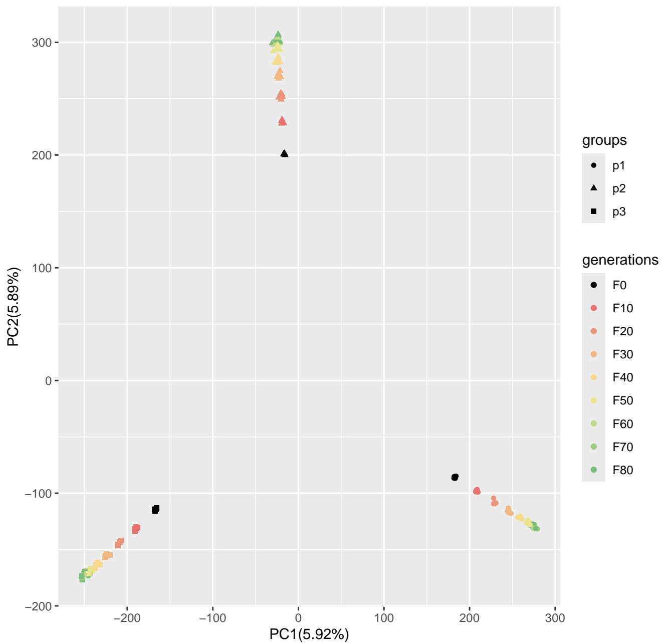
Run5_popsizel250_n400_10000loci_s10
