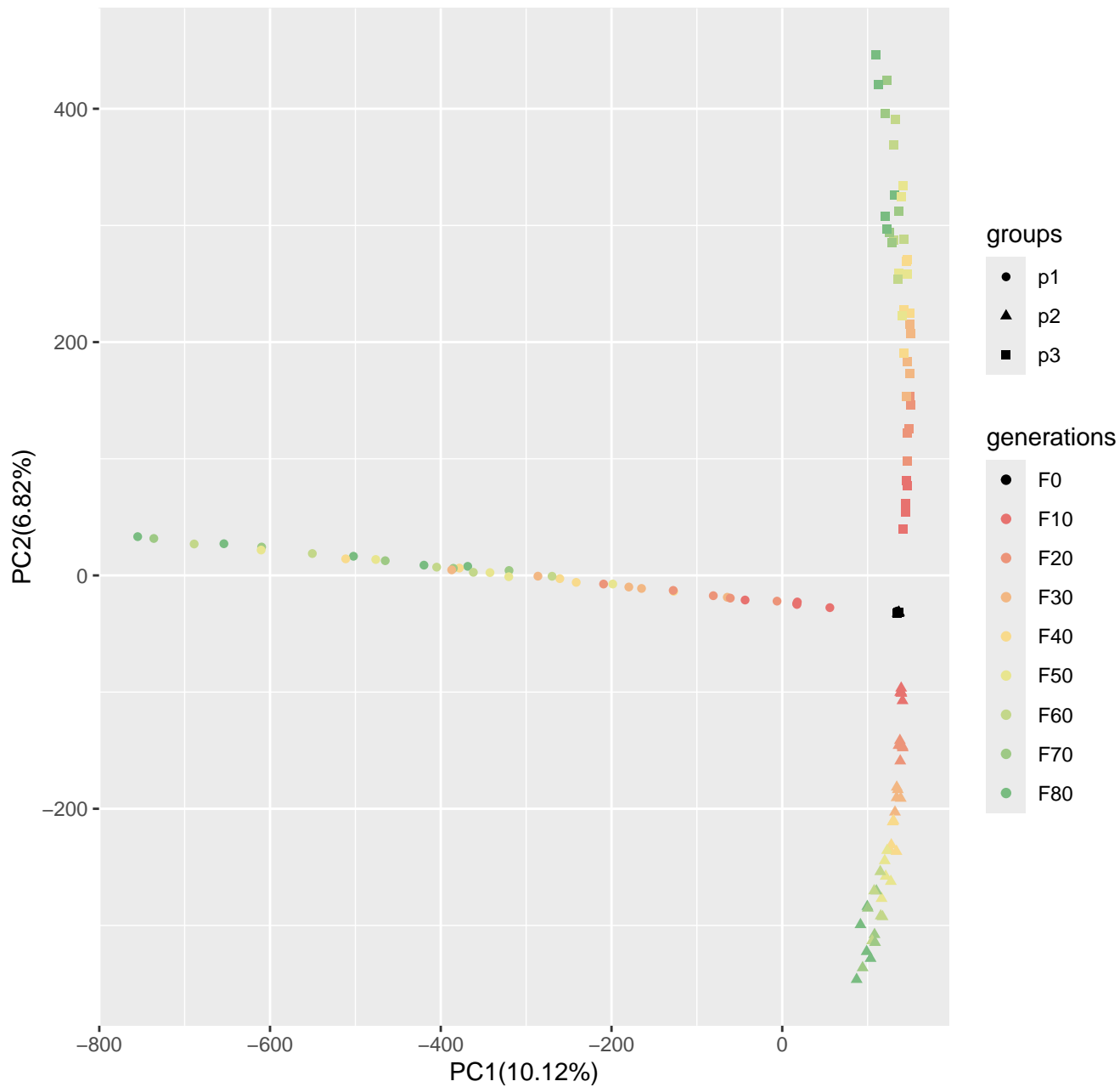
Run7_popsizel250_n400_20000loci_s100
