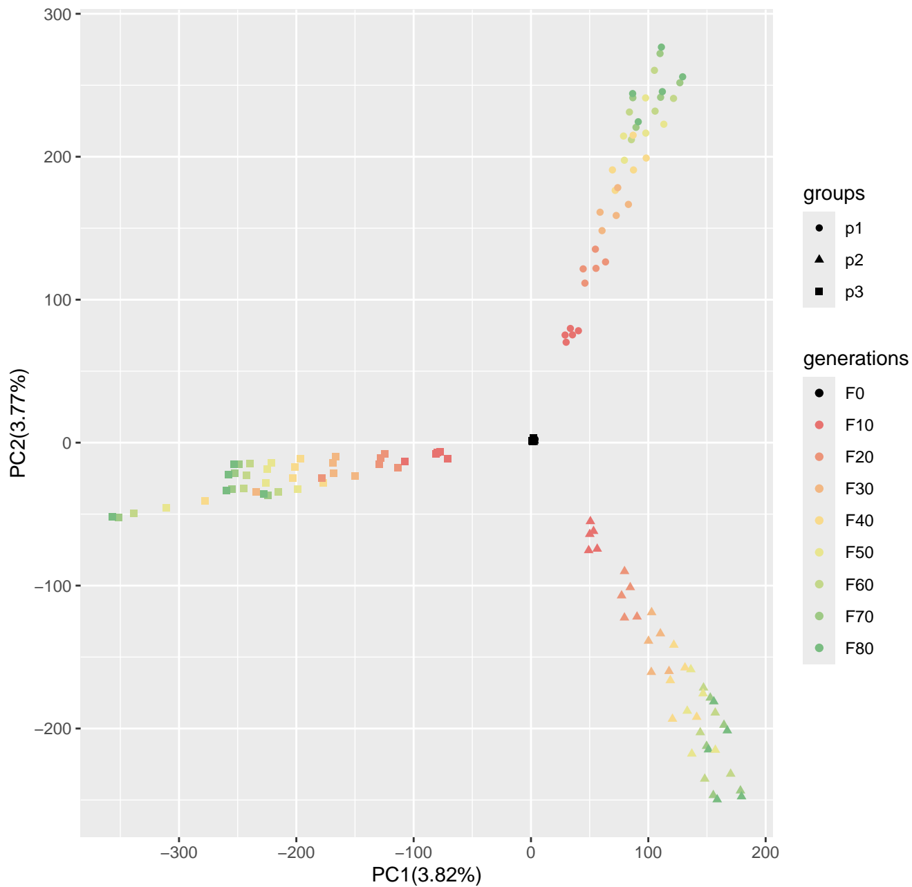
Run9_popsizel250_n400_20000loci_s100
