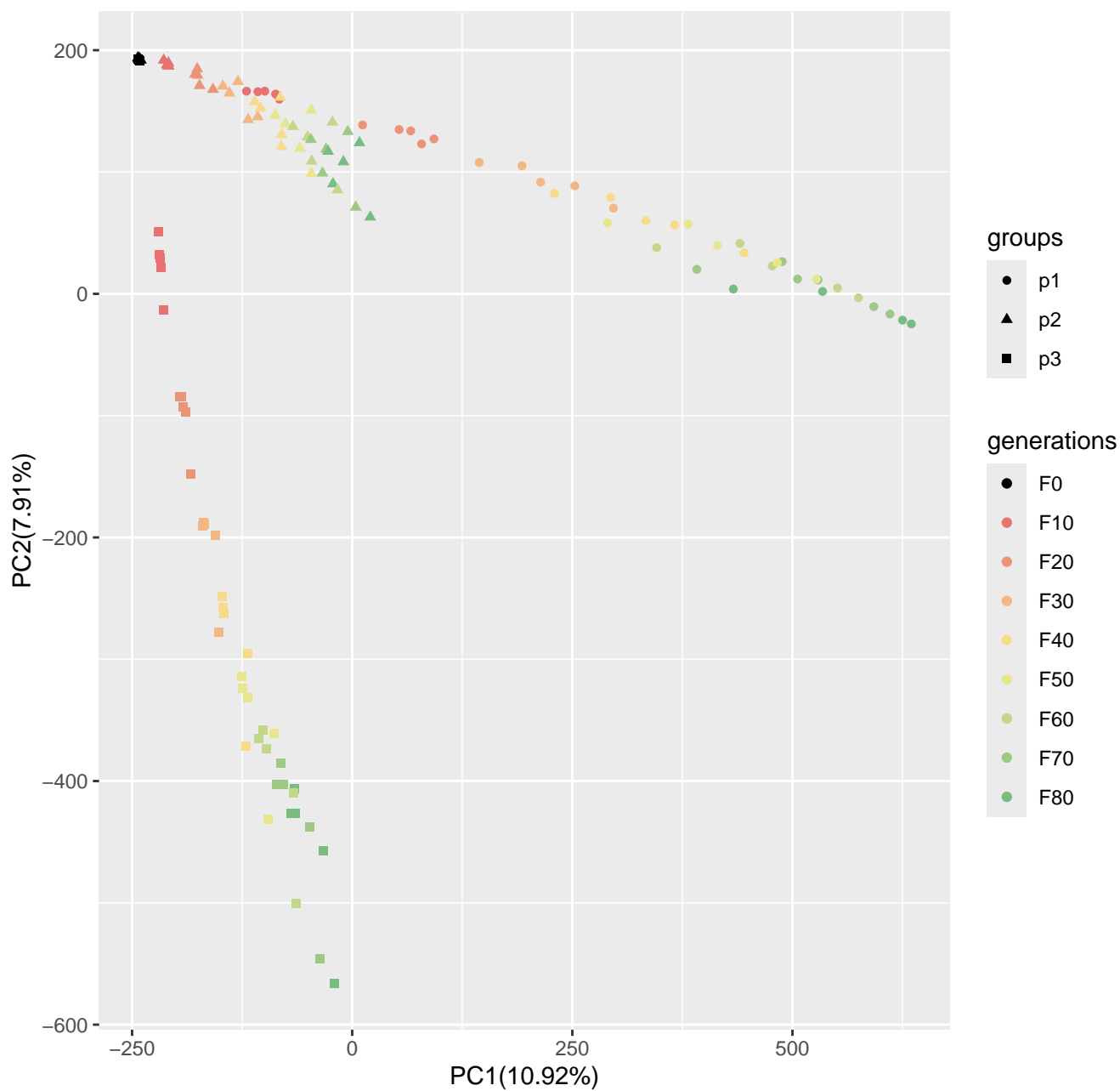
Run10_popsizel2500_n400_100loci_s10
