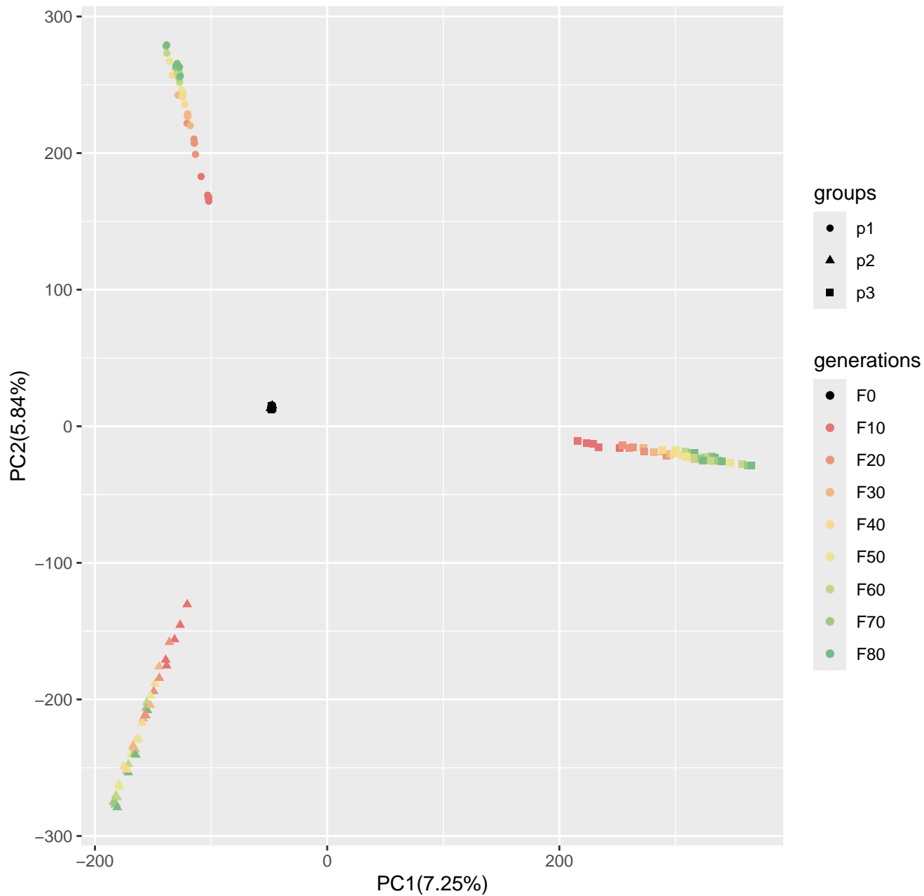
Run4_popsiz1250_n400_10loci_s10
