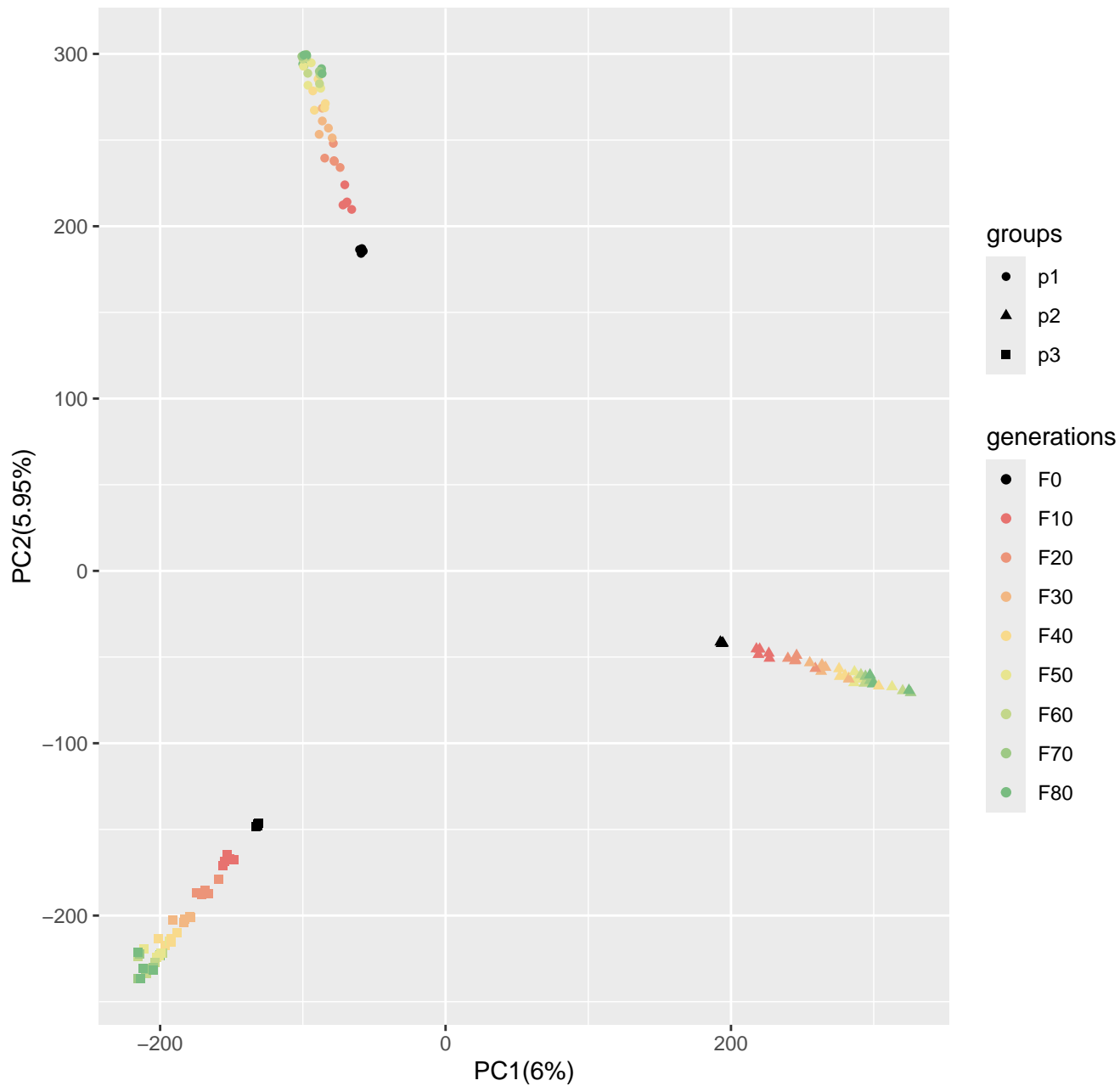
Run8_popsizel250_n400_5000loci_s10
