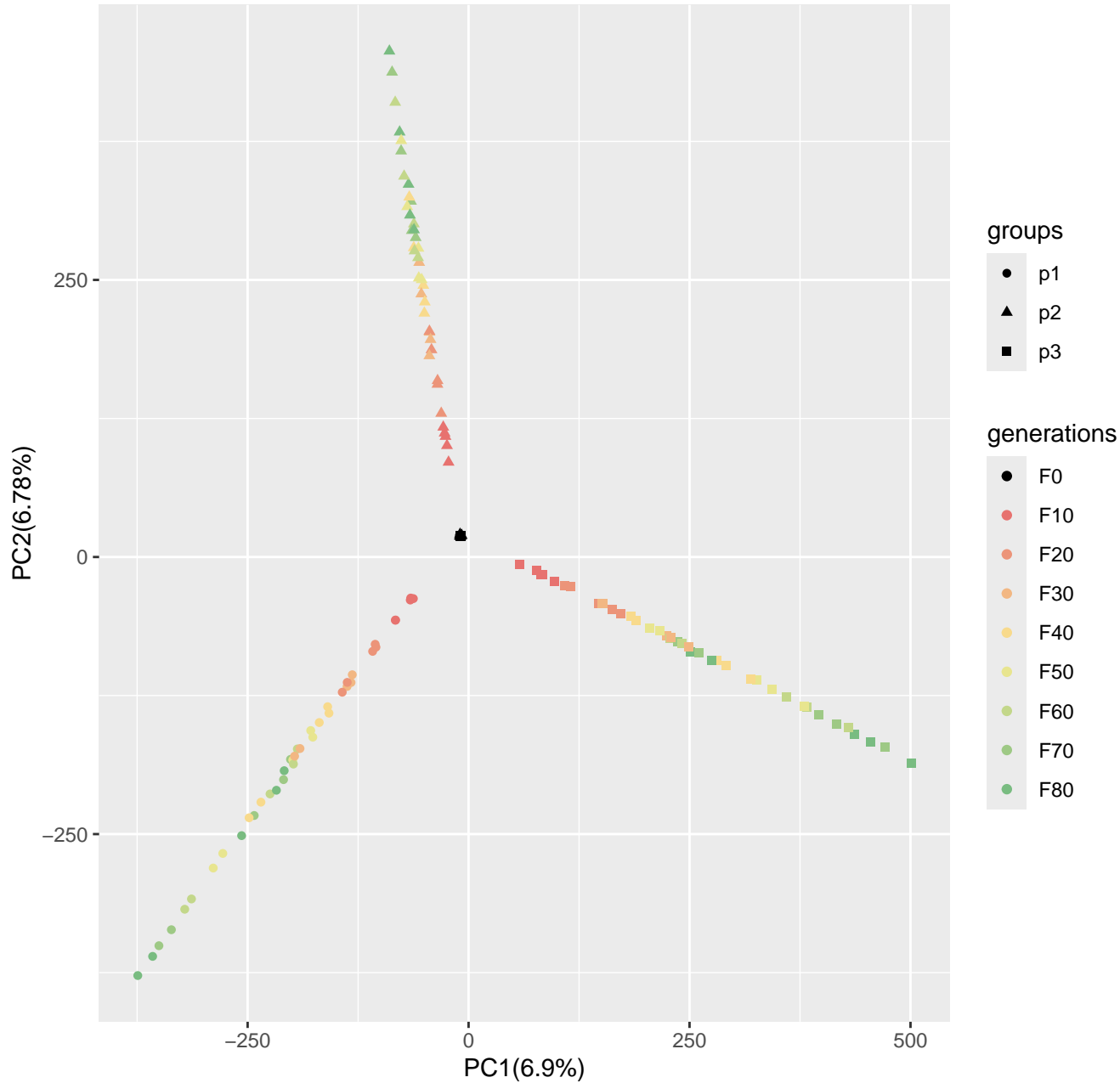
Run2_popsizel250_n400_20000loci_s100
