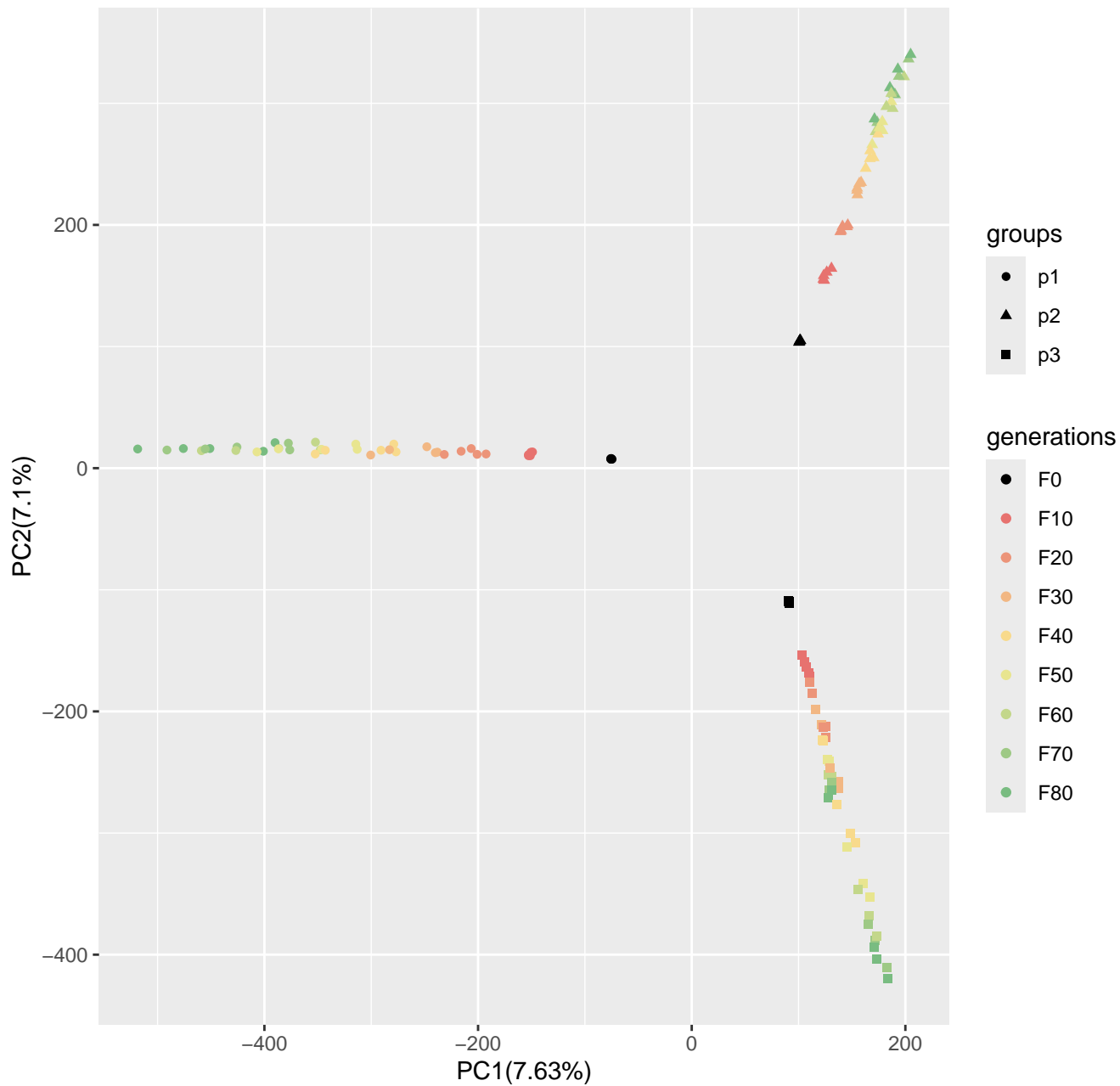
Run2_popsizel250_n400_5000loci_s50
