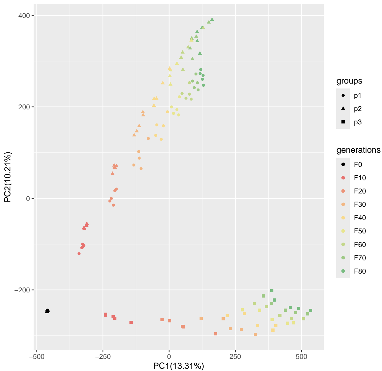
Run2_popsizel250_n400_1000loci_s50
