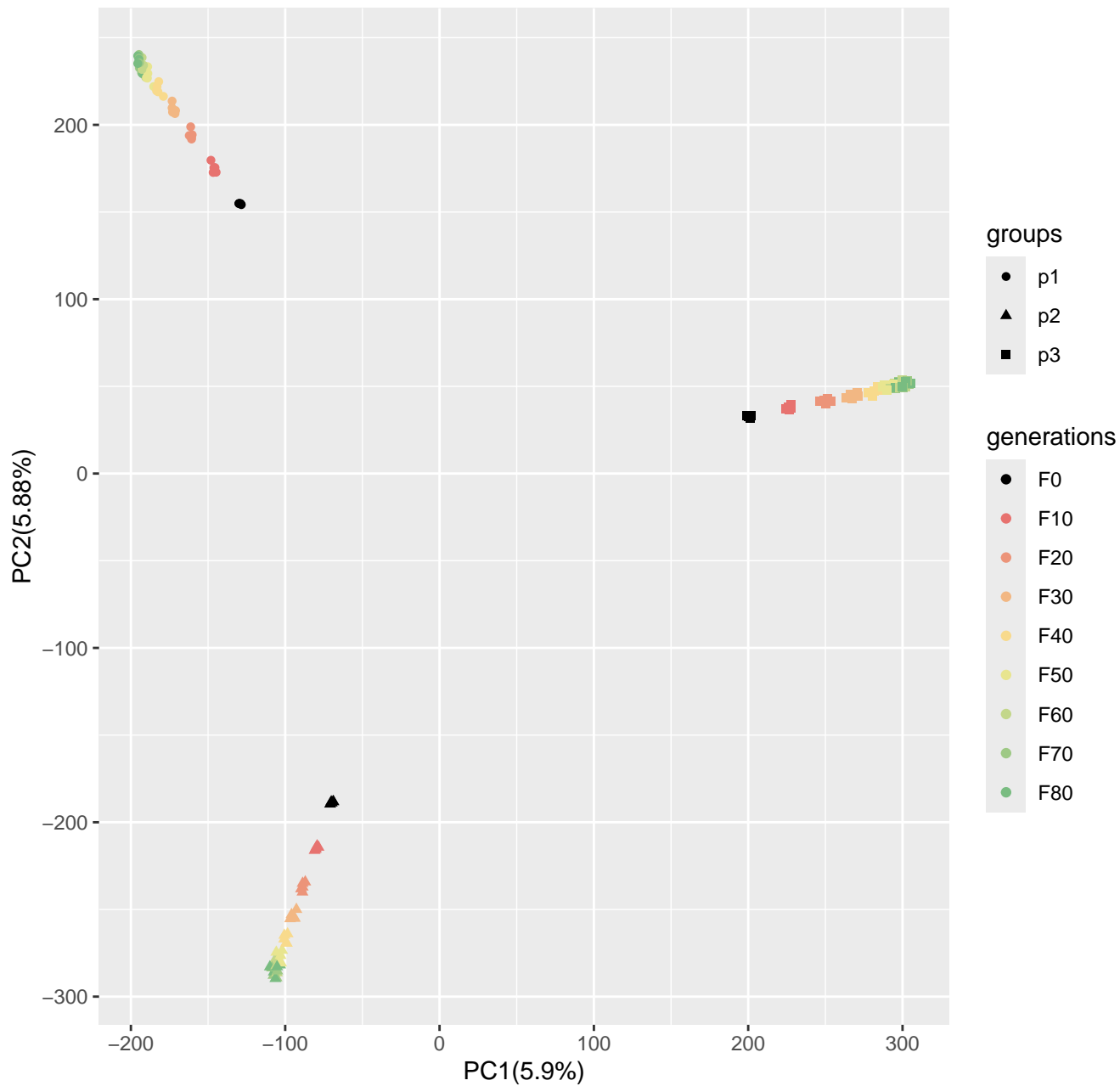
Run1_popsizel250_n400_20000loci_s10
