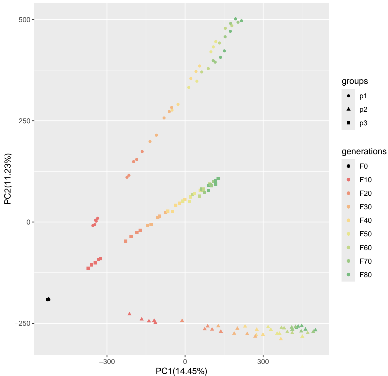
Run4_popsizel250_n400_1000loci_s50
