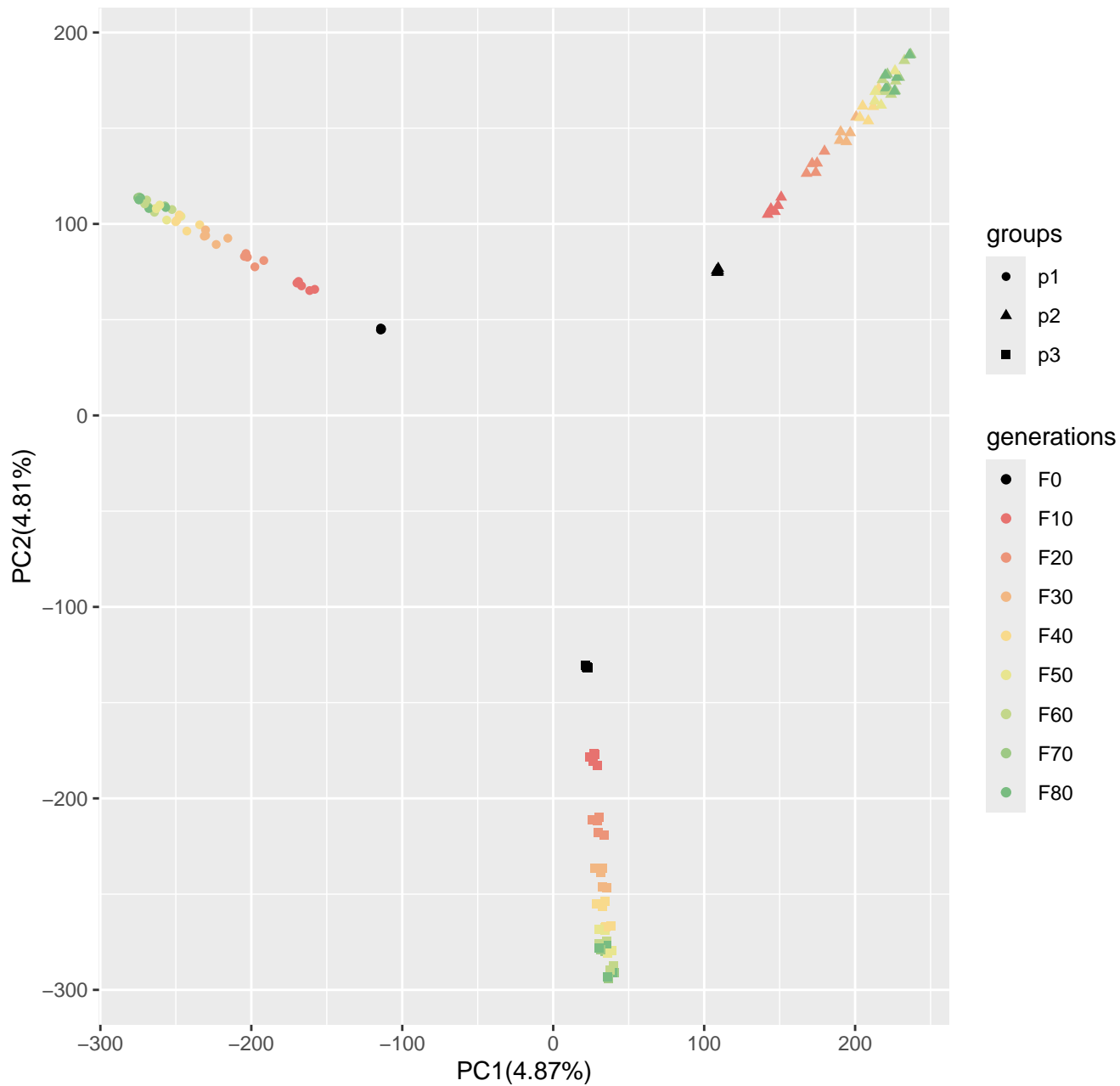
Run10_popsize300_n400_10loci_s0
