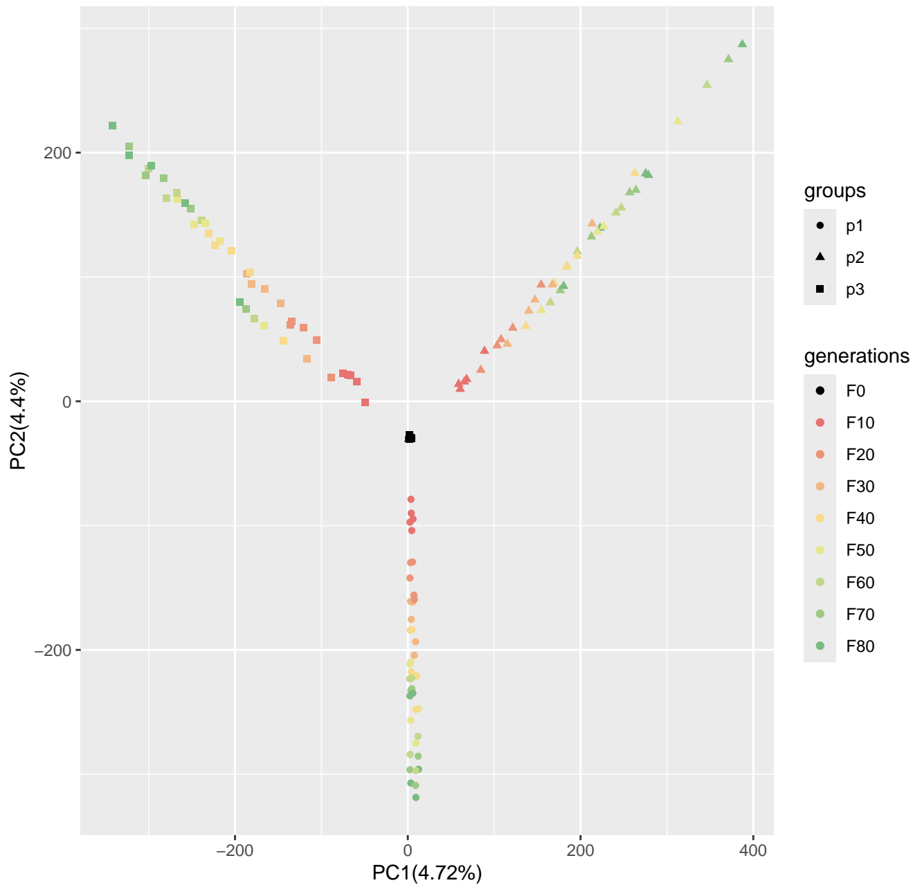
Run5_popsiz1250_n400_1000loci_s10
