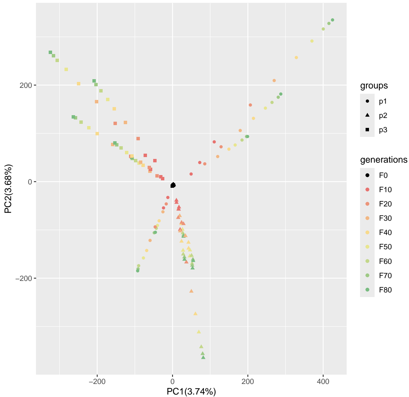
Run6_popsiz1250_n400_5000loci_s10
