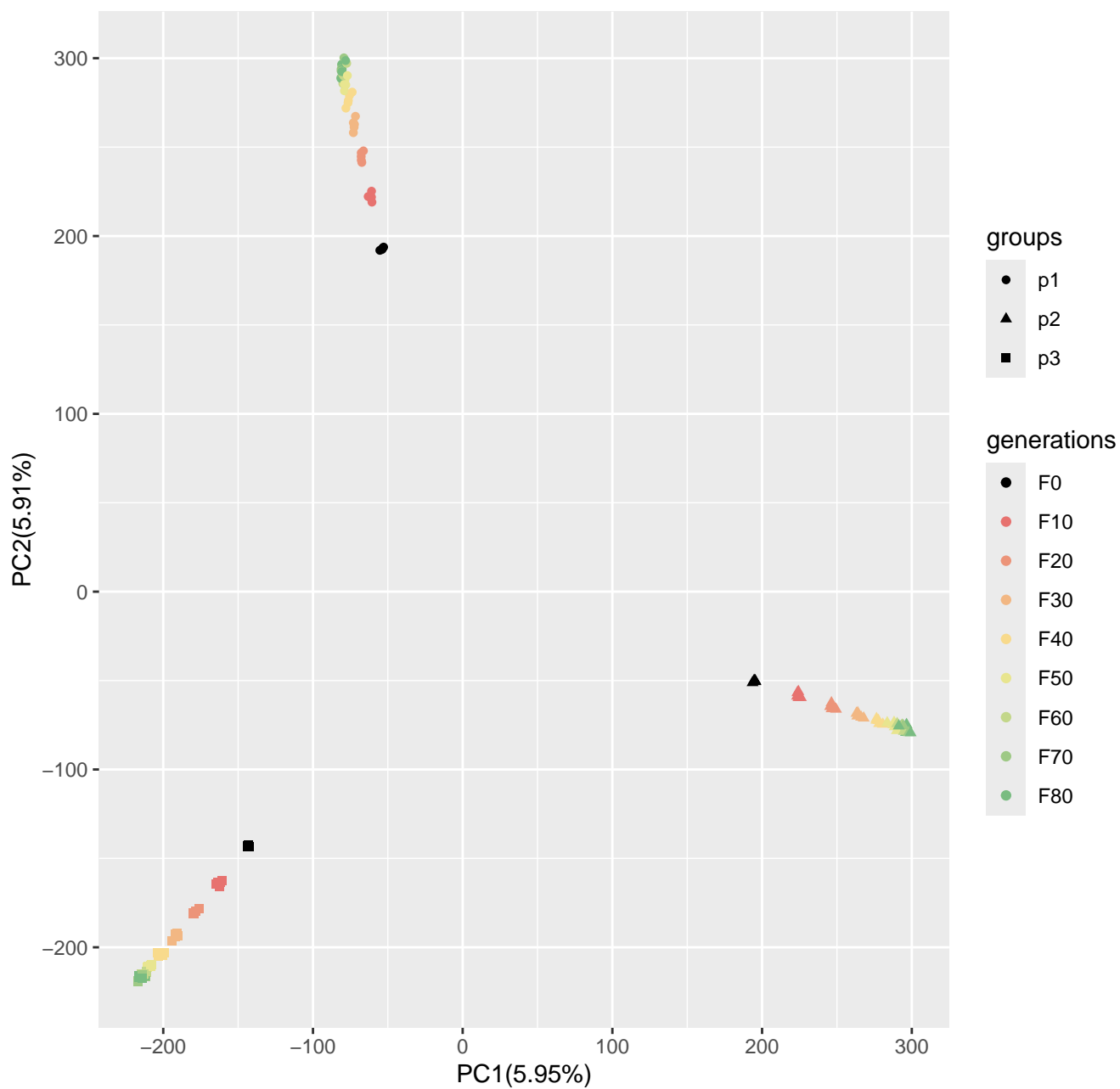
Run8_popsizel250_n400_1000loci_s10
