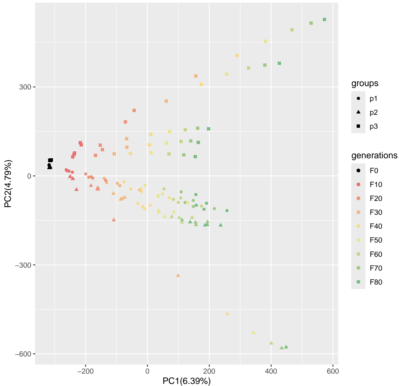
Run4_popsiz1250_n2500_100loci_s10
