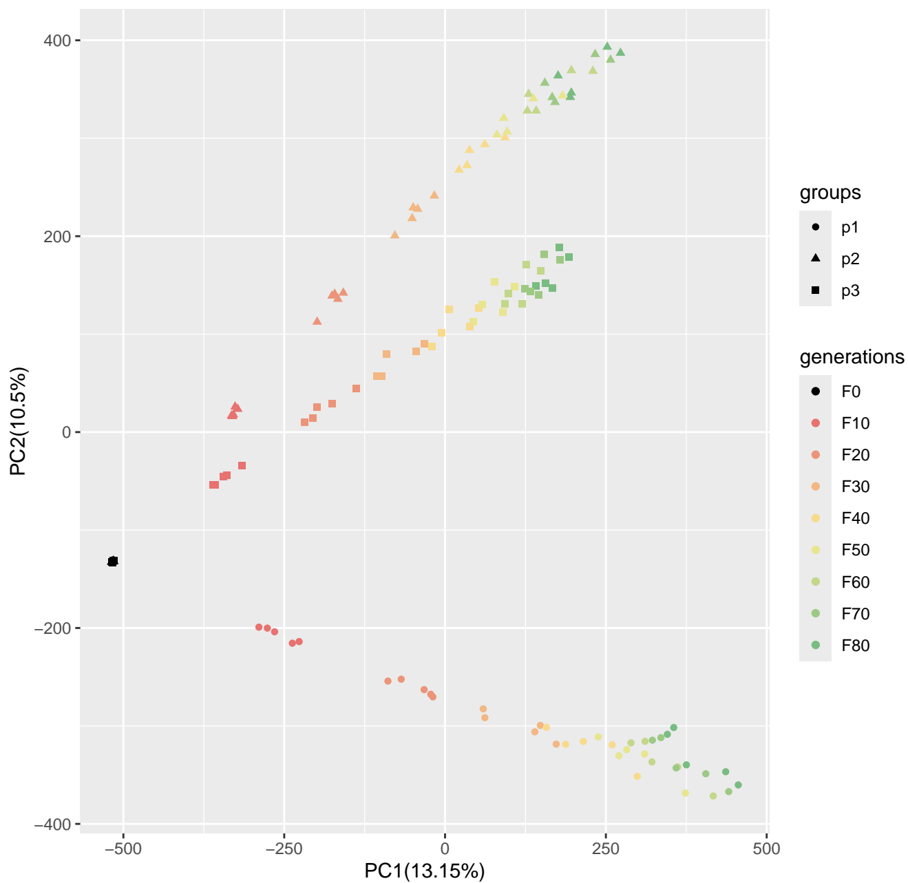
Run5_popsizel250_n400_1000loci_s50
