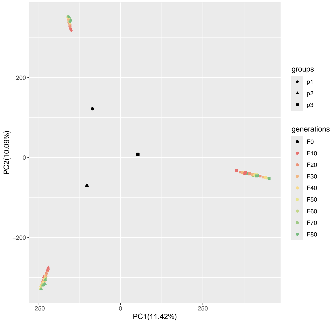
Run8_popsizel250_n400_10loci_s10
