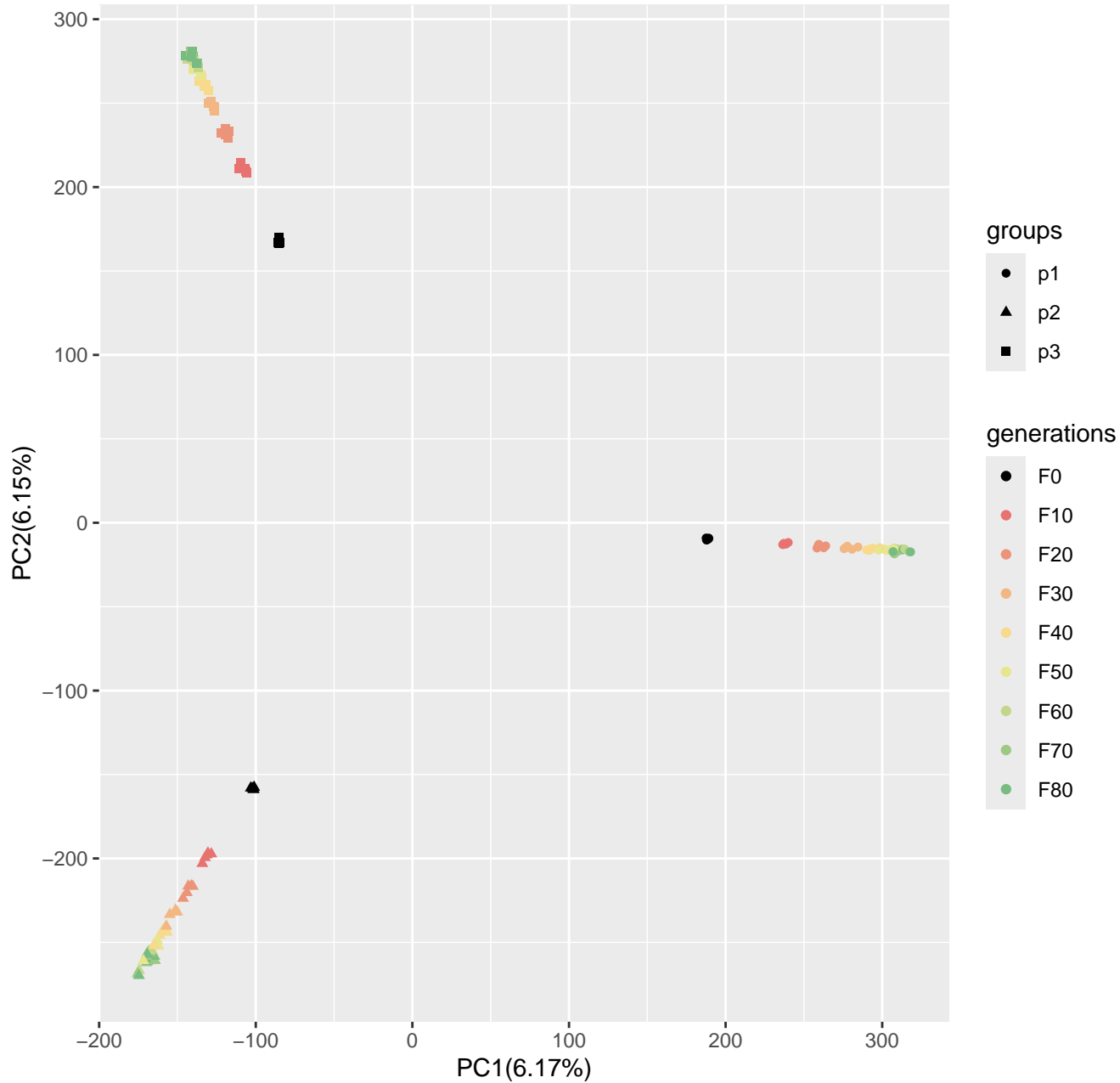
Run5_popsizel250_n400_10000loci_s100
