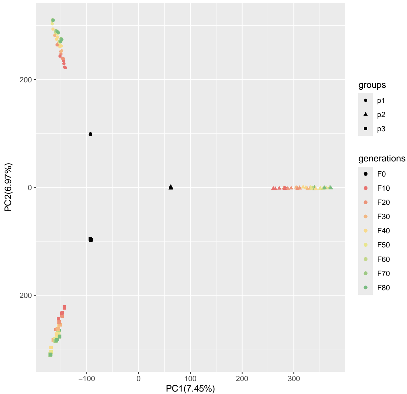
Run1_popsizel250_n400_1000loci_s100
