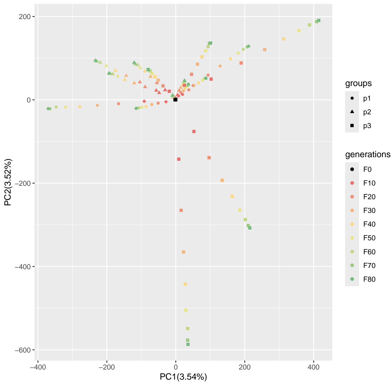
Run3_popsizel250_n400_20000loci_s10
