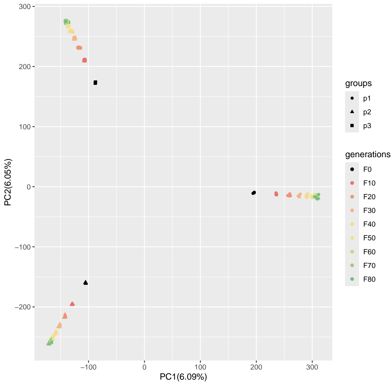
Run4_popsizel250_n400_20000loci_s100
