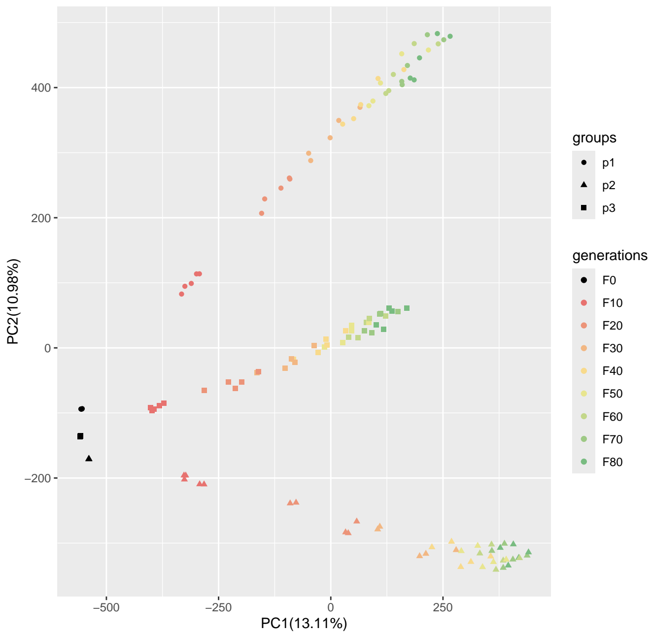
Run4_popsizel250_n400_1000loci_s50
