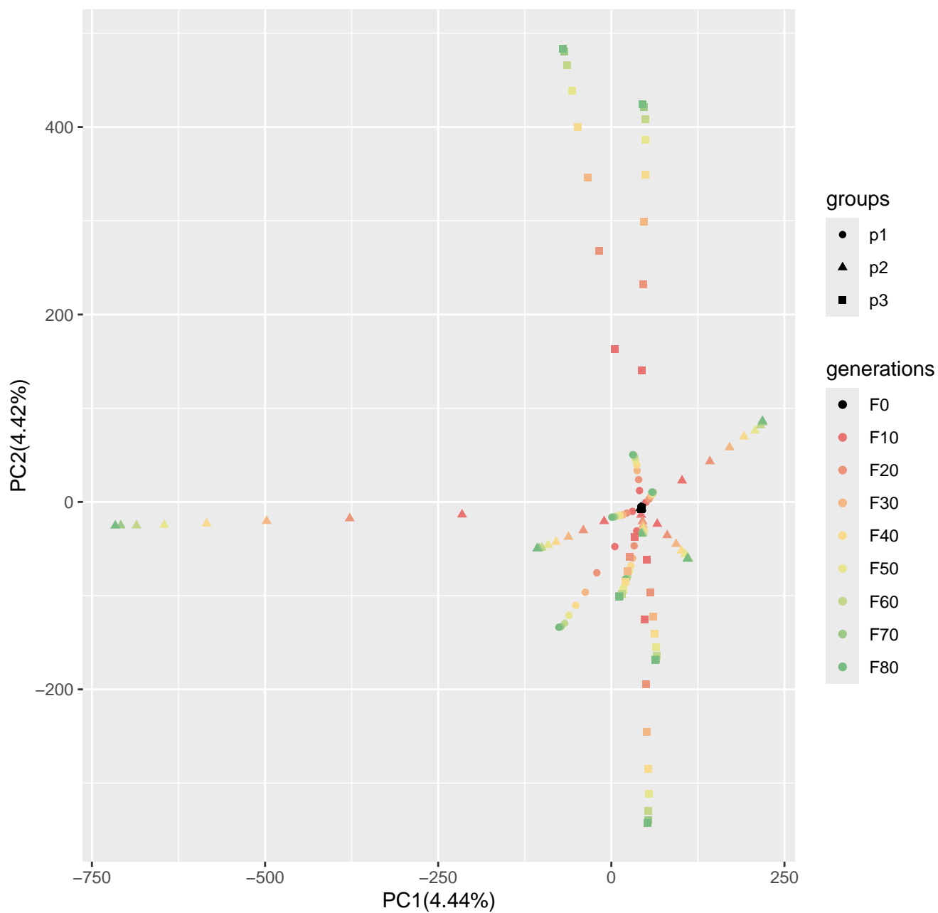
Run1_popsiz300_n400_10loci_s0
