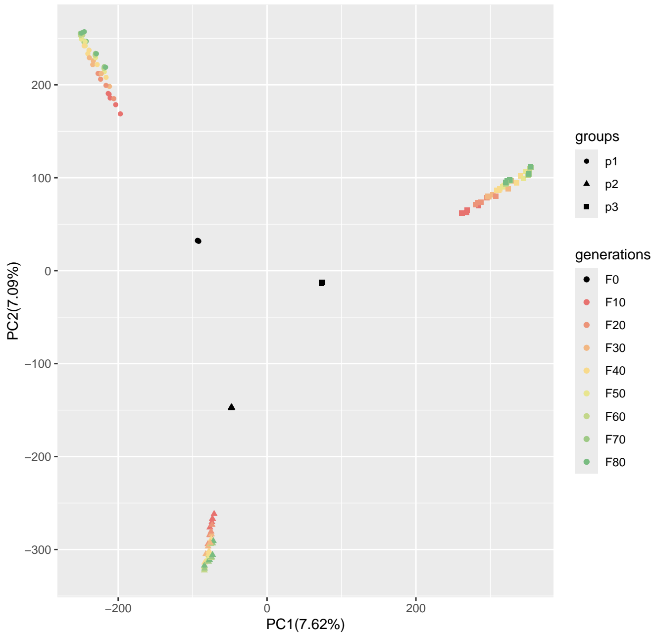
Run7_popsizel250_n400_1000loci_s100
