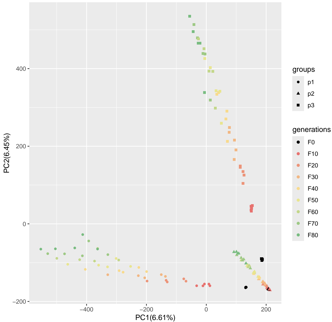
Run1_popsizel250_n800_100loci_s10
