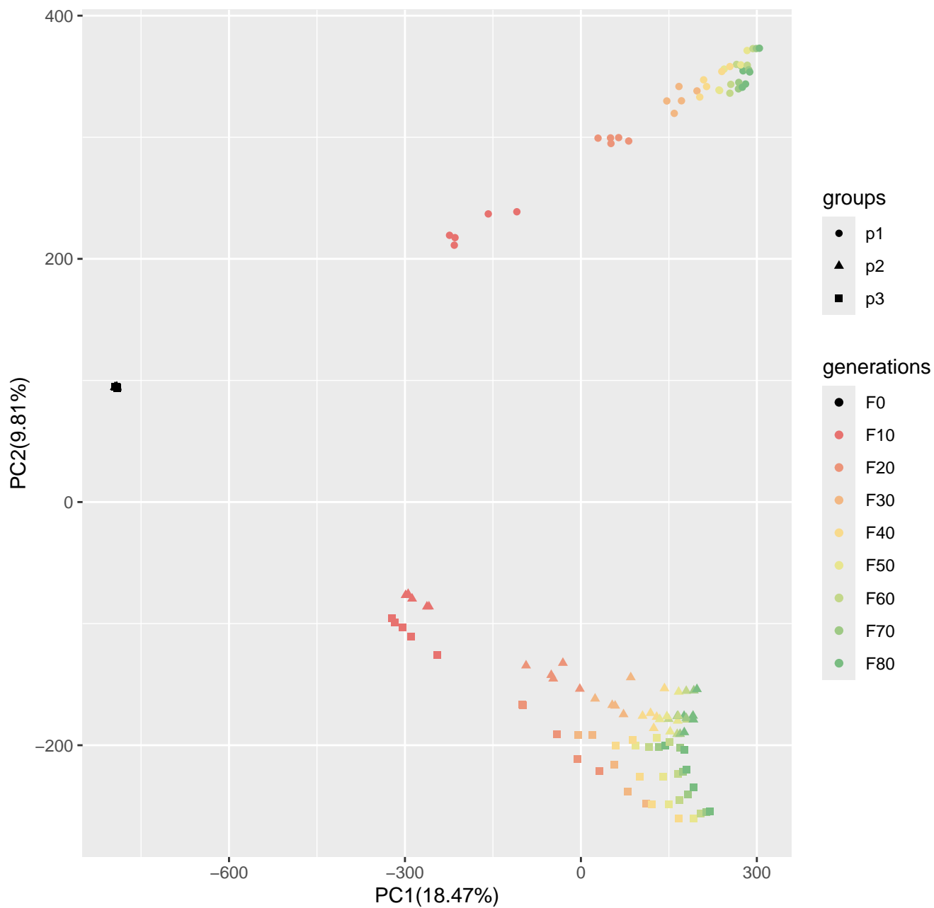
Run1_popsizel250_n400_1000loci_s100
