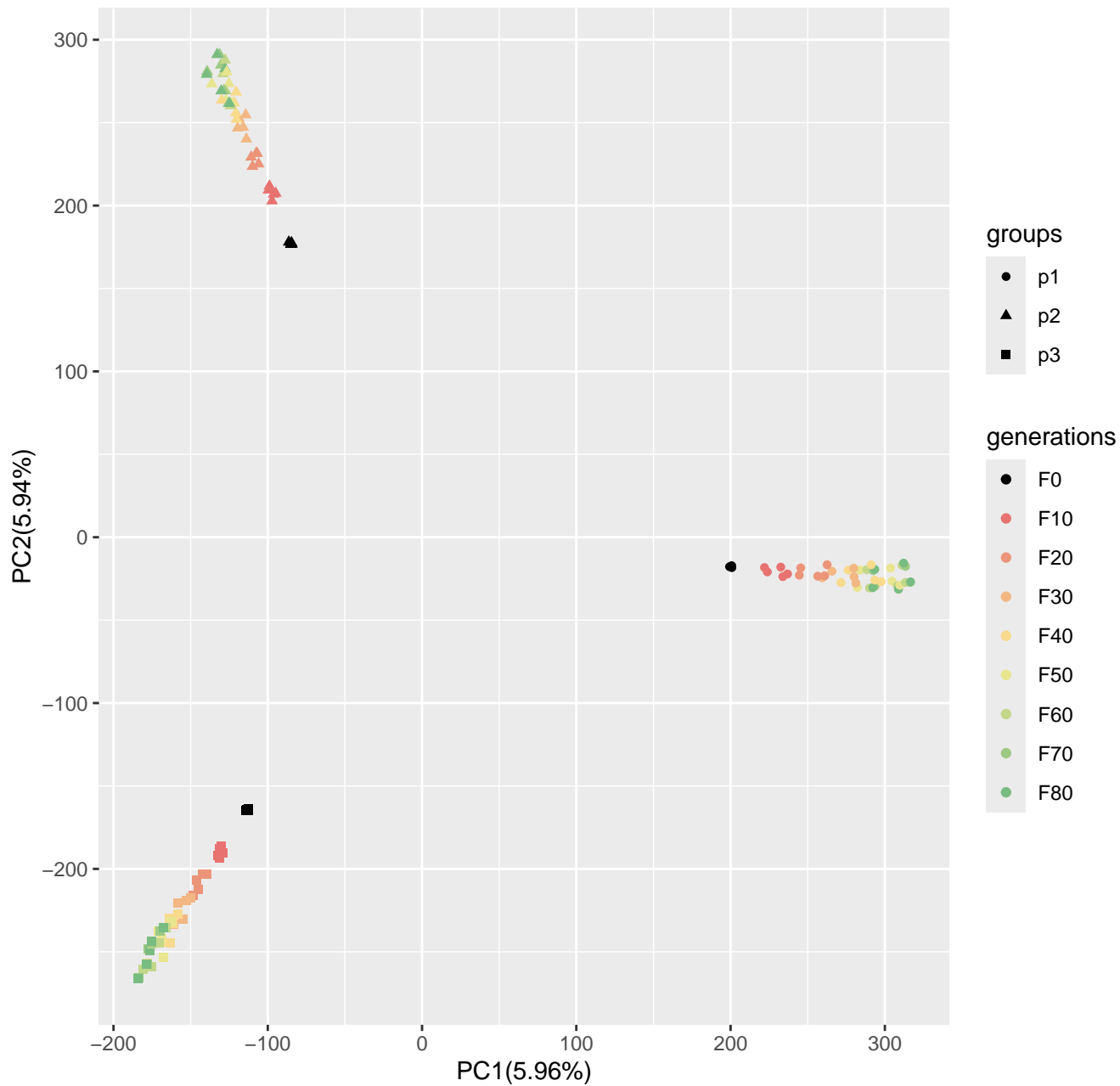
Run4_popsizel250_n400_20000loci_s10
