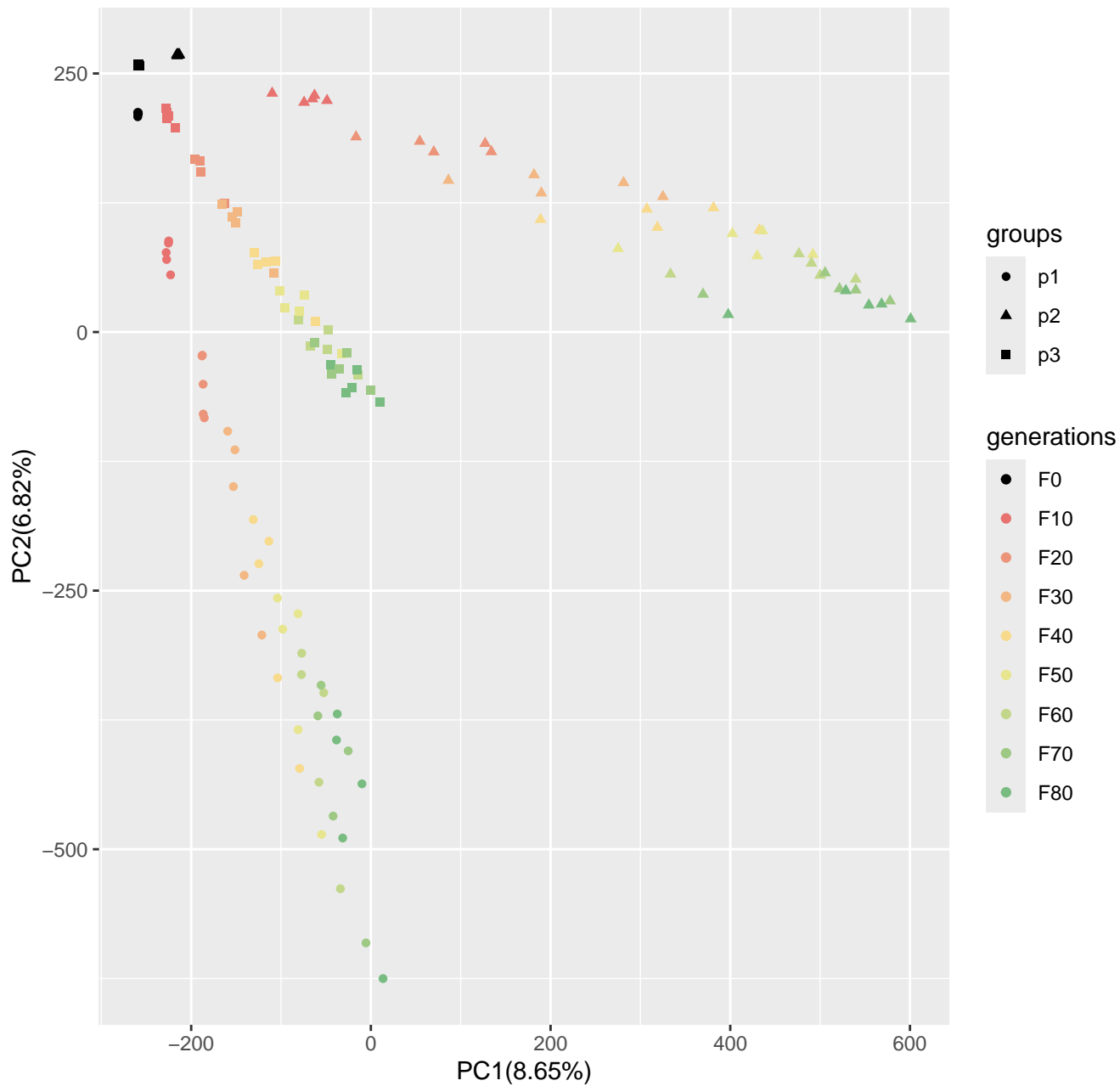
Run2_popsizel250_n800_100loci_s10
