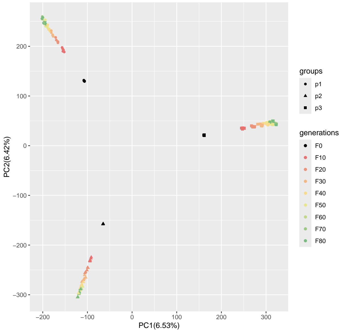
Run5_popsizel250_n400_1000loci_s50
