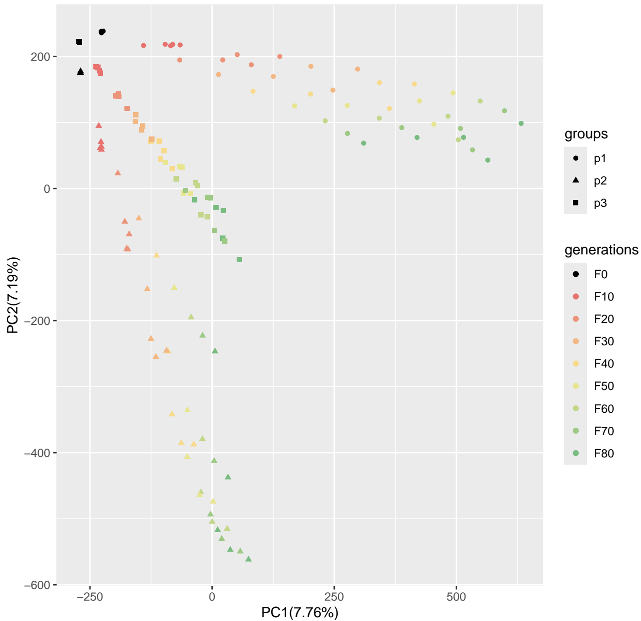
Run8_popsiz1250_n800_100loci_s10
