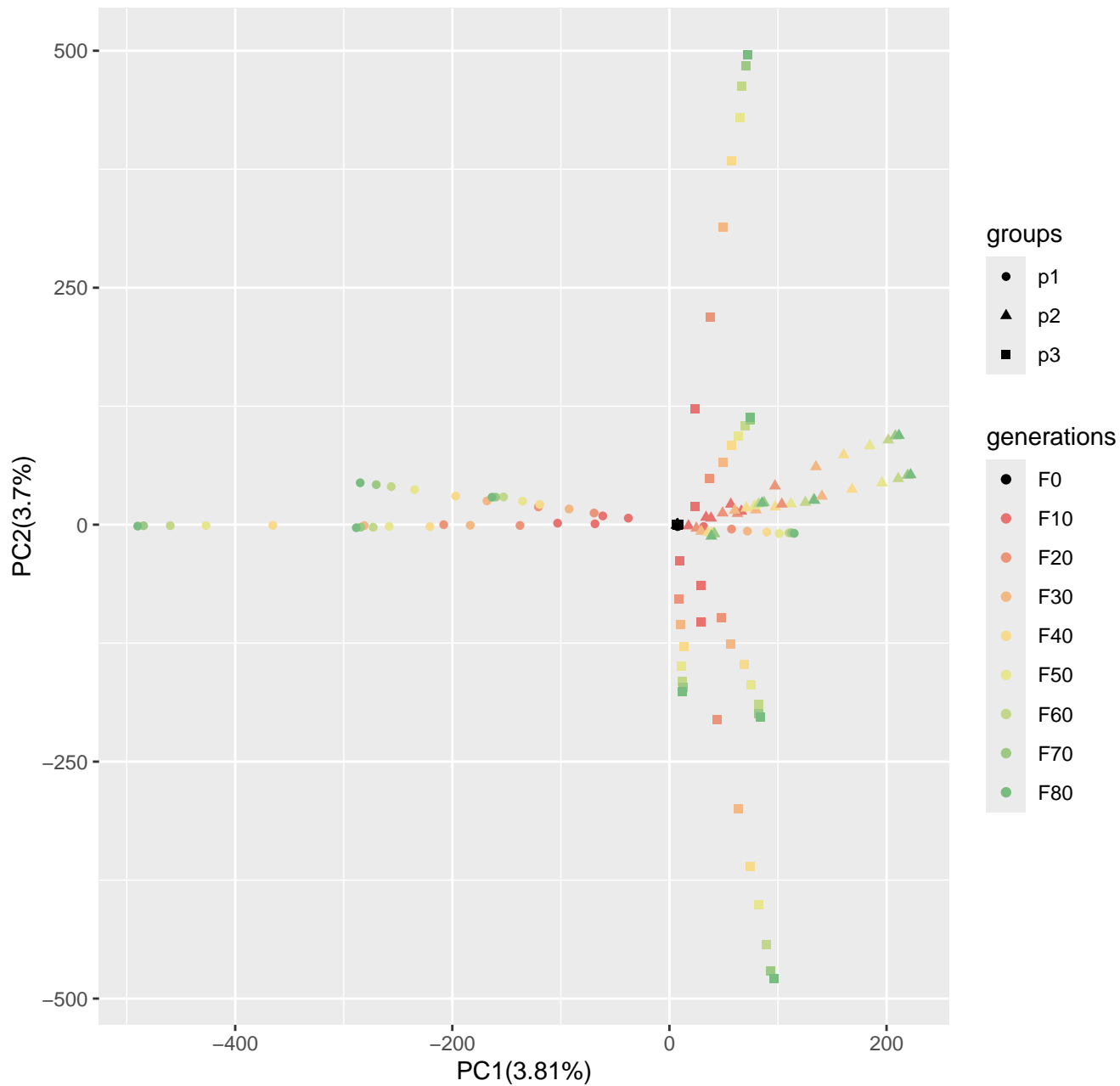
Run8_popsizel250_n400_10000loci_s10
