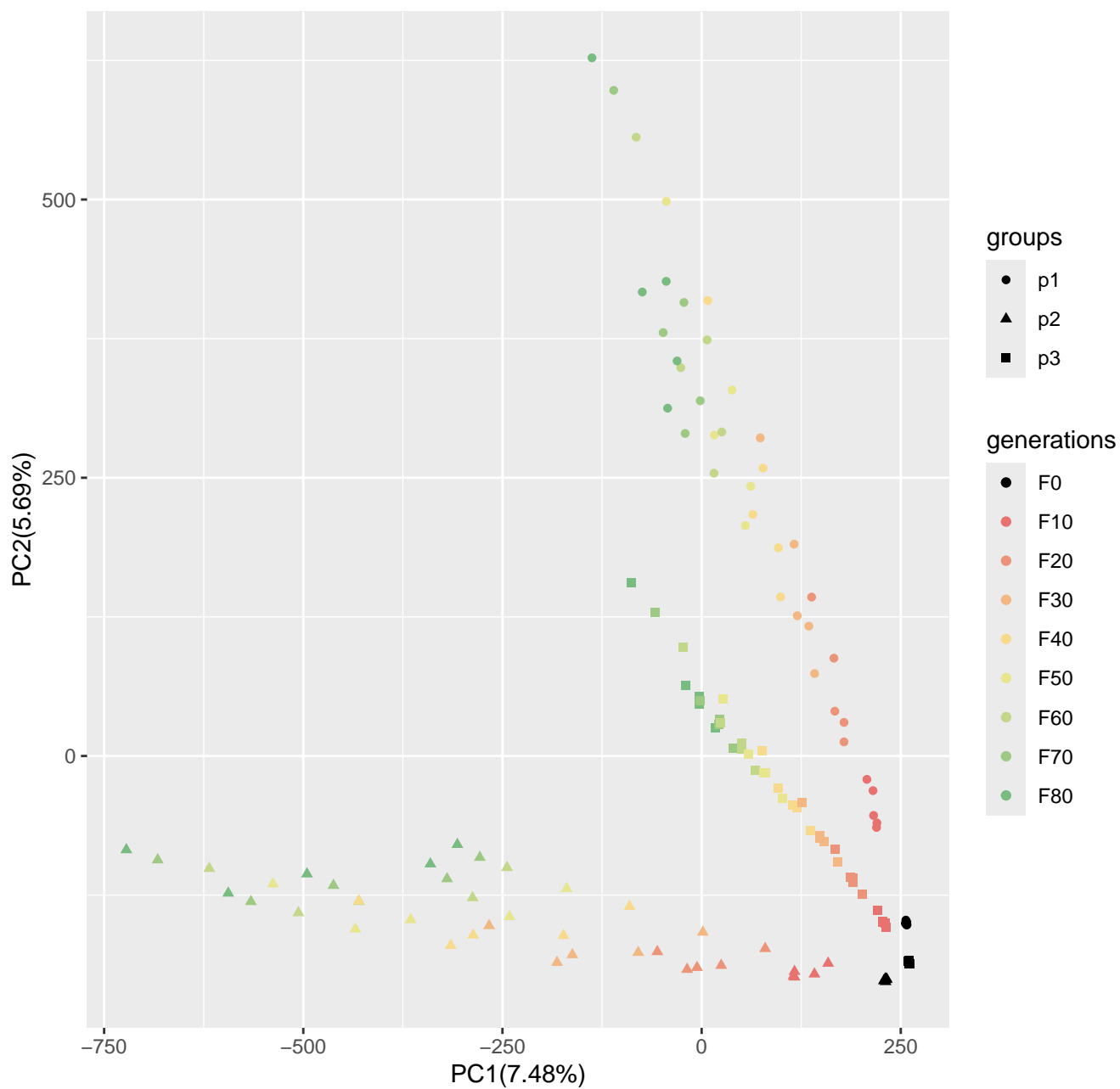
Run4_popsizel250_n1200_100loci_s10
