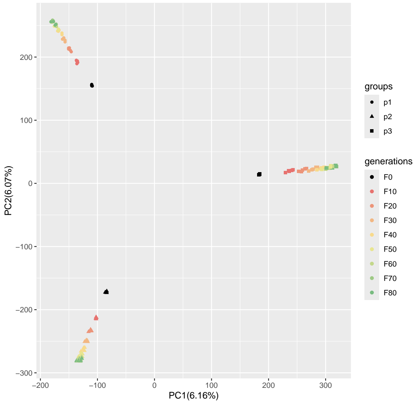
Run8_popsizel250_n400_10000loci_s100
