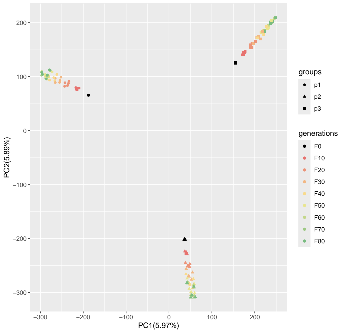
Run2_popsizel250_n400_10000loci_s10
