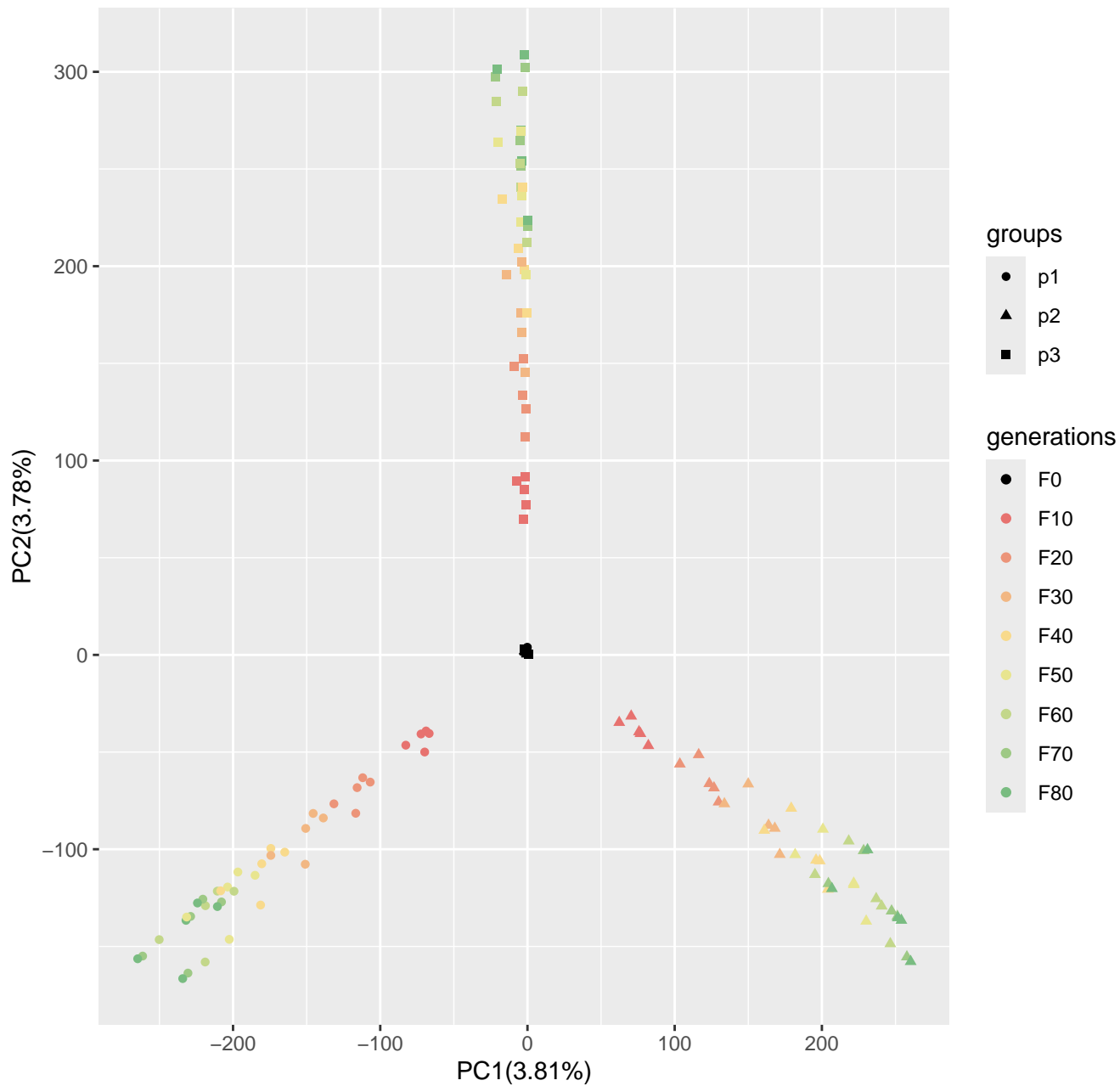
Run4_popsizel250_n400_20000loci_s100
