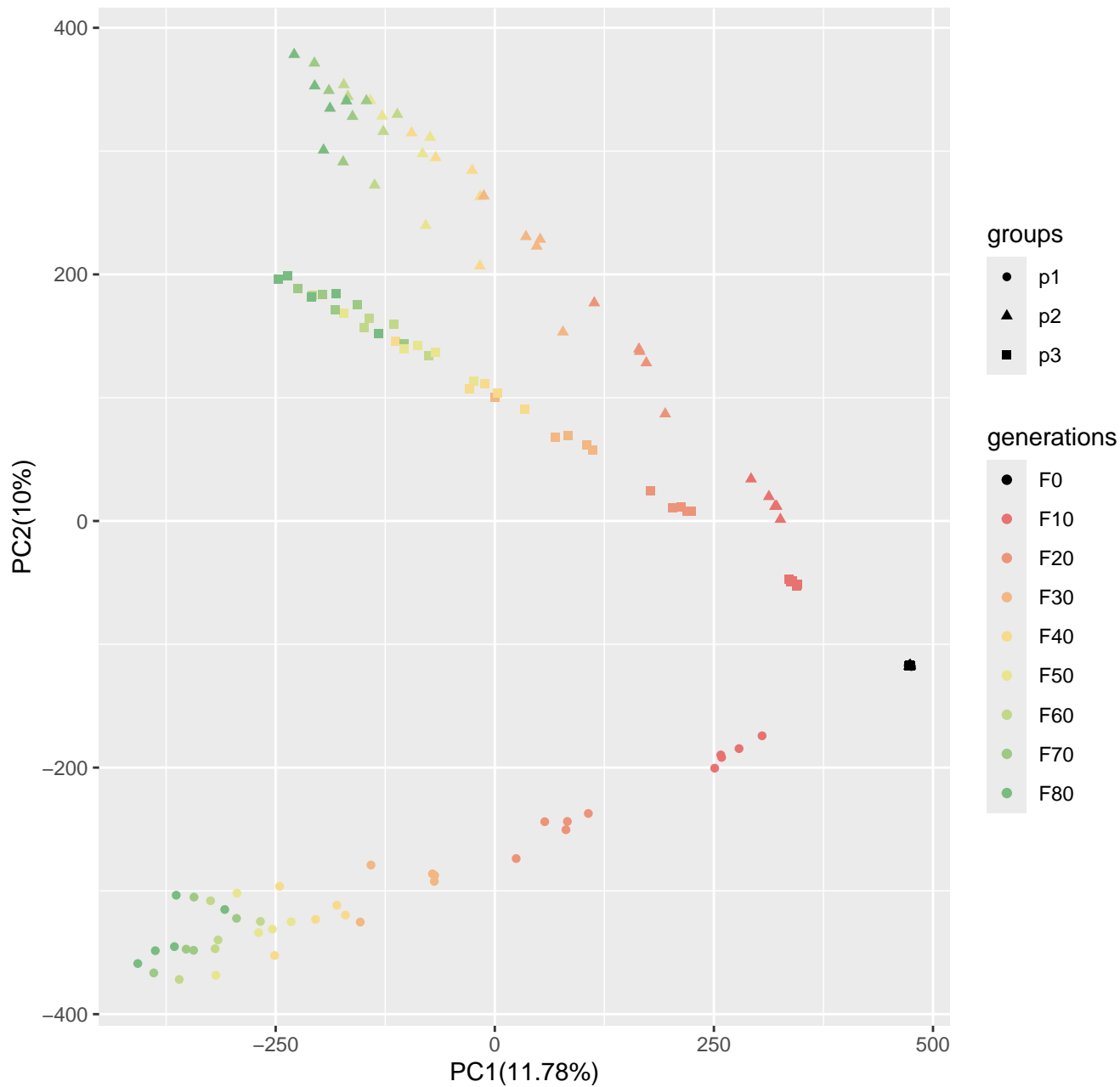
Run1_popsiz1250_n400_5000loci_s100
