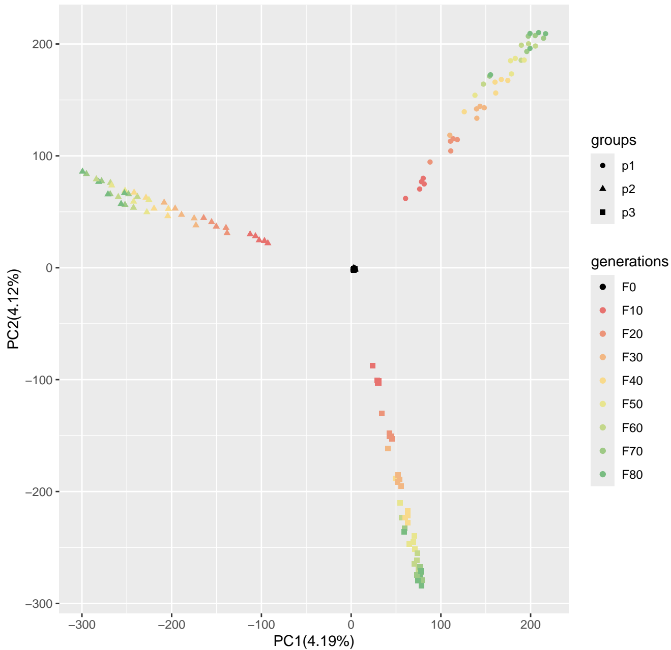
Run3_popsizel250_n400_10000loci_s100
