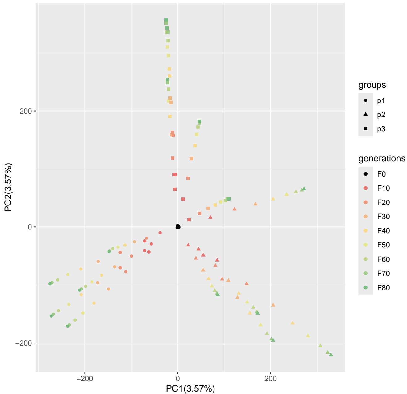
Run4_popsizel250_n400_1000loci_s10
