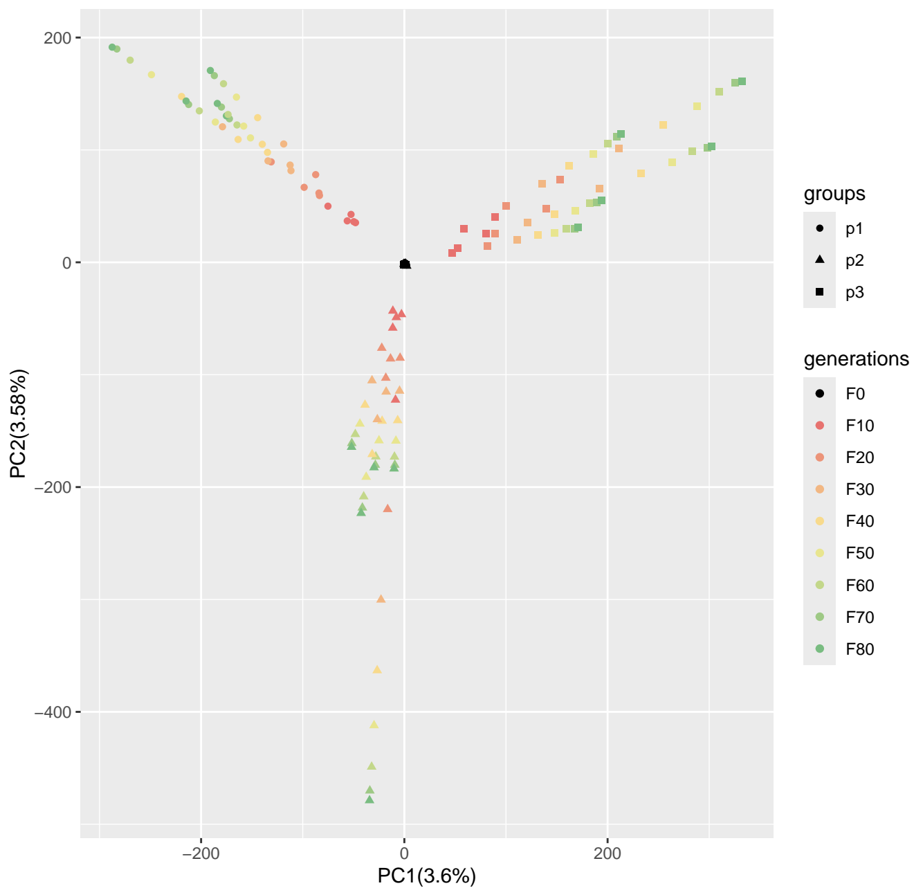
Run3_popsizel250_n400_20000loci_s50
