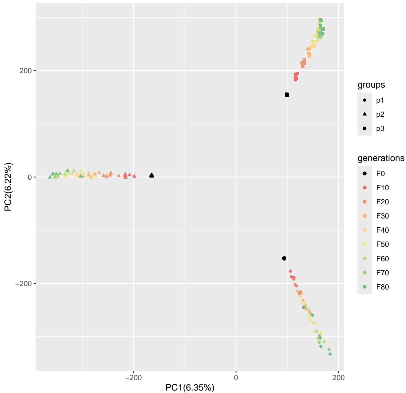
Run5_popsizel250_n400_20000loci_s50
