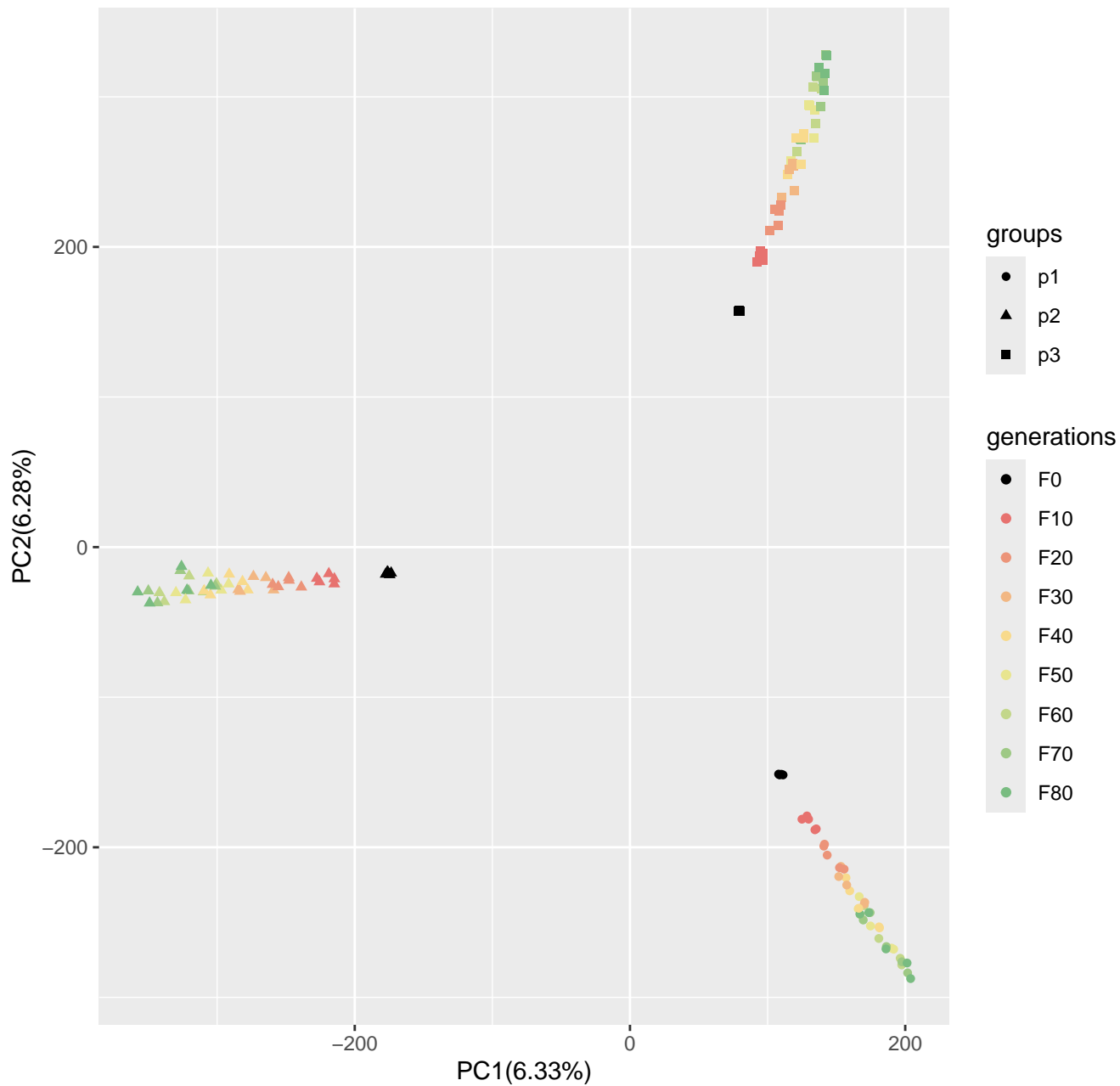
Run2_popsizel250_n400_1000loci_s10
