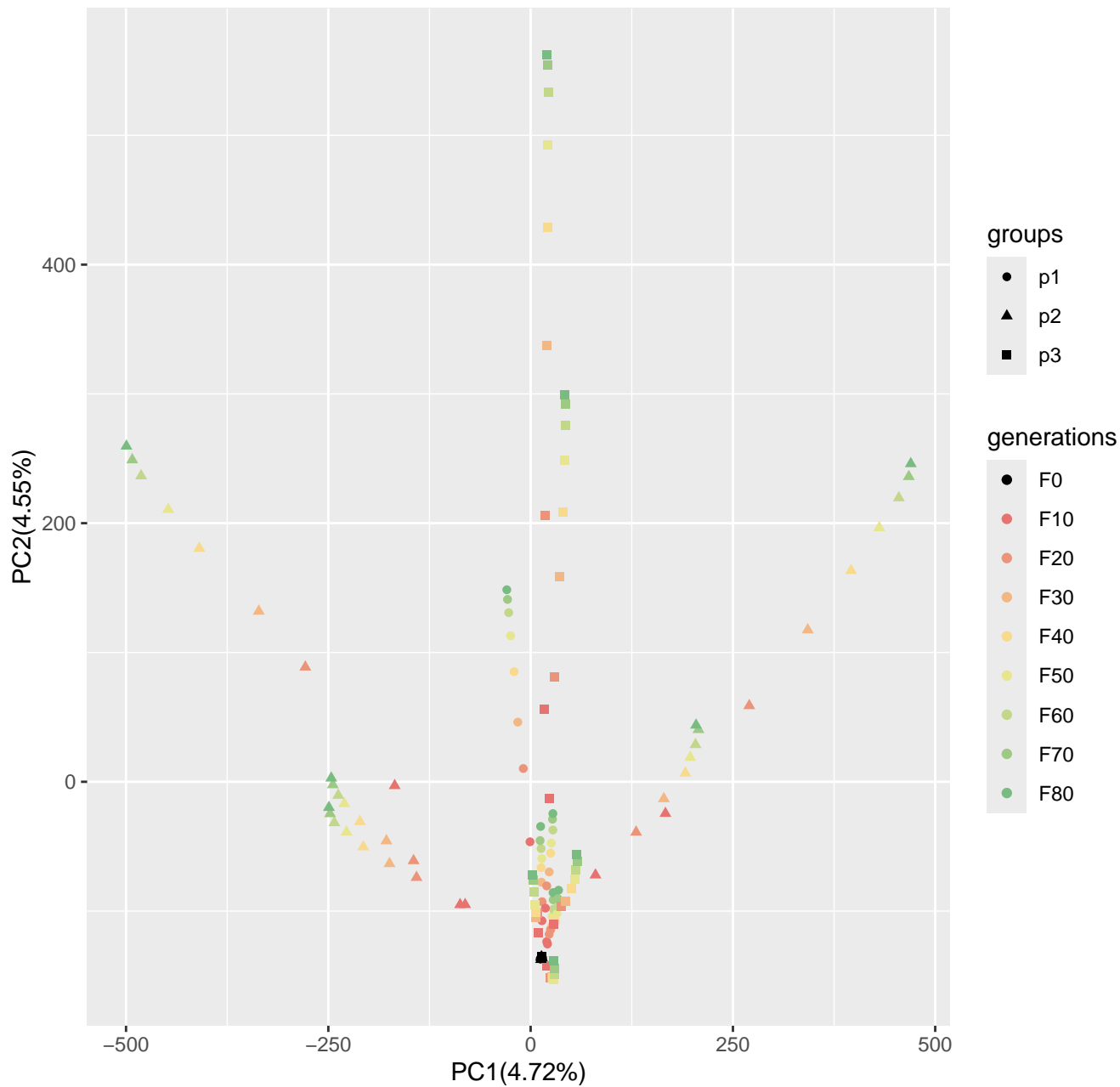
Run4_popsiz300_n400_10loci_s0
