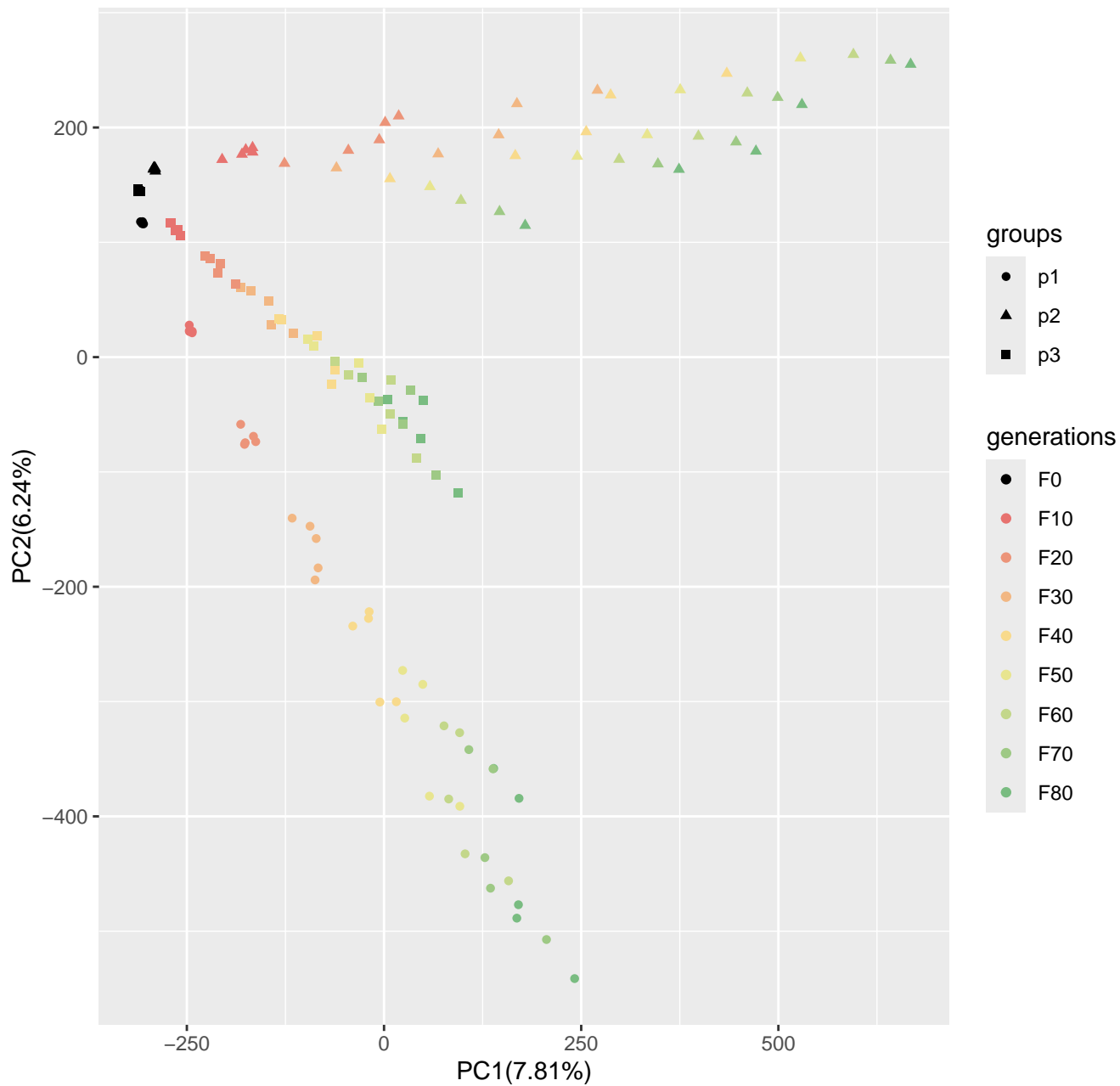
Run7_popsizel250_n1200_100loci_s10
