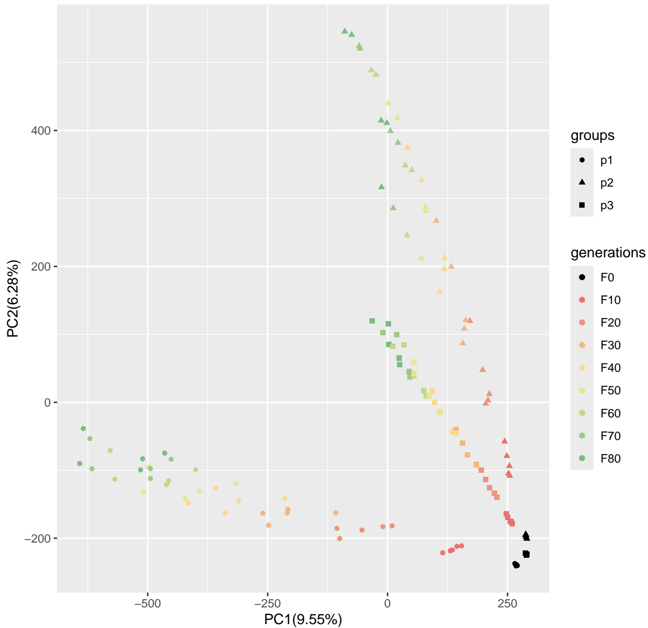
Run6_popsizel250_n1200_100loci_s10
