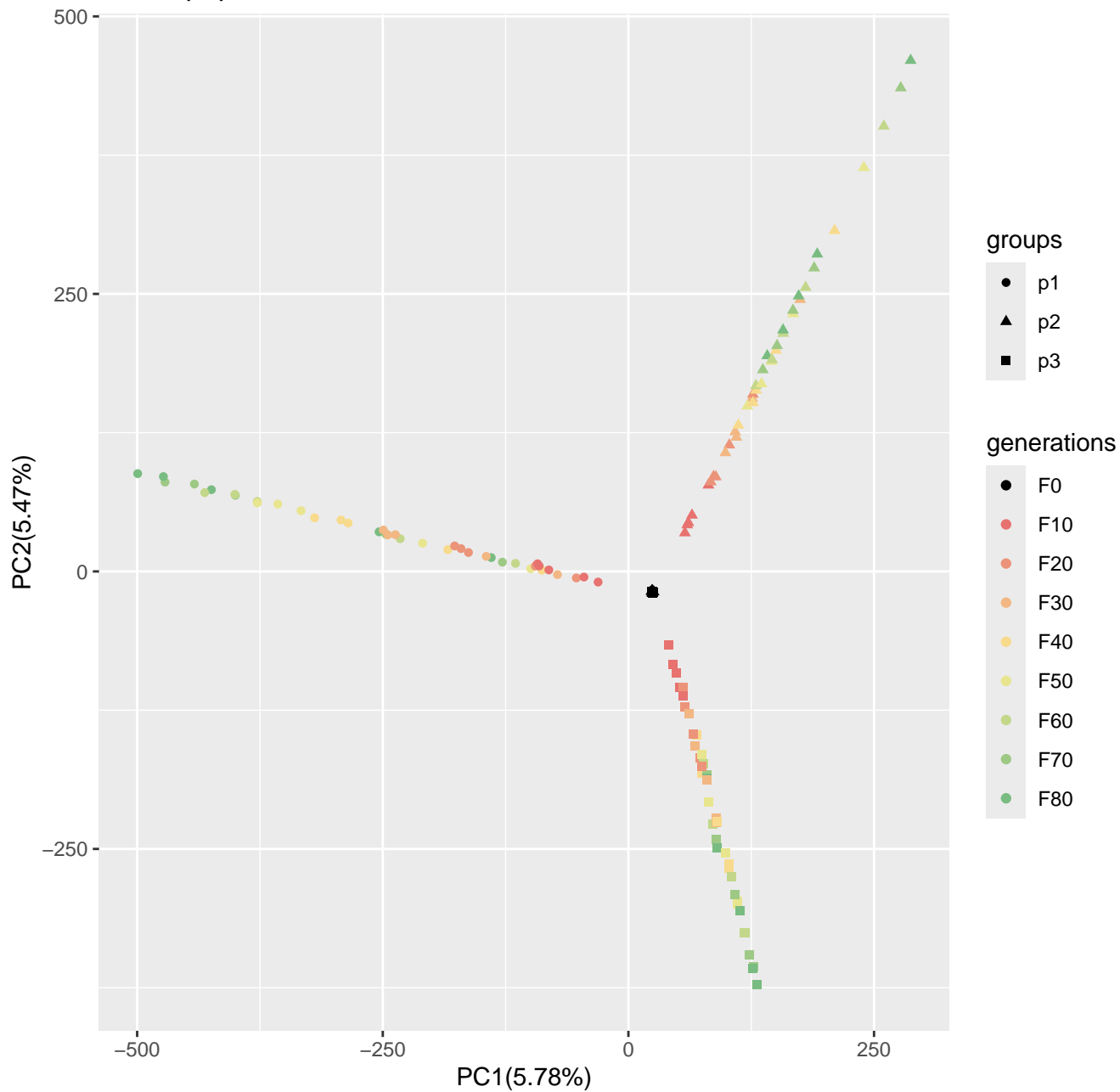
Run2_popsizel250_n400_10000loci_s50
