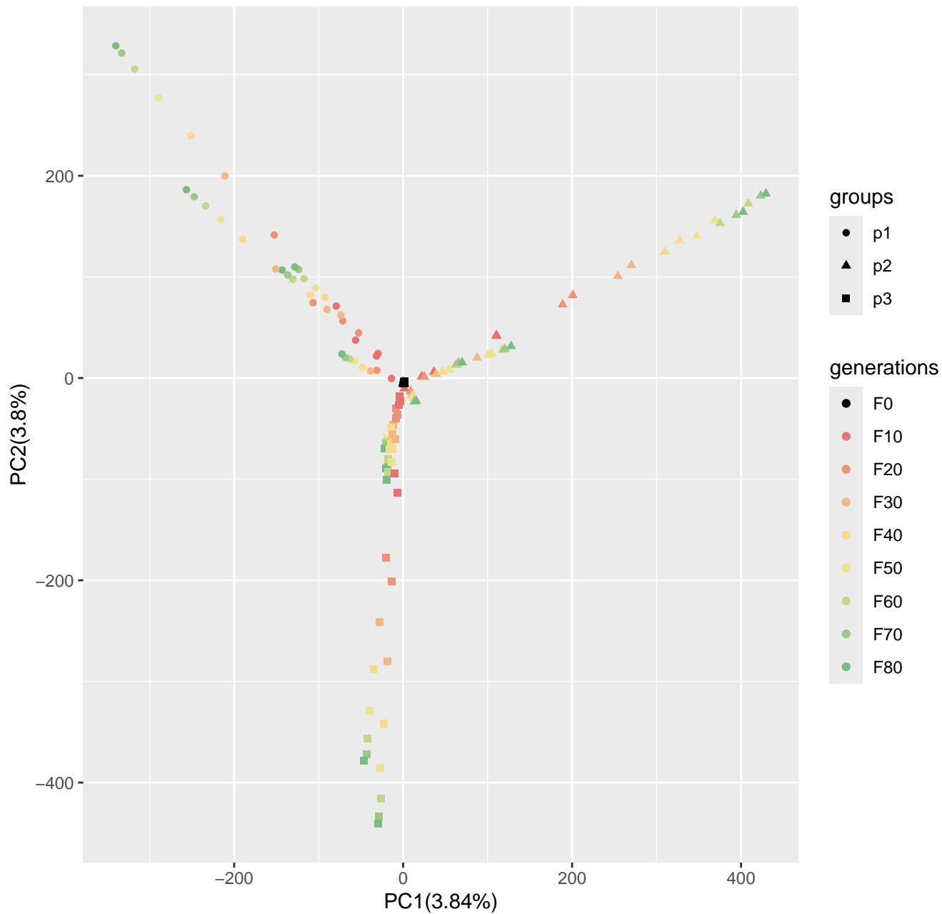
Run7_popsizel250_n400_5000loci_s10
