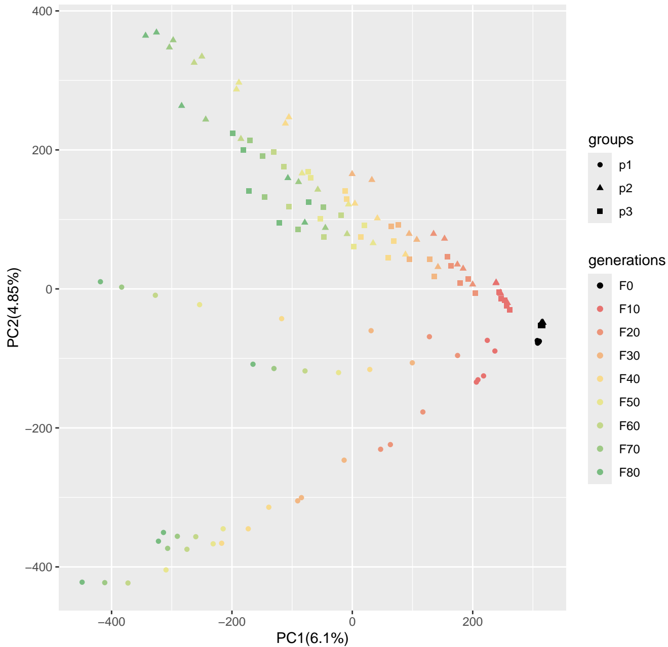
Run5_popsizel250_n2500_100loci_s10
