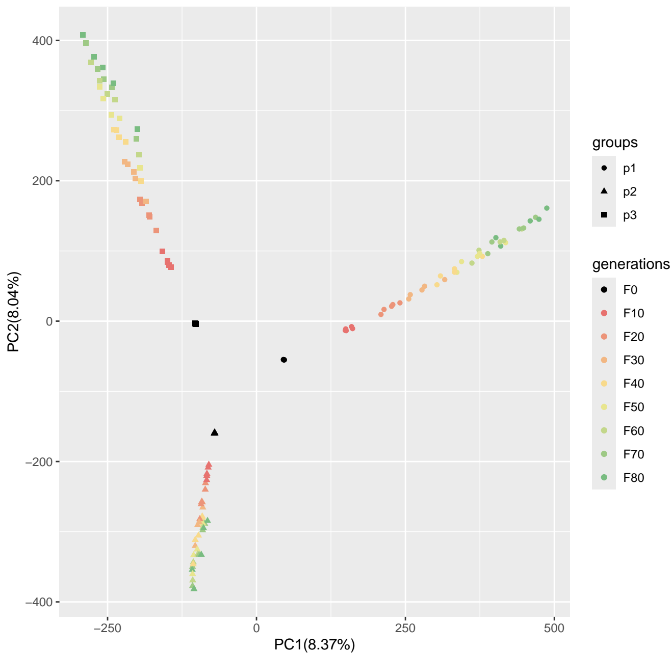
Run1_popsizel250_n400_10000loci_s100
