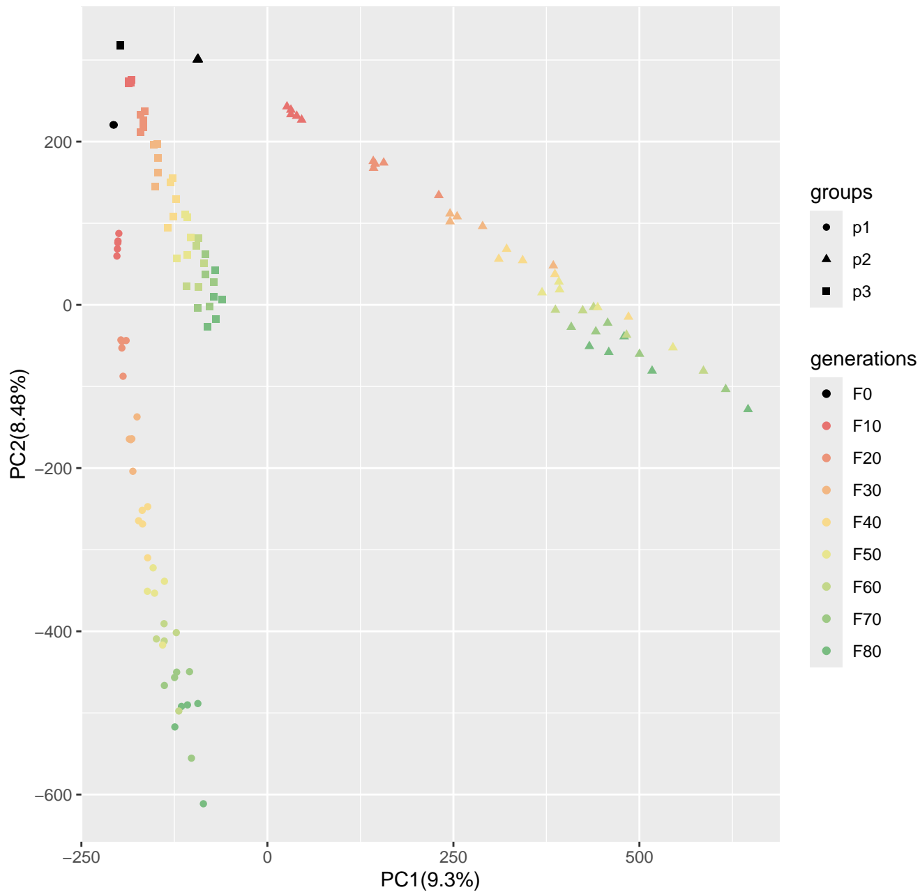
Run1_popsiz1250_n400_100loci_s10
