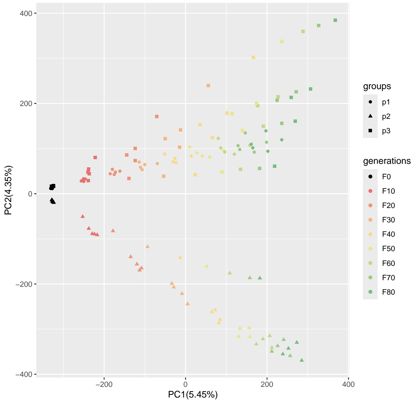
Run1_popsizel250_n2500_100loci_s10
