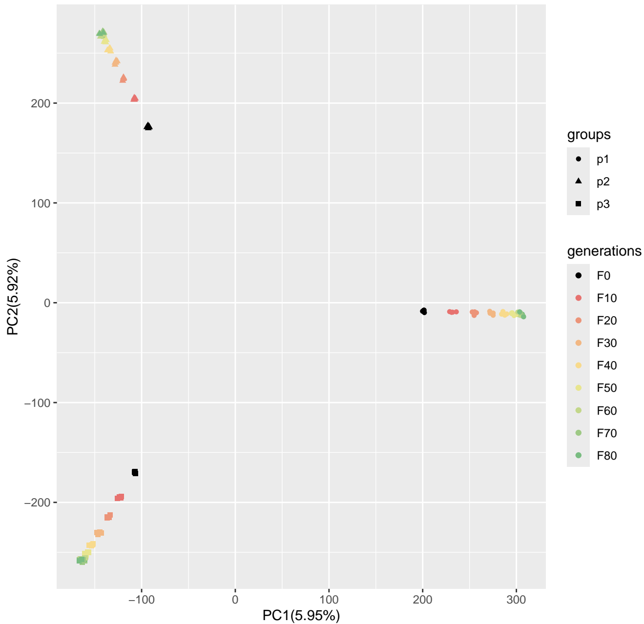
Run1_popsizel250_n400_1000loci_s10
