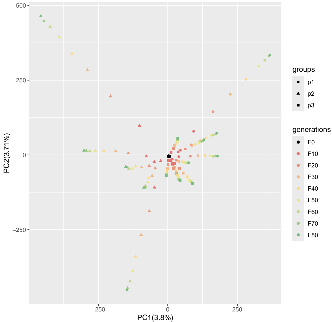
Run5_popsizel250_n400_5000loci_s10
