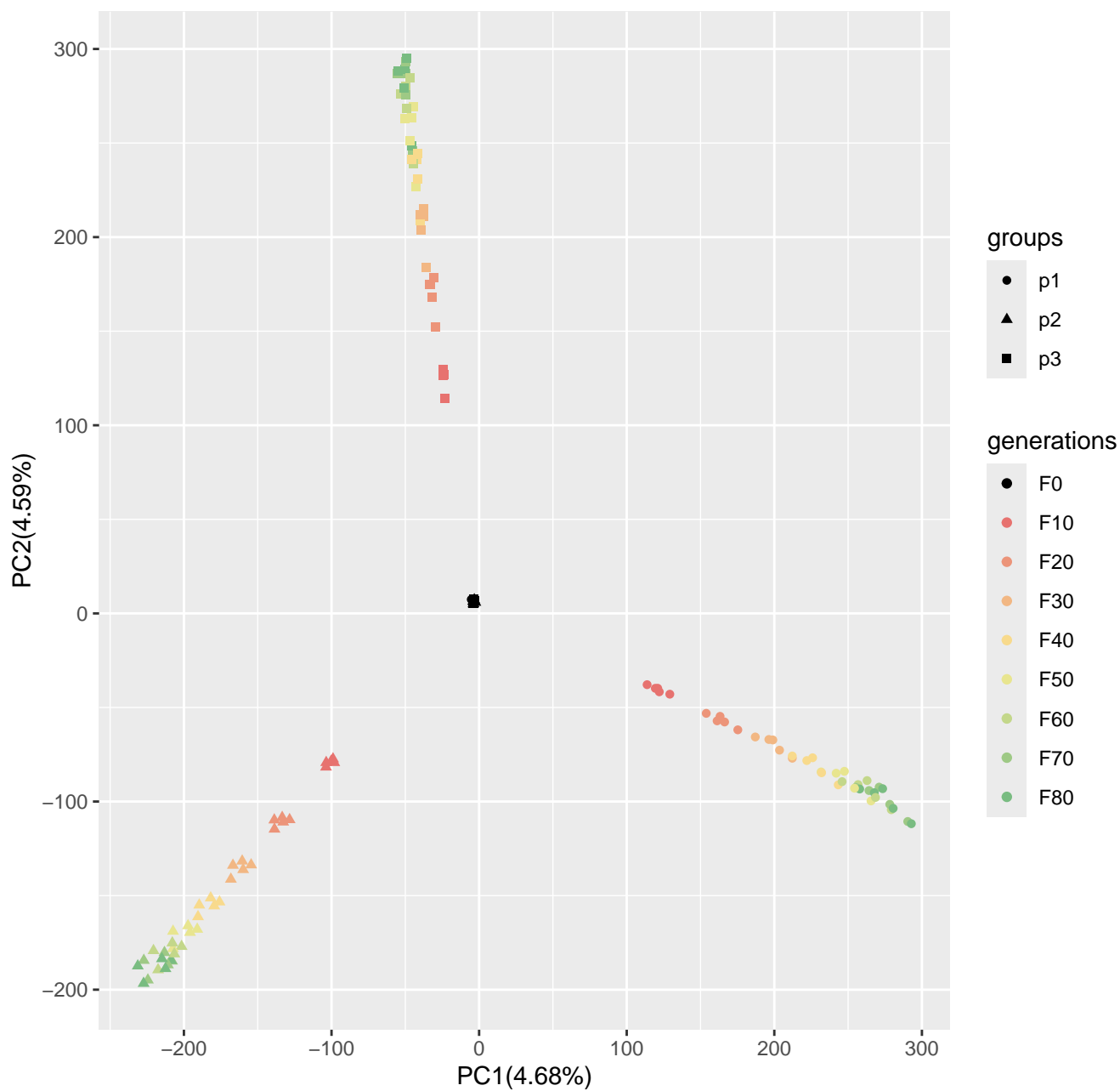
Run7_popsizel250_n400_5000loci_s100
