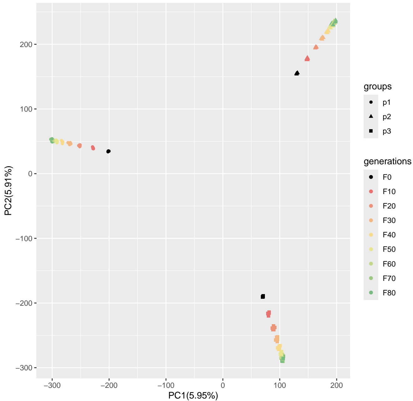
Run2_popsizel250_n400_10000loci_s10
