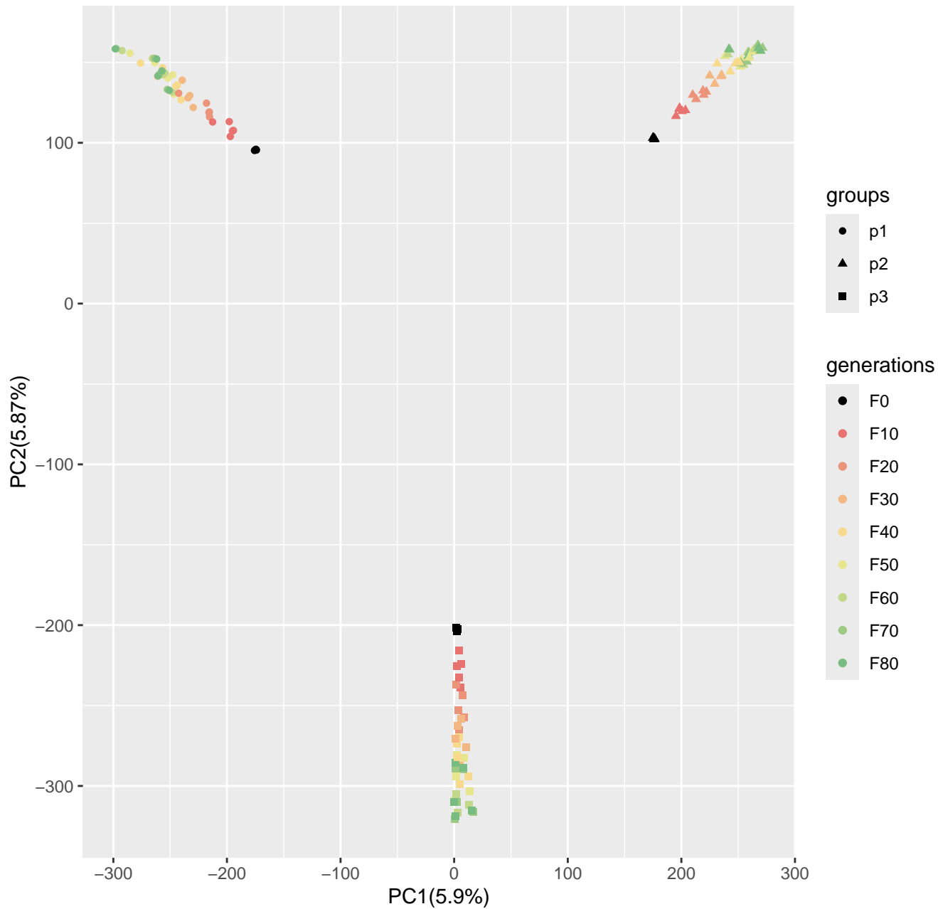
Run10_popsize1250_n400_20000loci_s10
