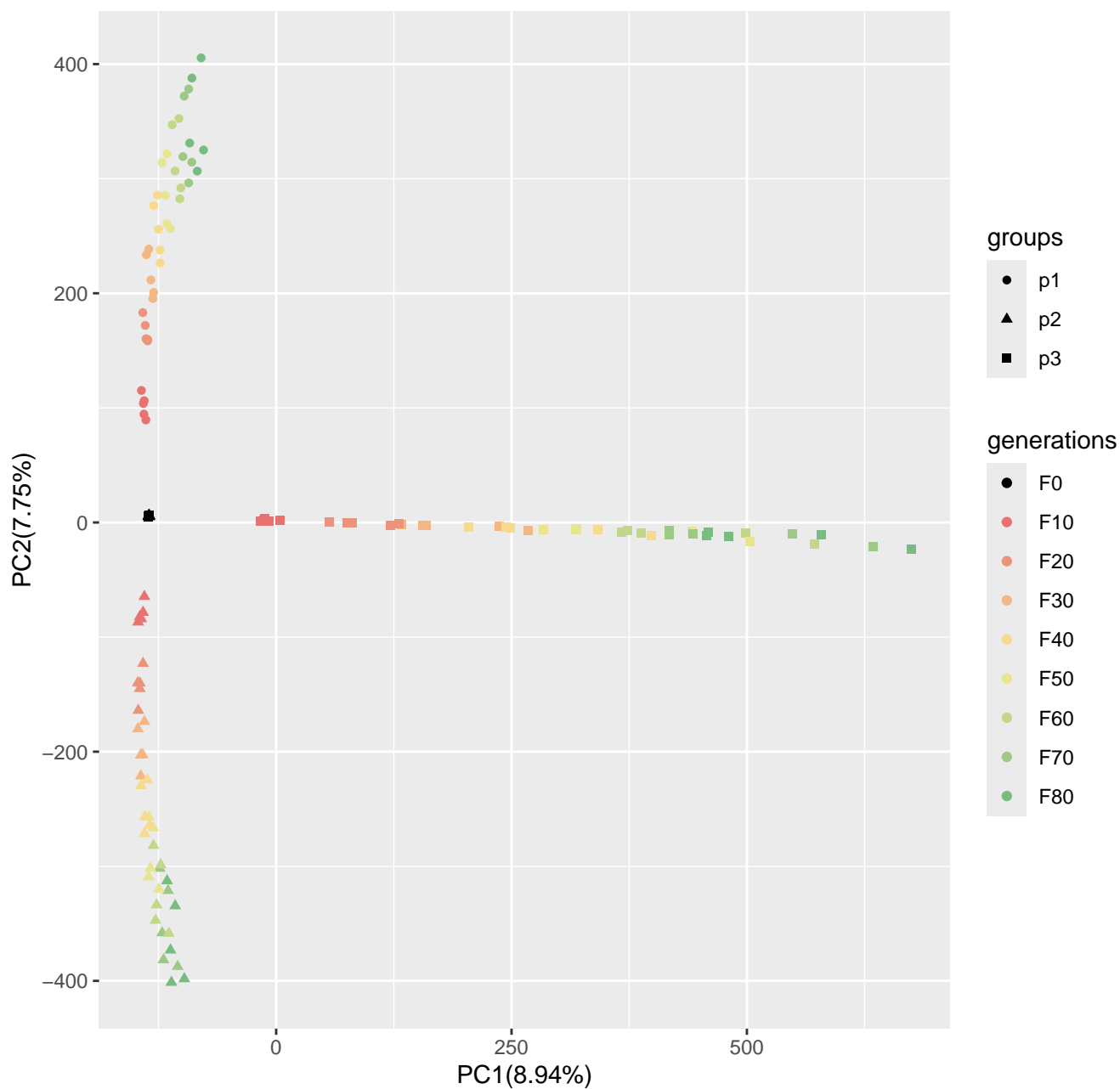
Run10_popsizel250_n400_10000loci_s100
