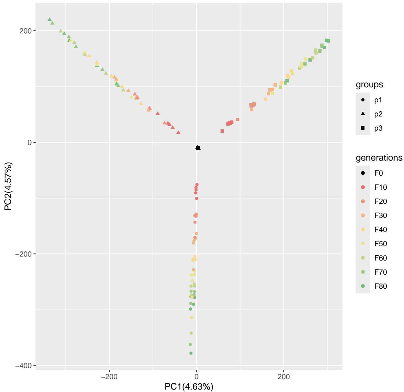
Run2_popsizel250_n400_20000loci_s50
