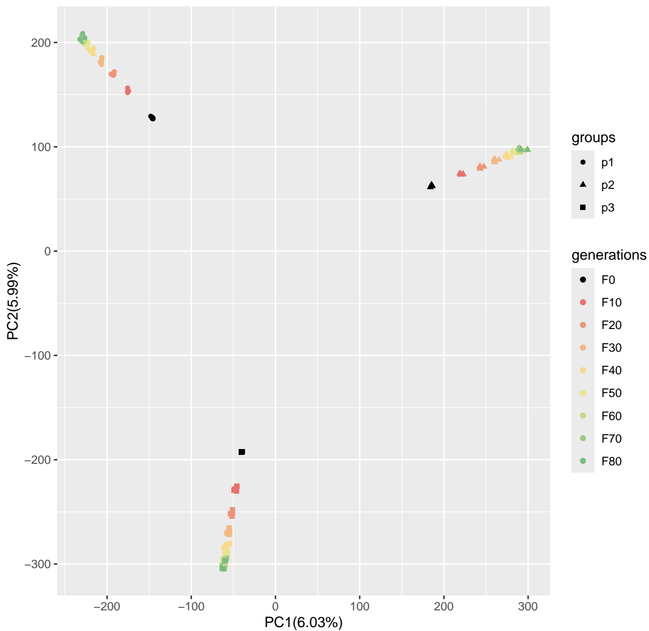
Run5_popsizel250_n400_20000loci_s100
