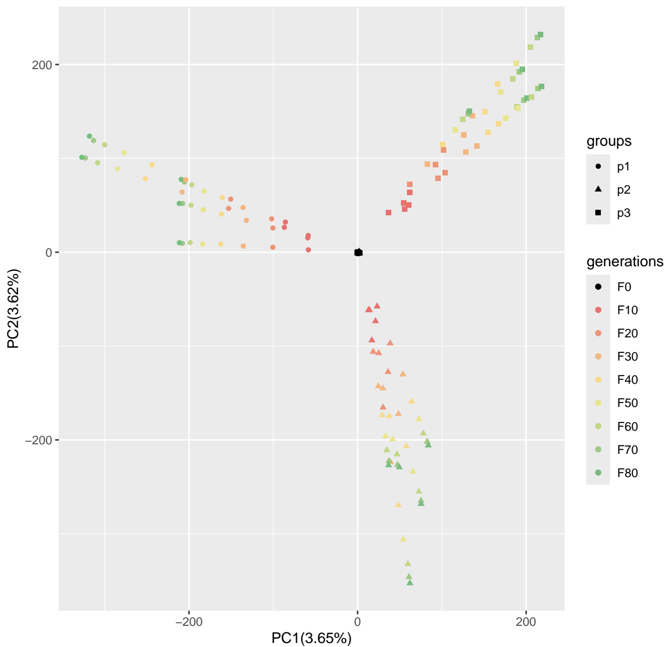
Run2_popsizel250_n400_10000loci_s50
