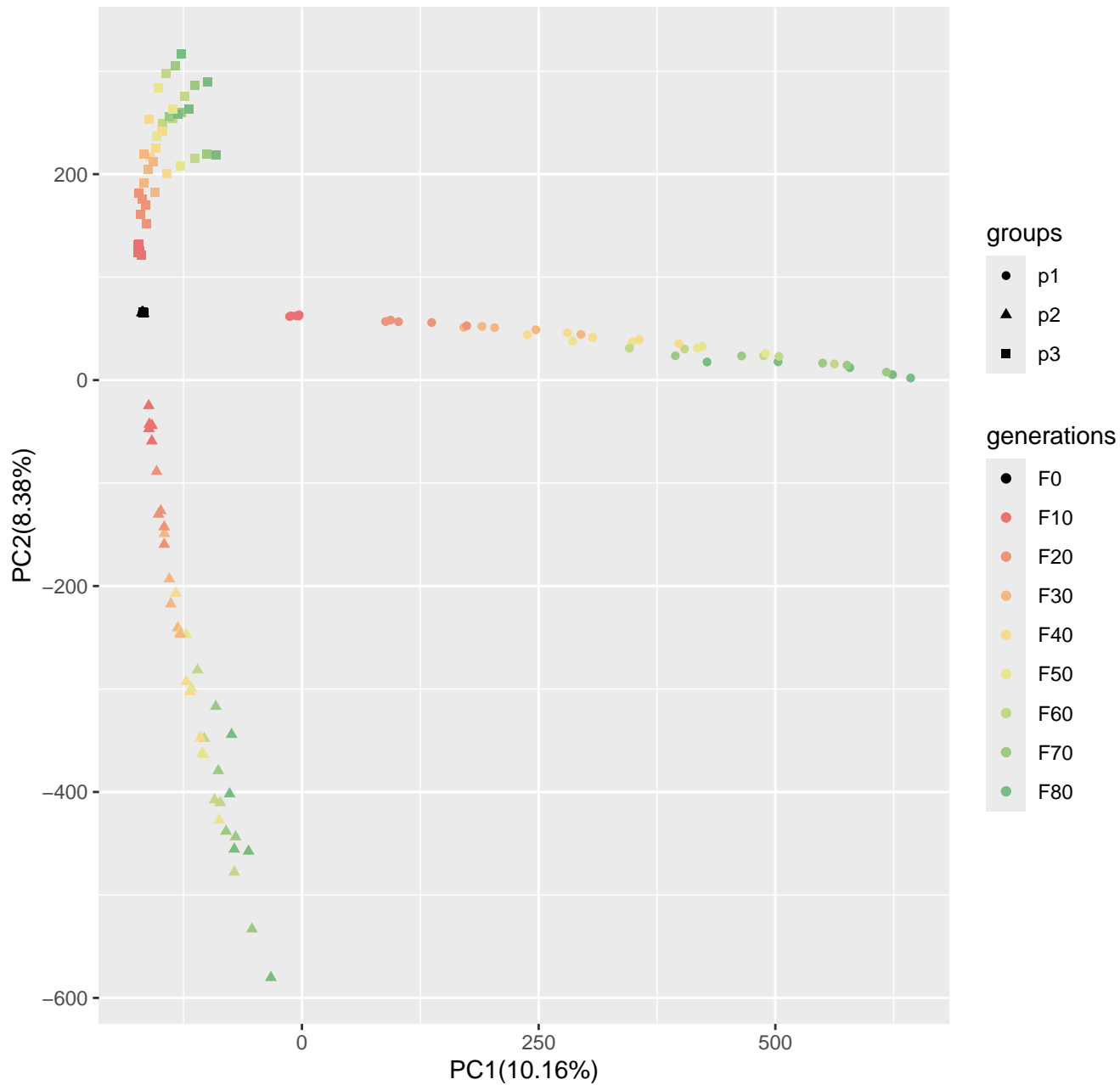
Run2_popsizel250_n400_10000loci_s100
