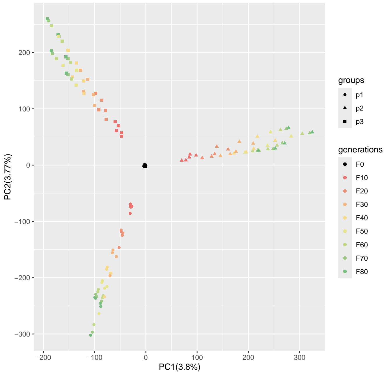
Run2_popsizel250_n400_20000loci_s100
