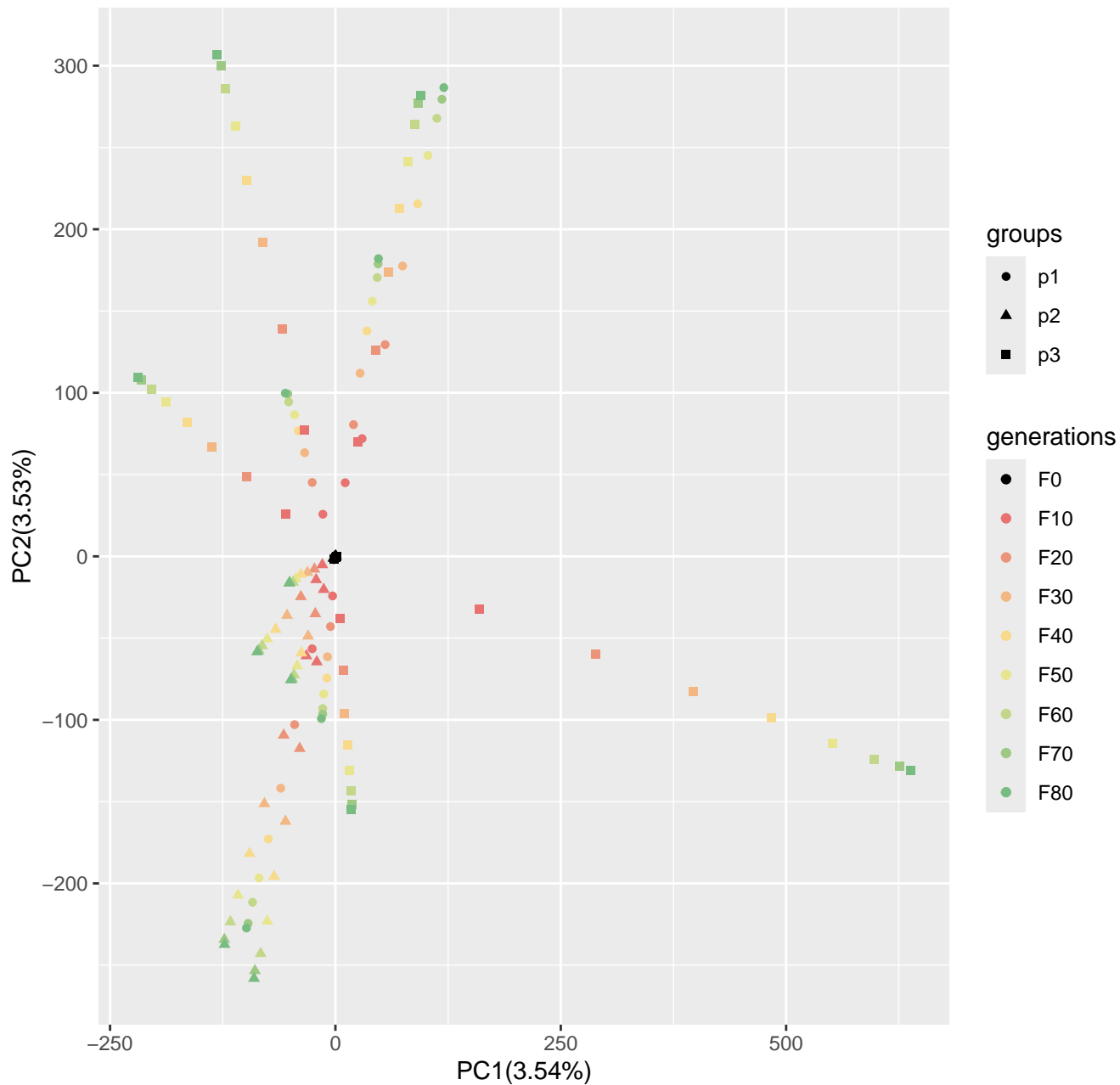
Run10_popsiz1250_n400_10000loci_s10
