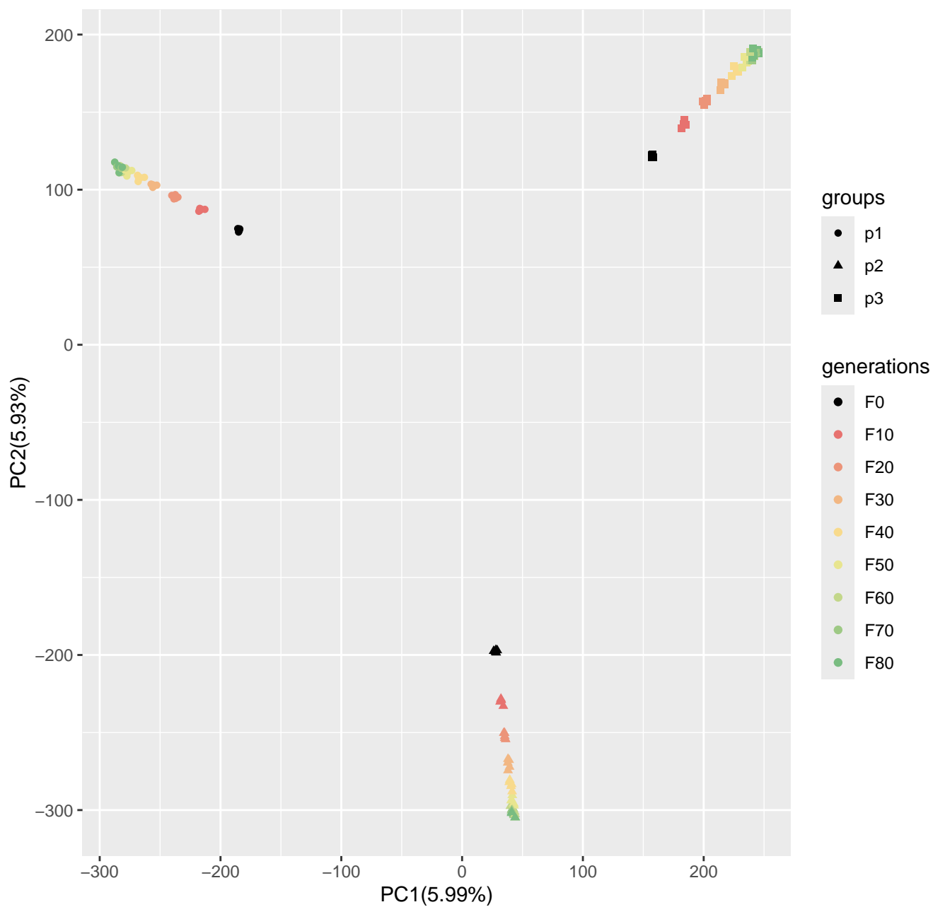
Run1_popsizel250_n400_10000loci_s50
