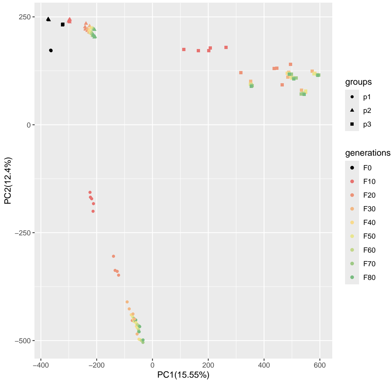
Run1_popsizel250_n400_10loci_s10
