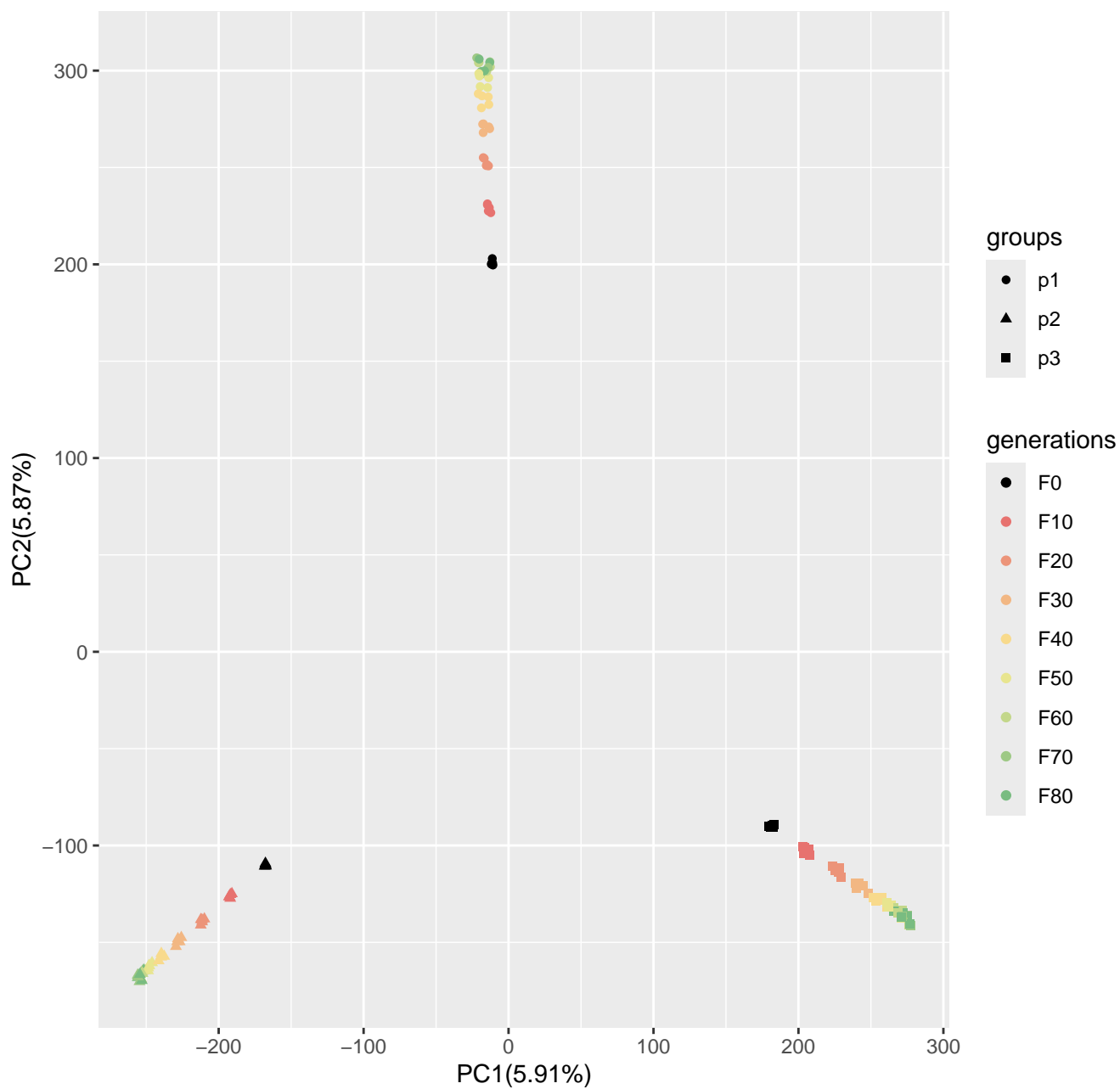
Run8_popsizel250_n400_5000loci_s10
