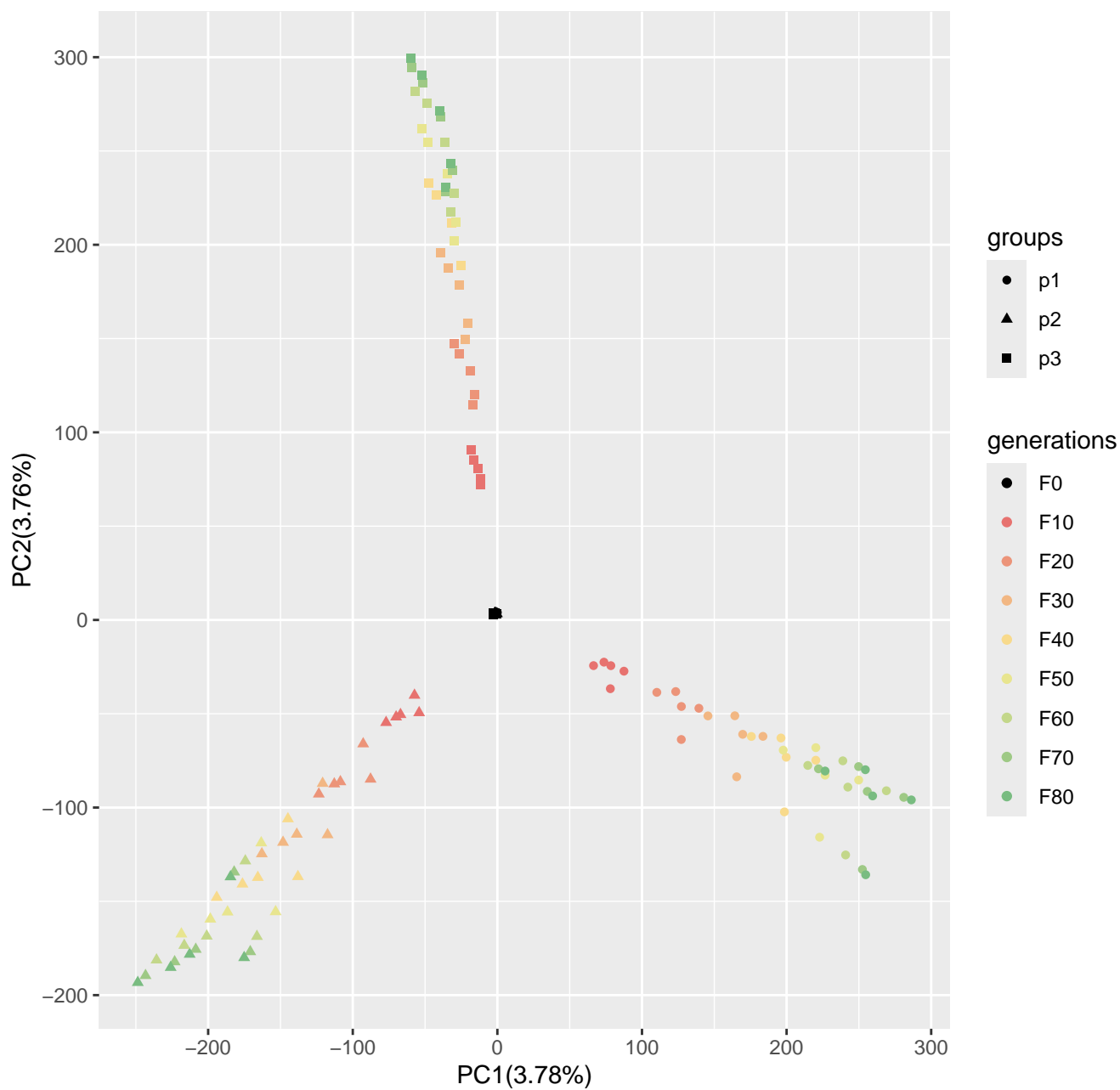
Run7_popsizel250_n400_5000loci_s50
