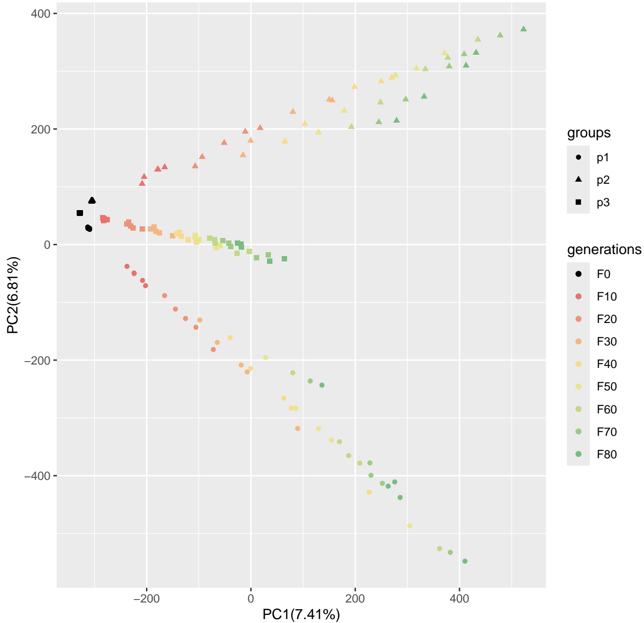
Run2_popsizel250_n1200_100loci_s10
