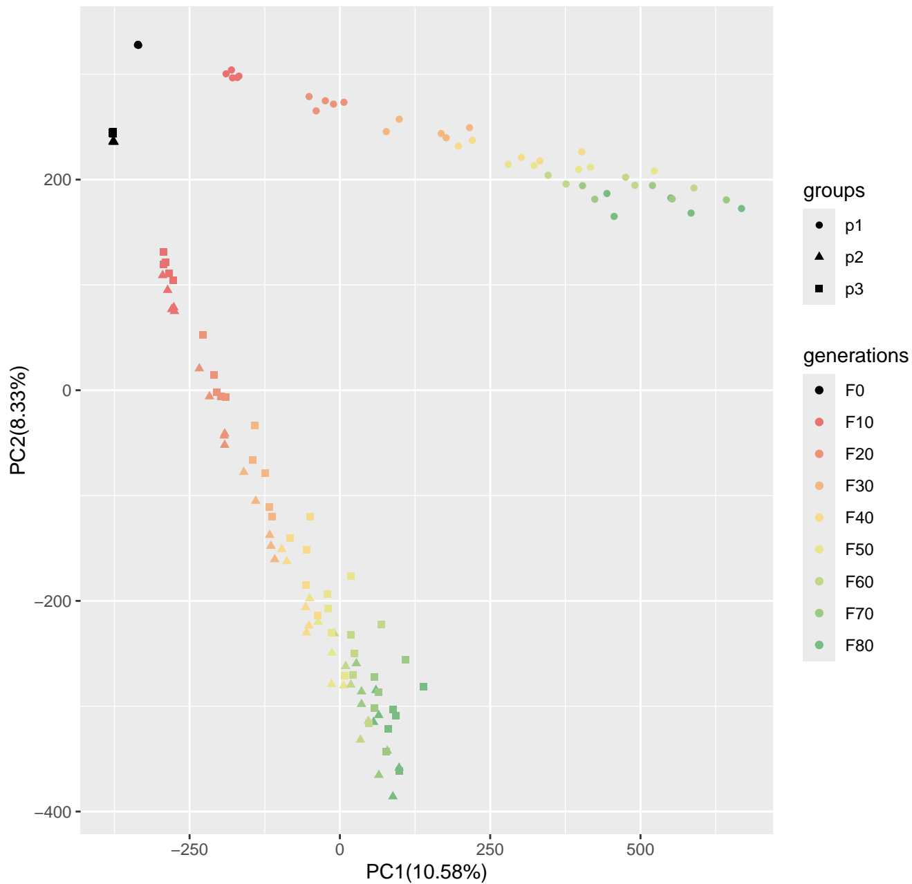
Run3_popsiz1250_n400_5000loci_s100
