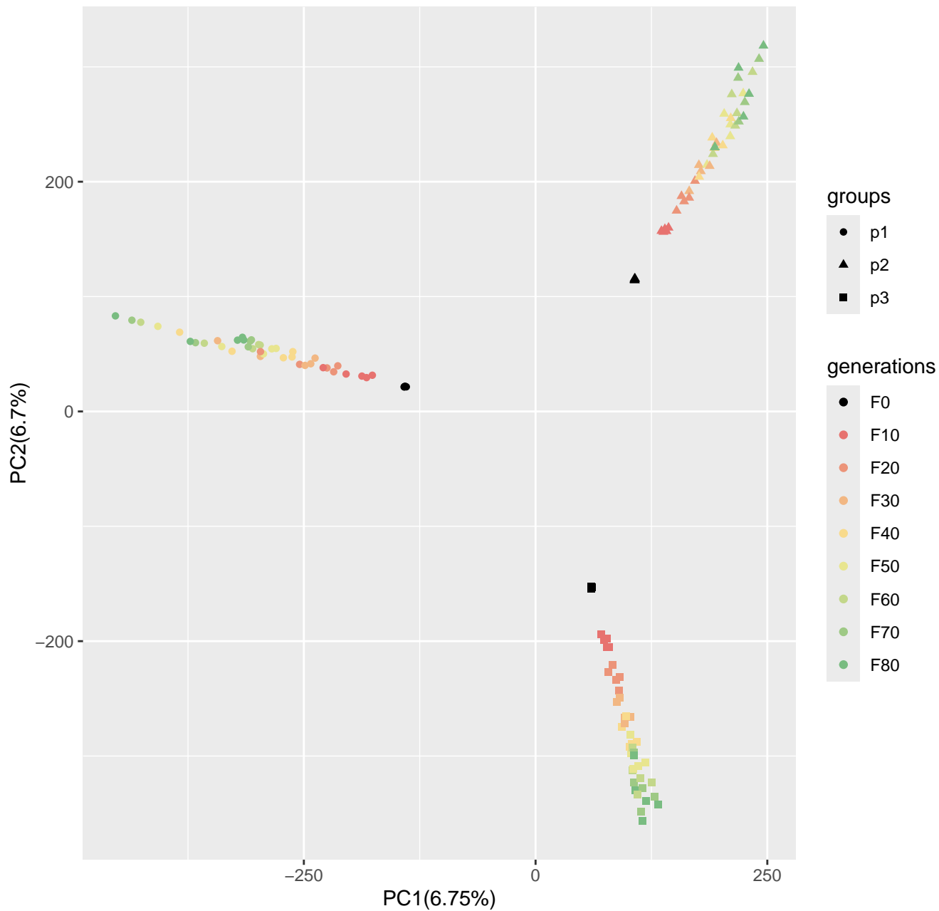
Run7_popsizel250_n400_10000loci_s50
