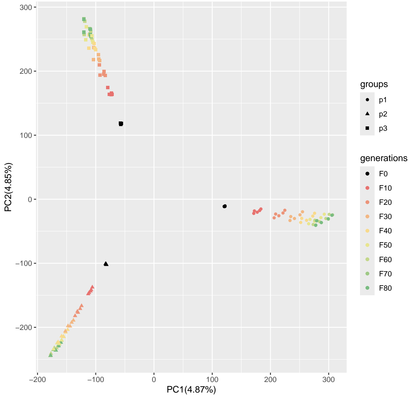
Run3_popsiz300_n400_10loci_s0
