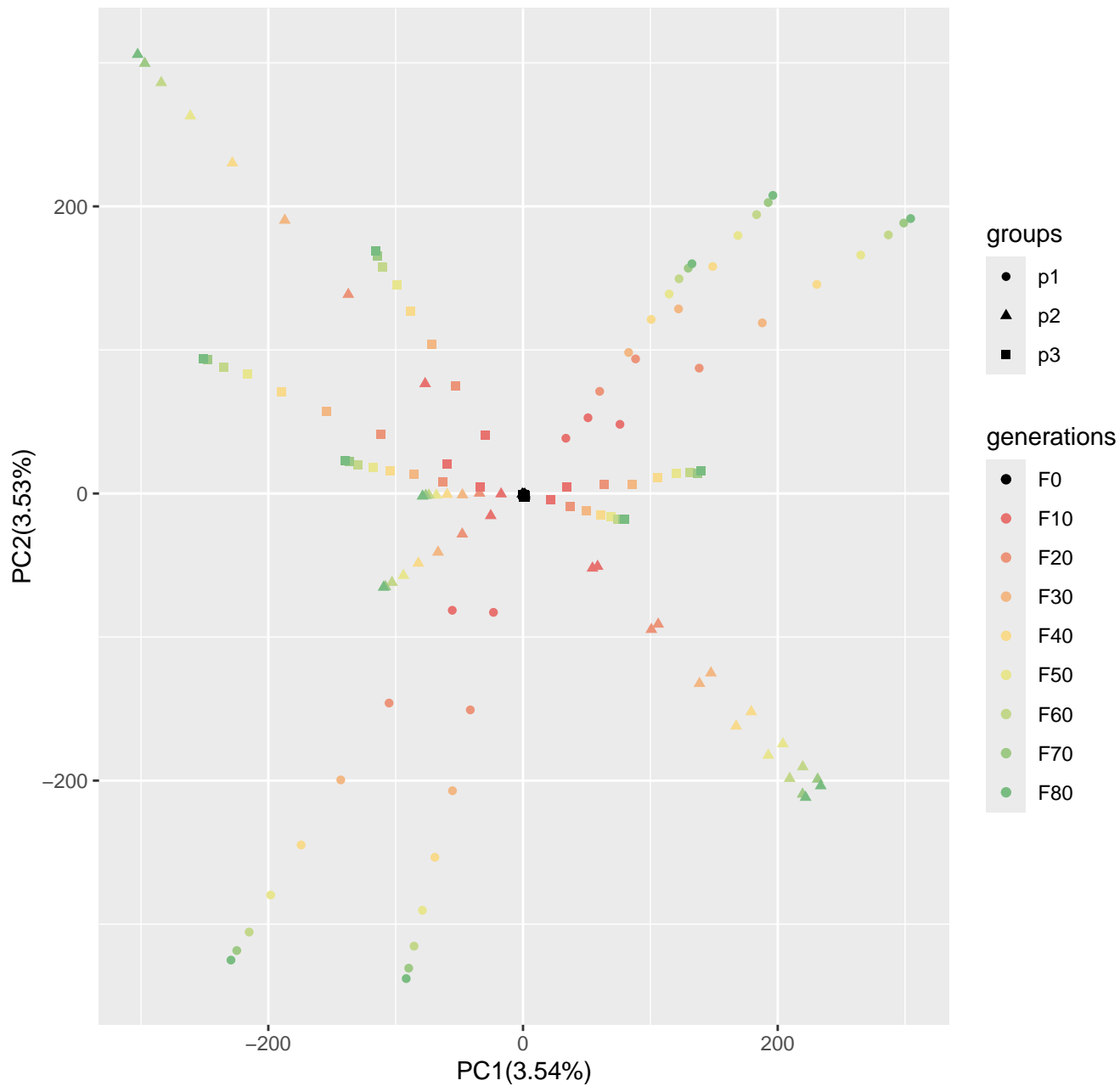
Run8_popsiz1250_n400_10loci_s0
