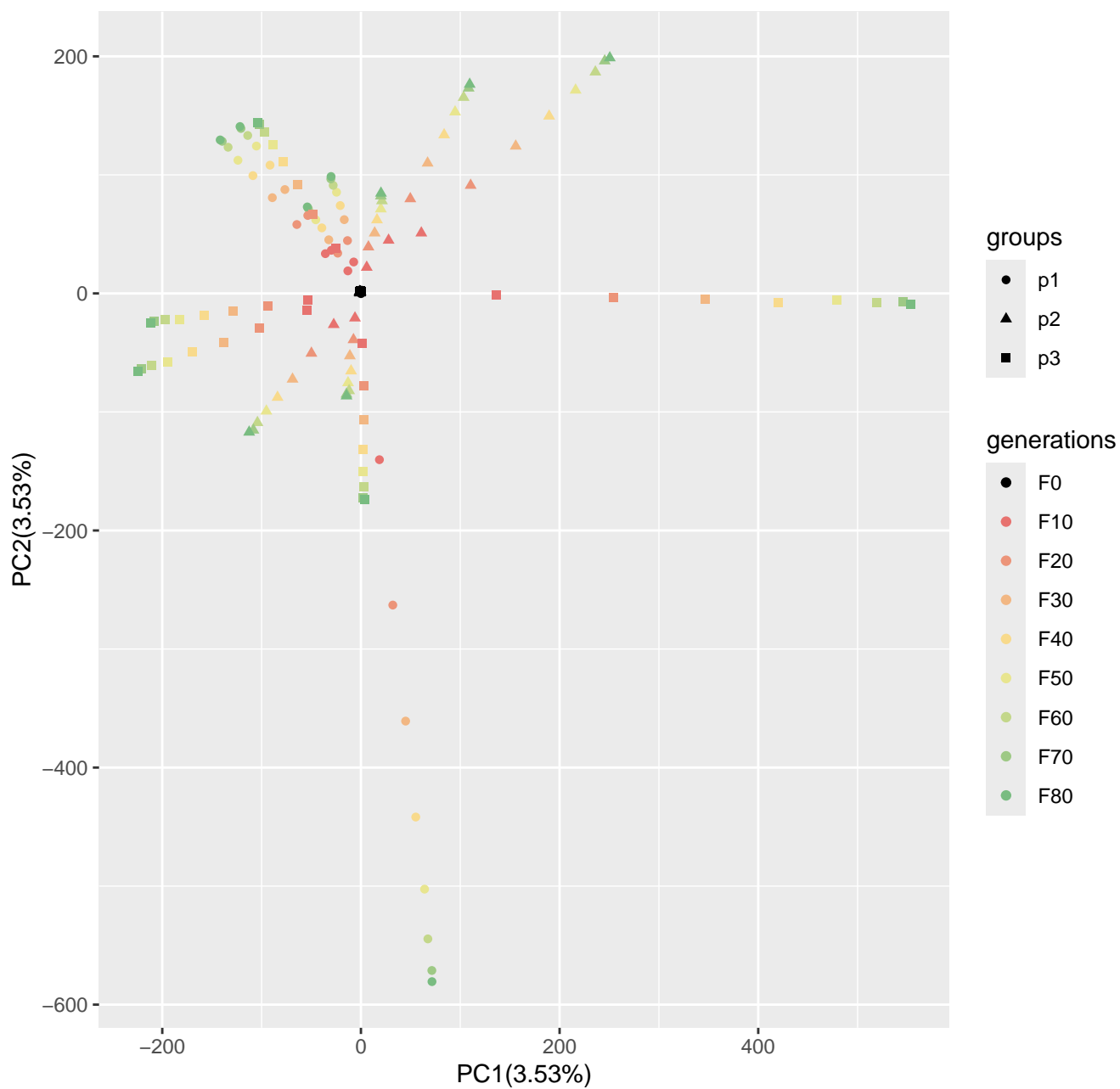
Run7_popsizel250_n400_10000loci_s10
