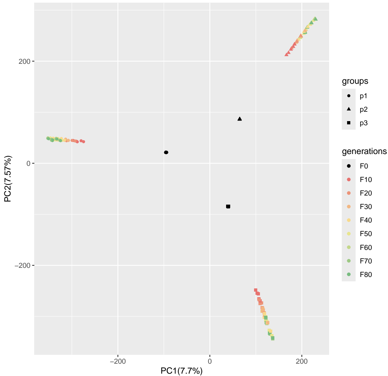
Run5_popsizel250_n400_1000loci_s100
