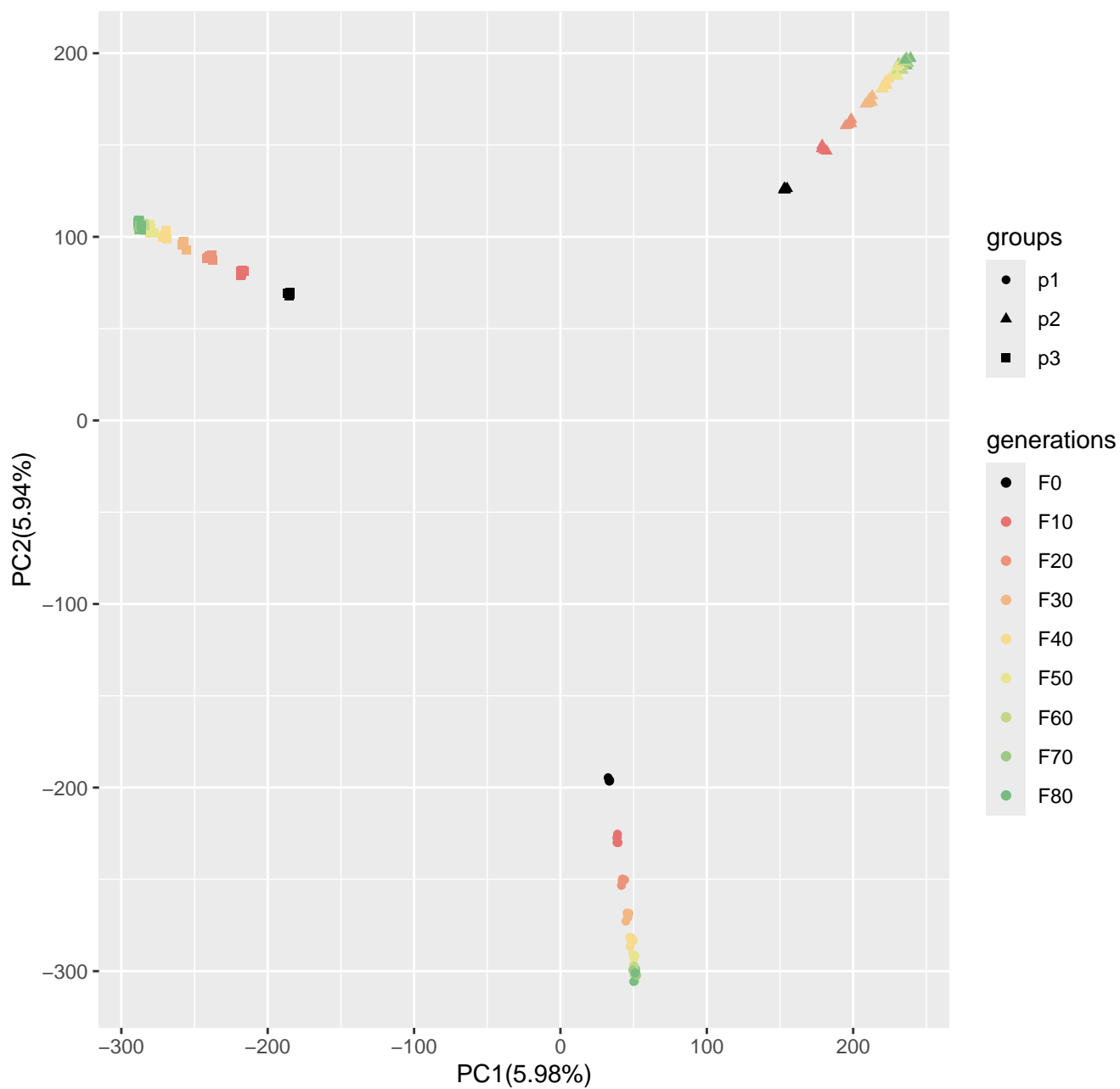
Run8_popsizel250_n400_10000loci_s50
