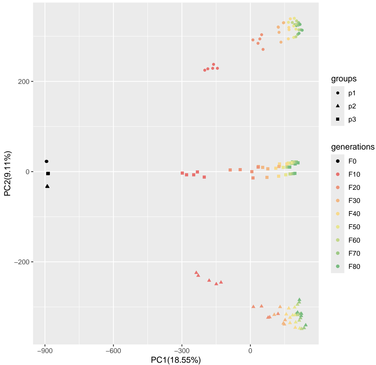
Run4_popsizel250_n400_1000loci_s100
