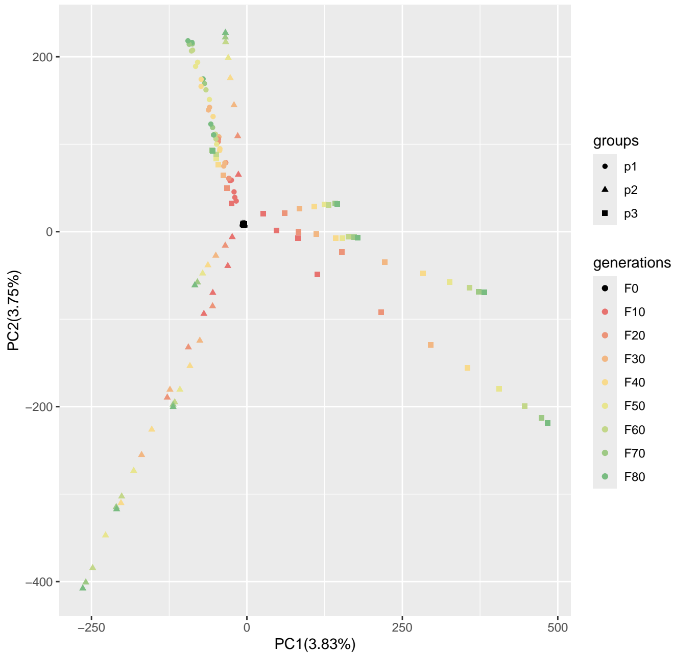
Run10_popsiz1250_n400_5000loci_s10
