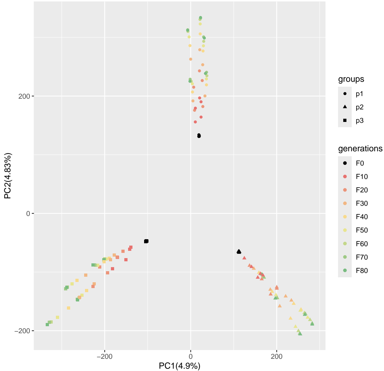
Run6_popsiz300_n400_10loci_s0
