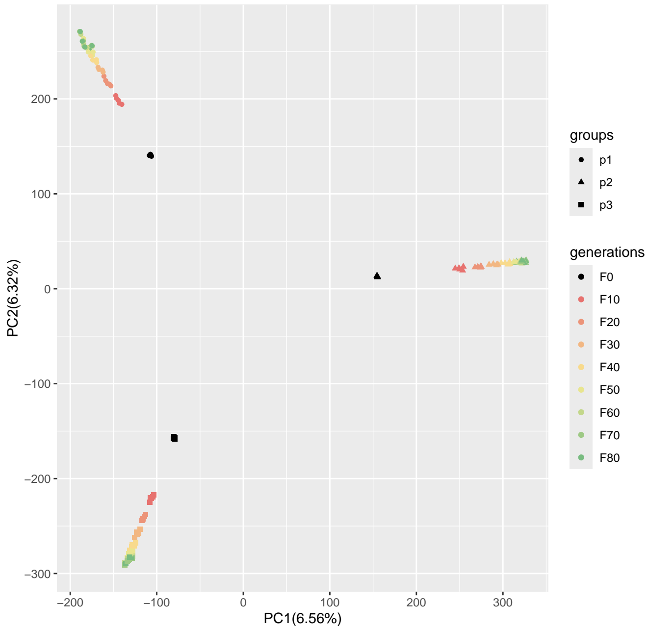
Run1_popsizel250_n400_1000loci_s50
