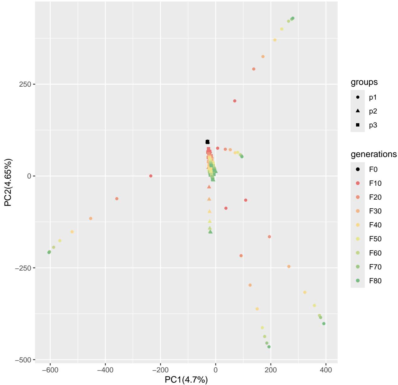
Run2_popsiz300_n400_10loci_s0
