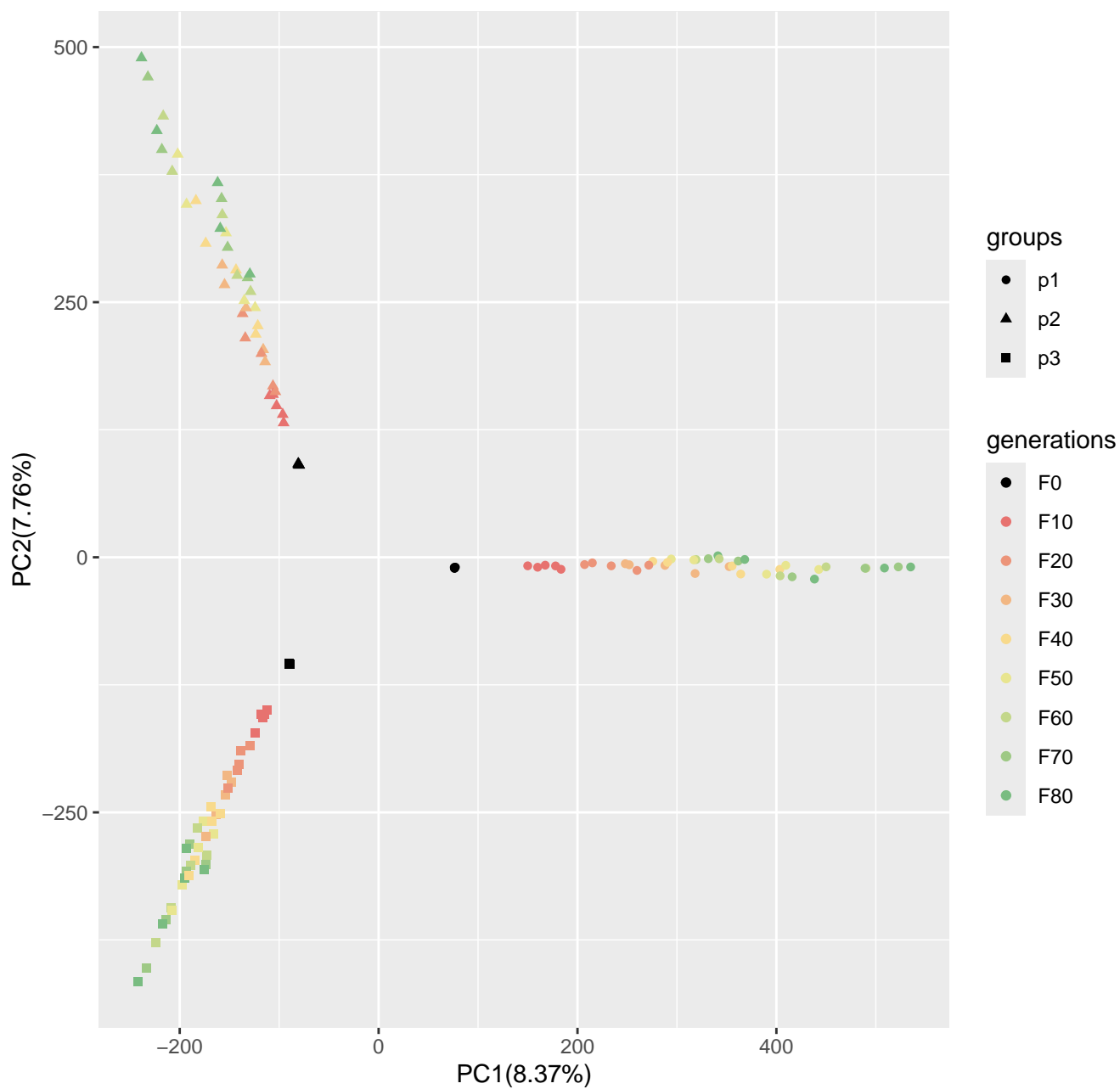
Run1_popsizel250_n400_5000loci_s50
