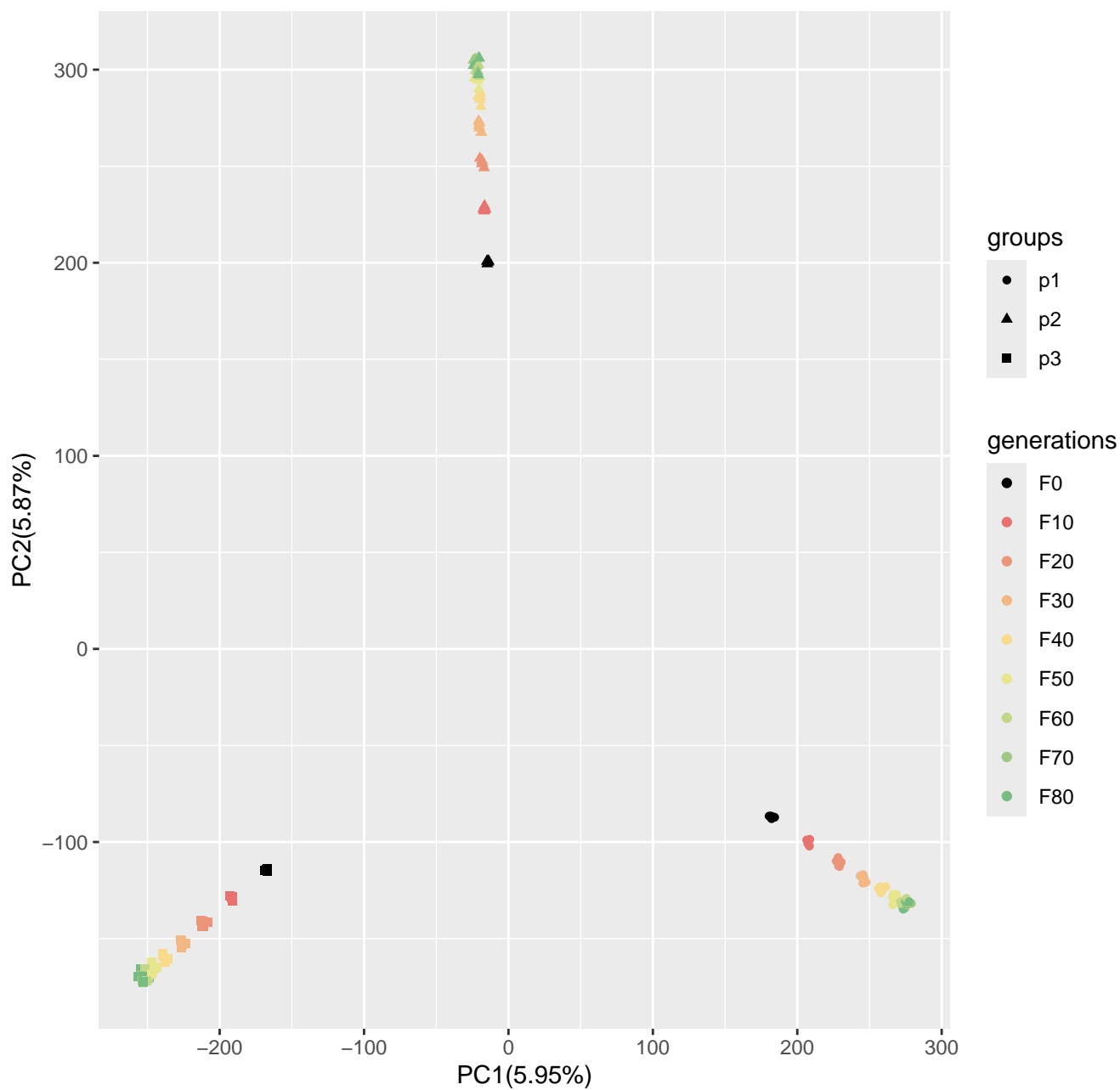
Run1_popsizel250_n400_5000loci_s10
