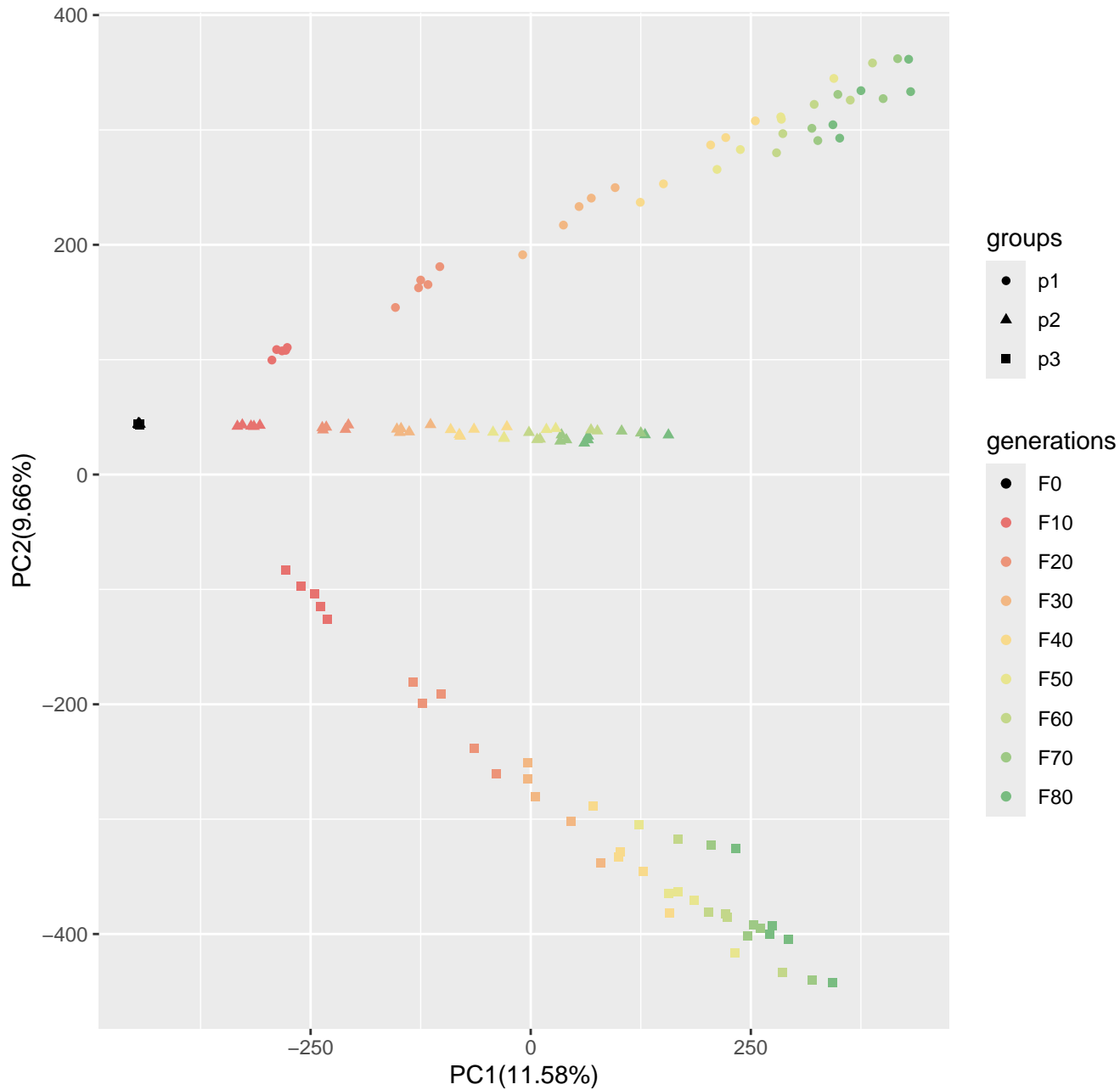
Run8_popsiz1250_n400_1000loci_s50
