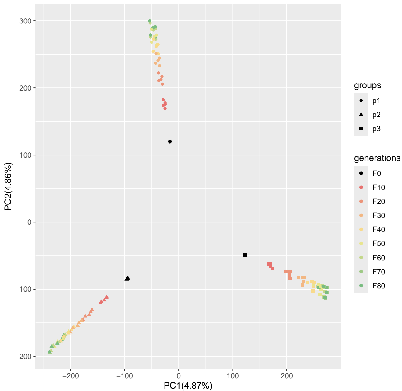
Run2_popsiz300_n400_10loci_s0
