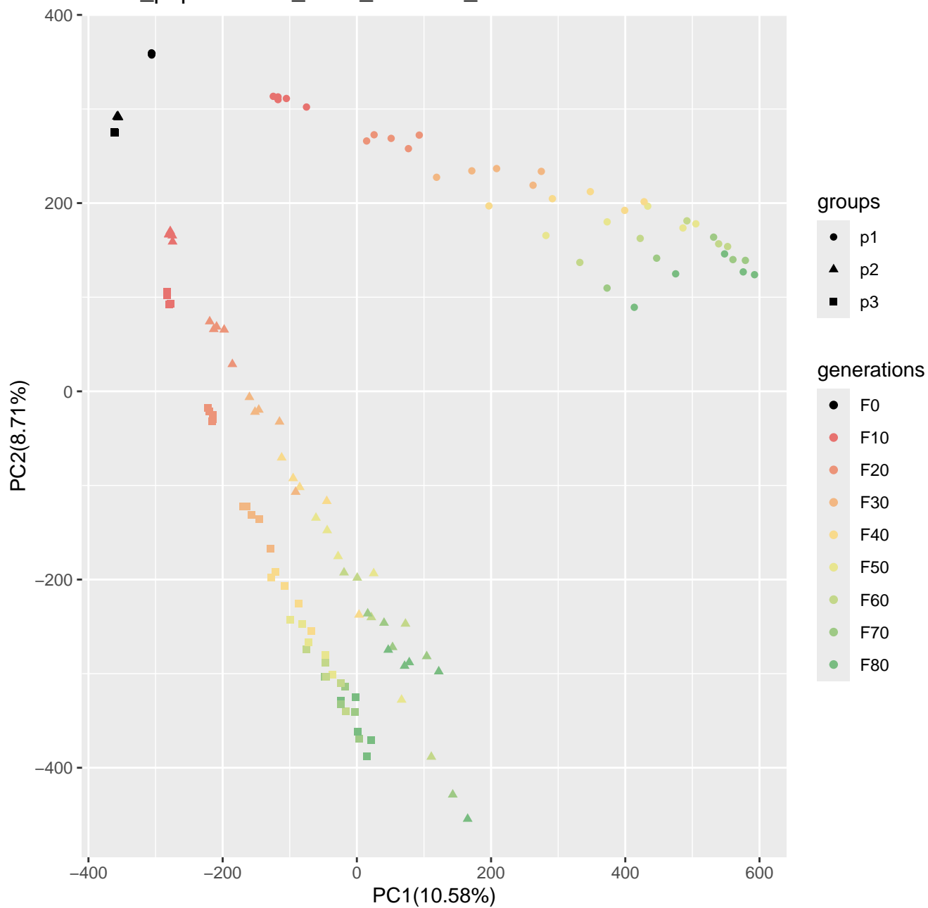
Run6_popsiz1250_n400_5000loci_s100
