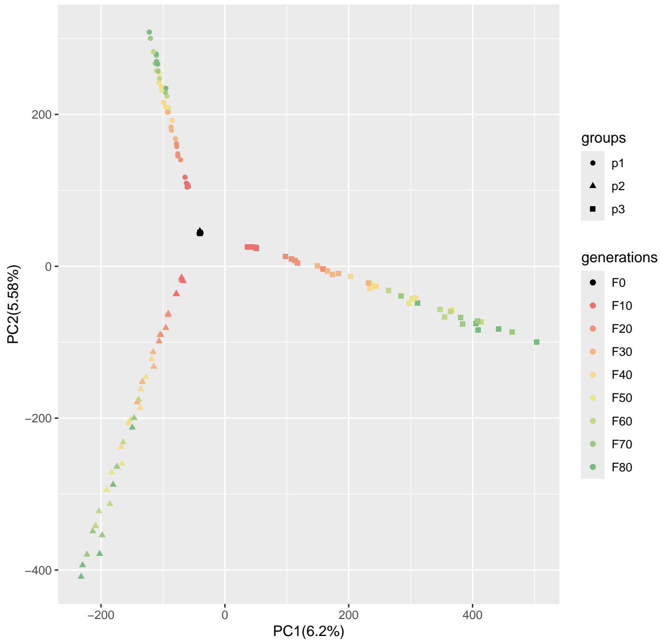
Run8_popsizel250_n400_10000loci_s50
