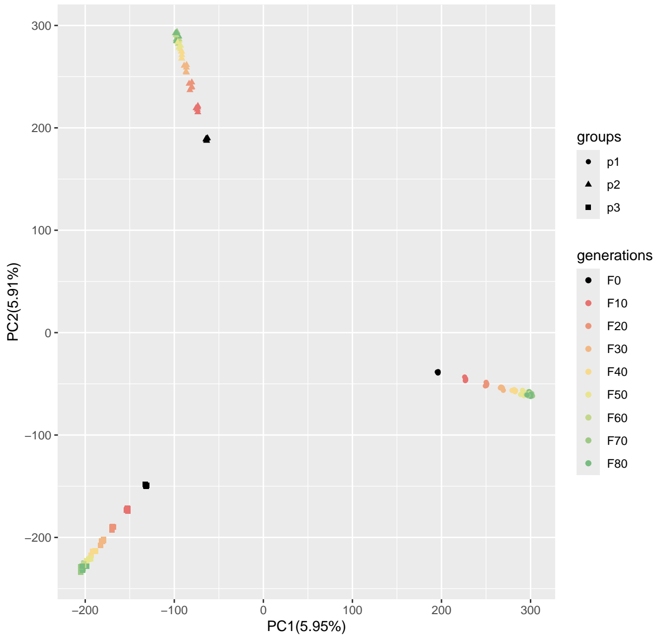
Run3_popsizel250_n400_20000loci_s50
