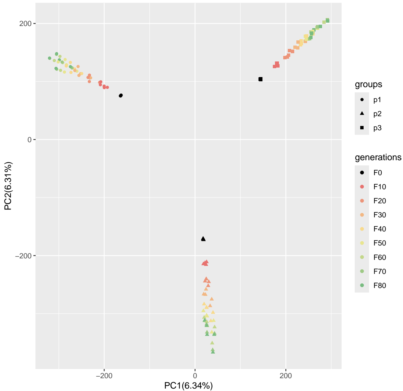
Run4_popsizel250_n400_20000loci_s50
