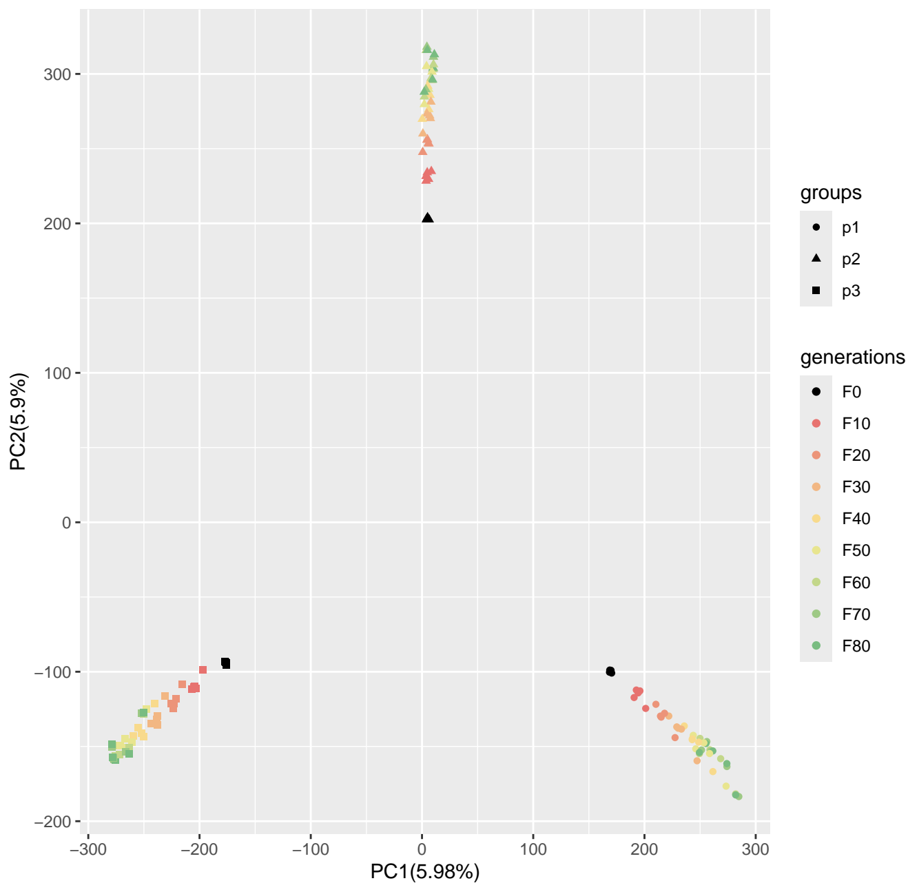
Run1_popsizel250_n400_20000loci_s10
