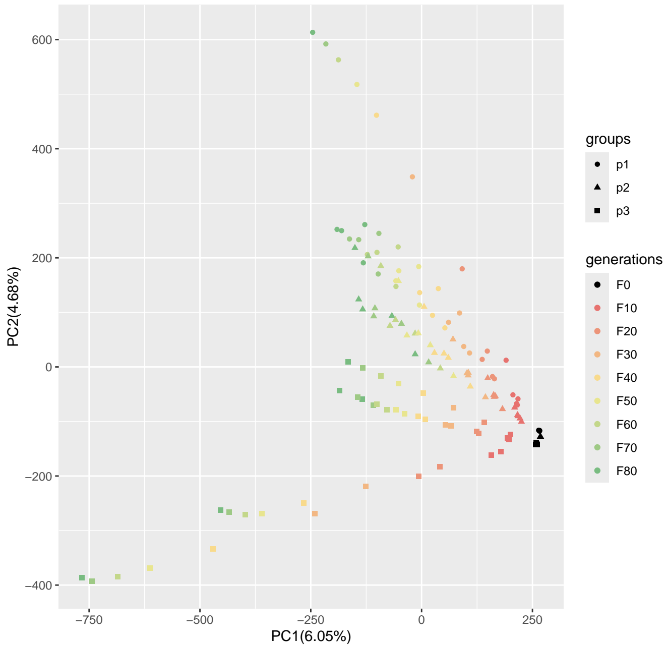
Run9_popsizel250_n2500_100loci_s10
