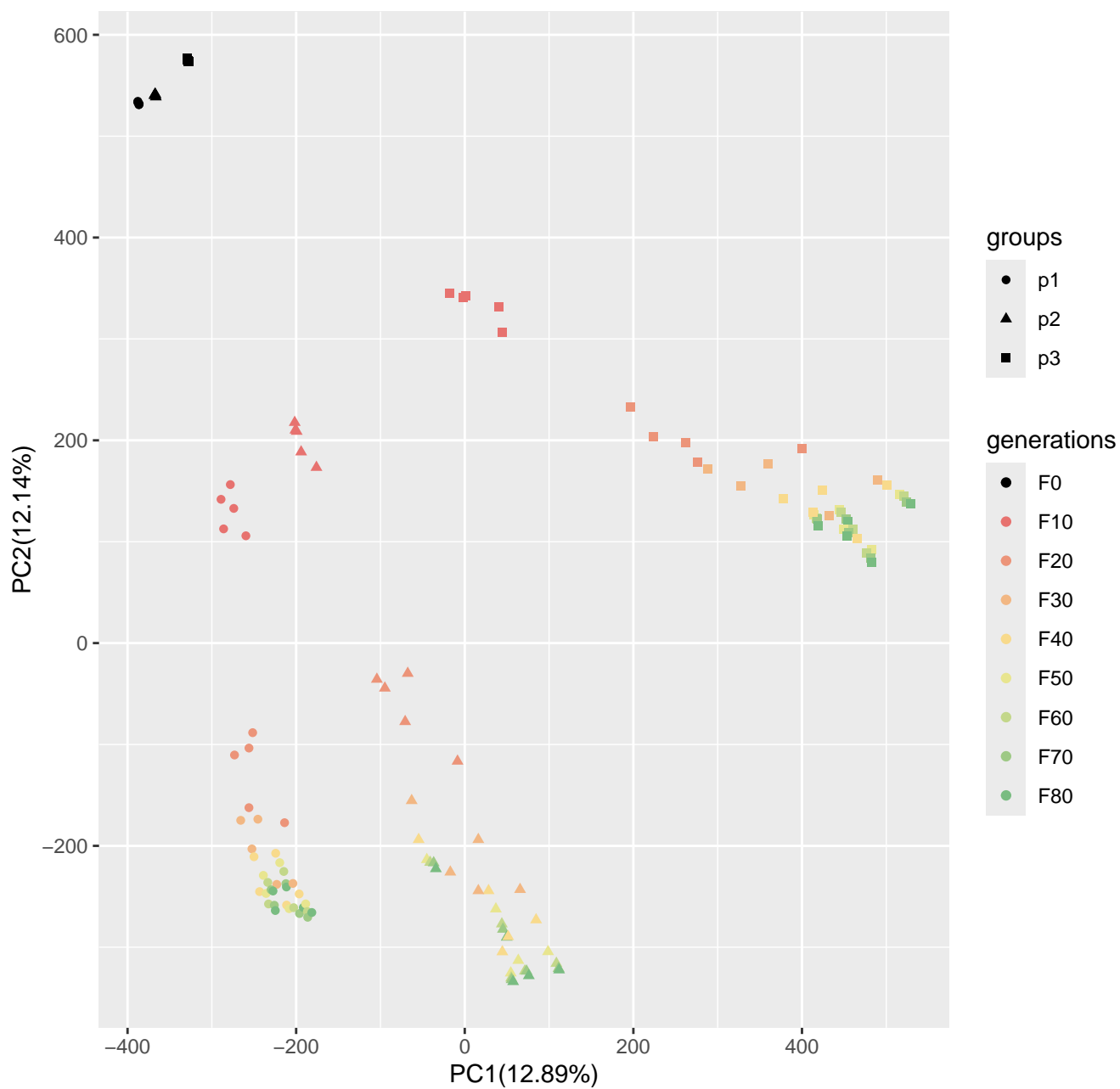
Run5_popsiz1250_n400_10loci_s10
