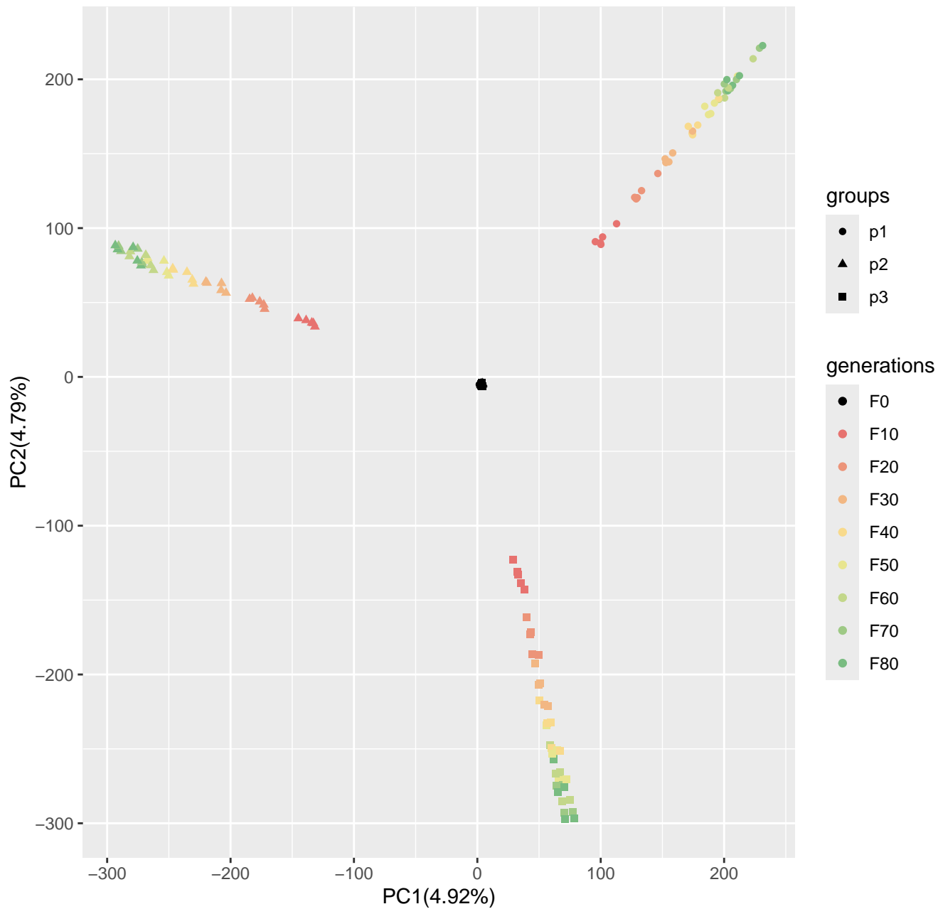
Run4_popsizel250_n400_5000loci_s100
