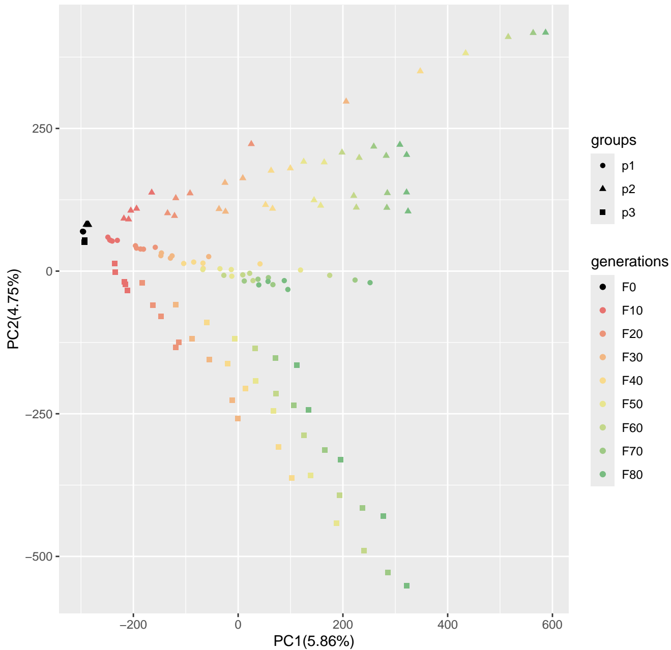
Run10_popsizel250_n2500_100loci_s10
