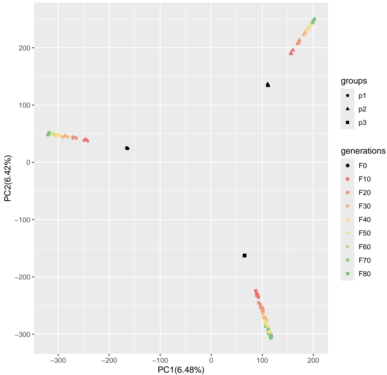
Run8_popsizel250_n400_5000loci_s100
