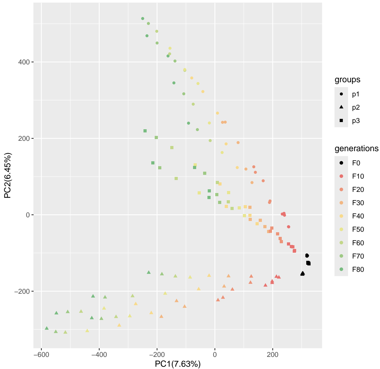
Run1_popsizel250_n1200_100loci_s10
