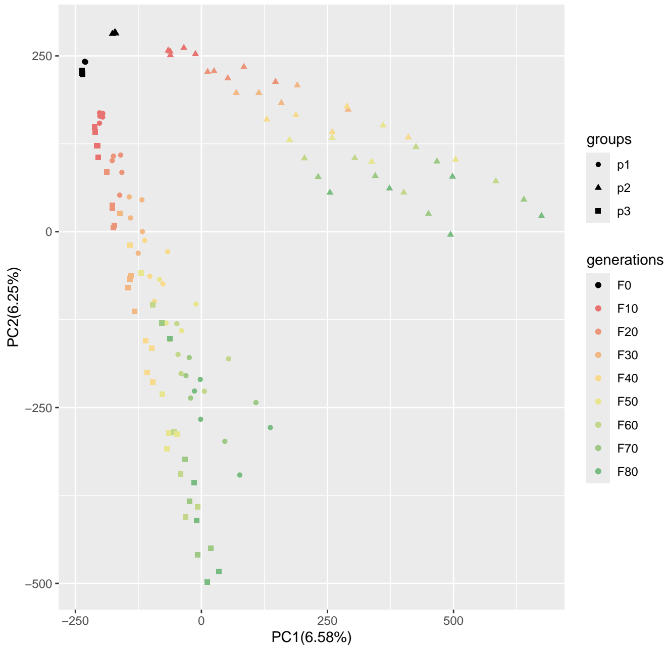
Run5_popsizel250_n800_100loci_s10
