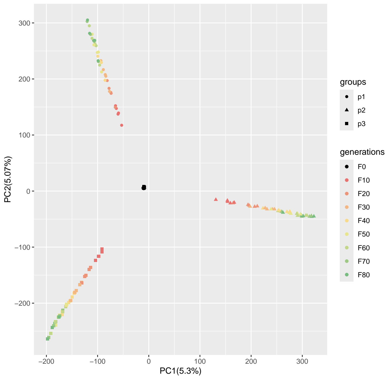
Run4_popsiz1250_n400_1000loci_s50
