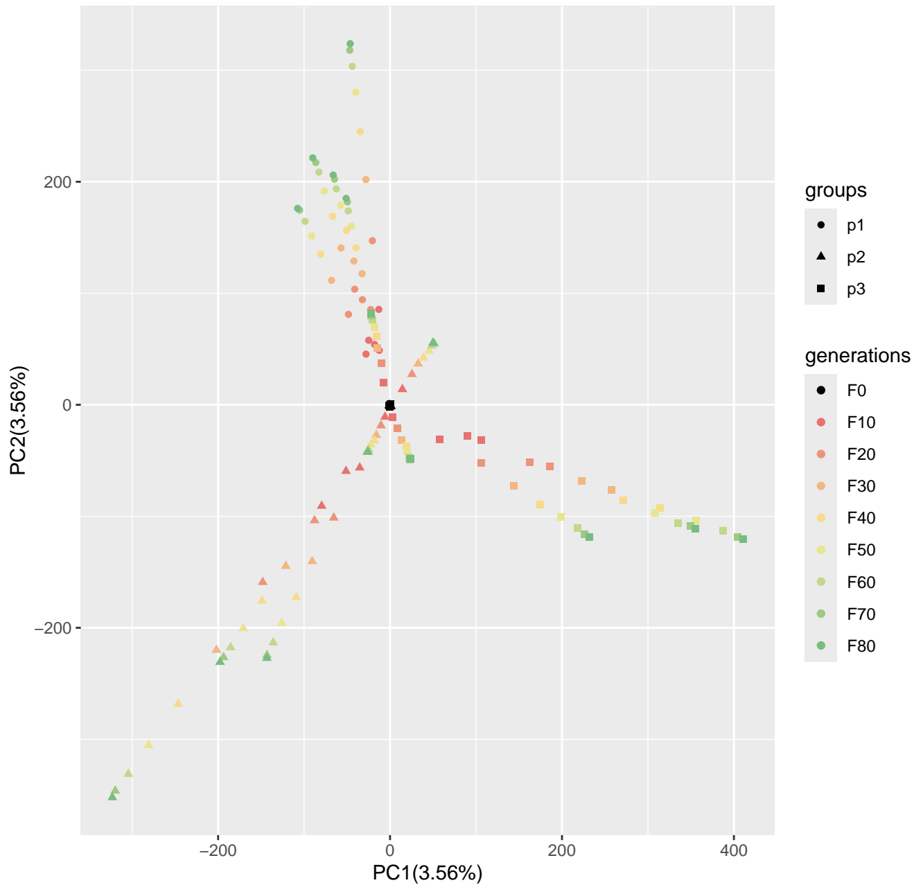
Run5_popsizel250_n400_1000loci_s10
