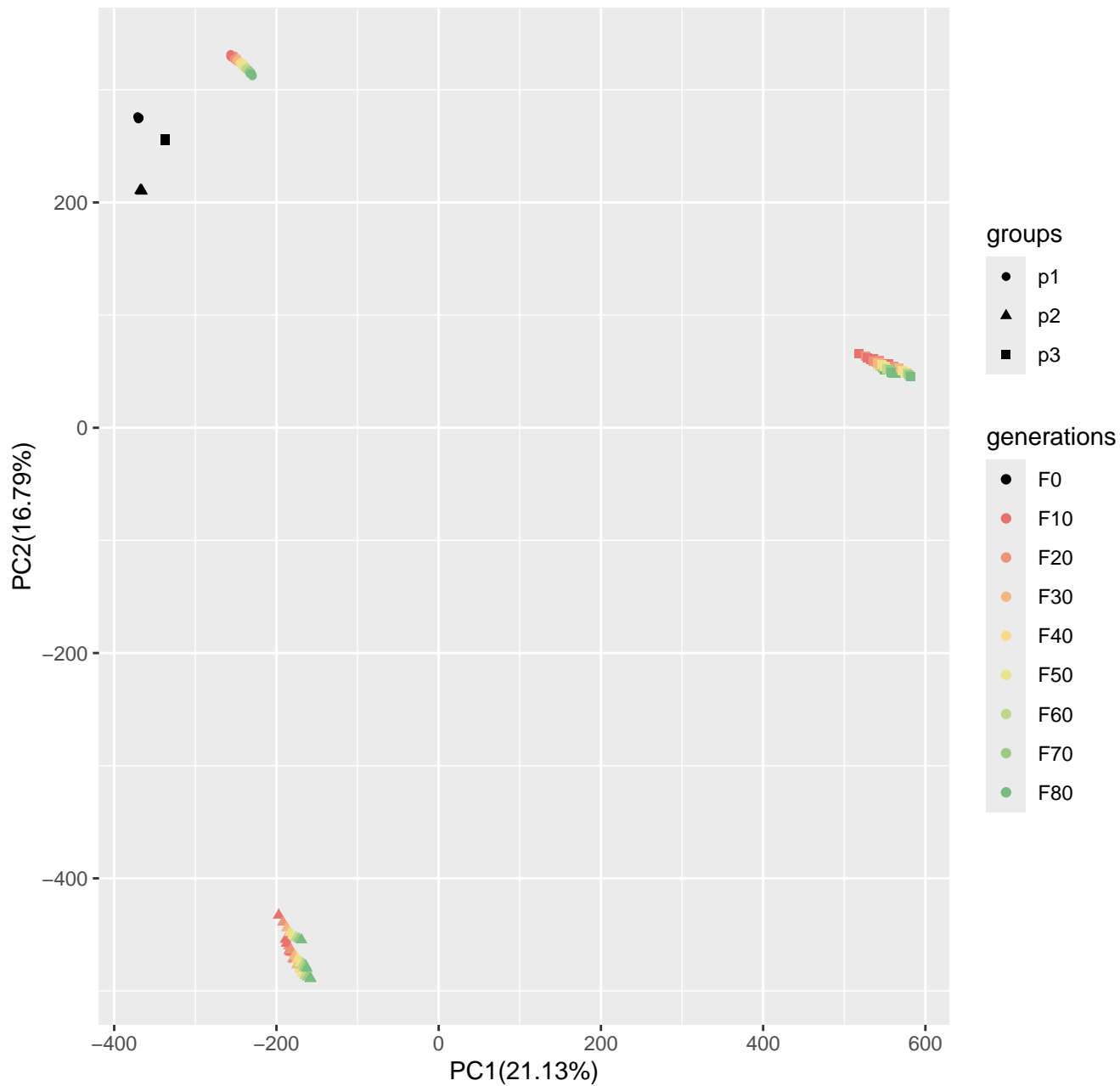
Run8_popsizel250_n400_10loci_s50
