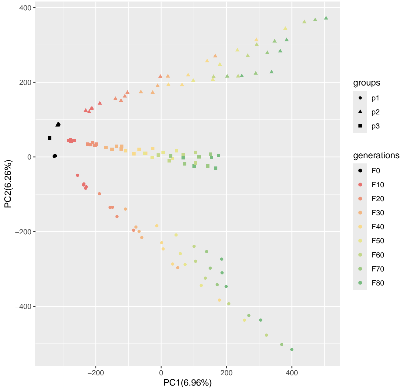
Run10_popsiz1250_n800_100loci_s10
