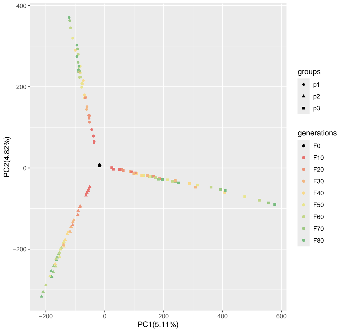
Run1_popsizel250_n400_20000loci_s50
