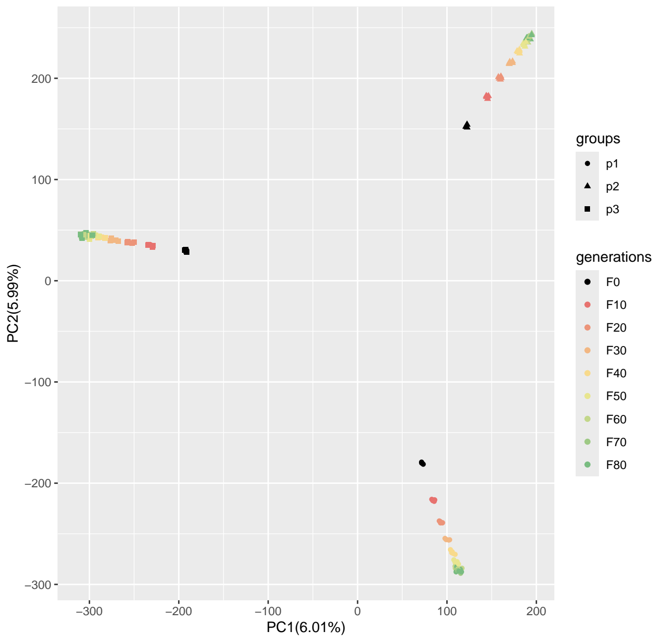
Run1_popsizel250_n400_20000loci_s100
