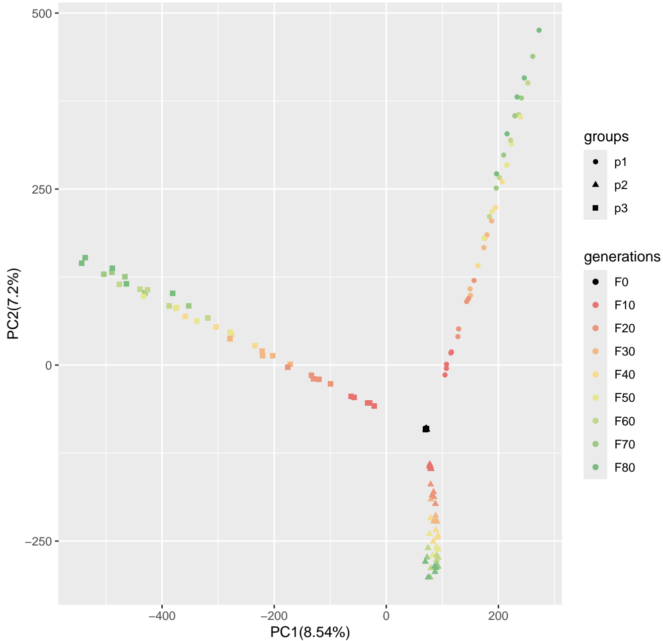
Run5_popsizel250_n400_5000loci_s50
