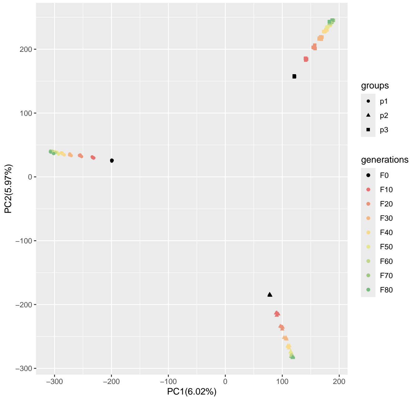
Run2_popsizel250_n400_10000loci_s50
