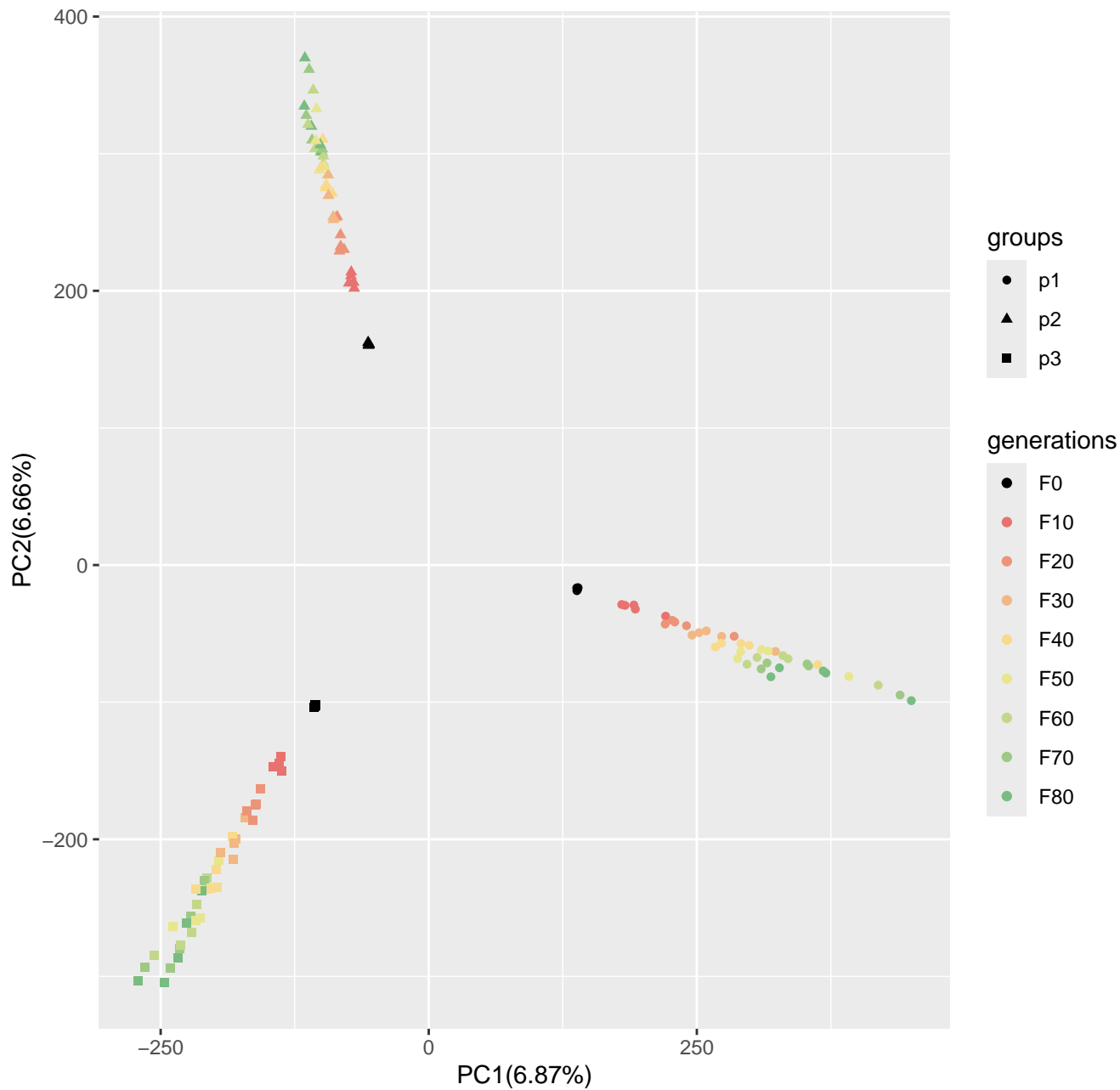
Run10_popsizel250_n400_10000loci_s50
