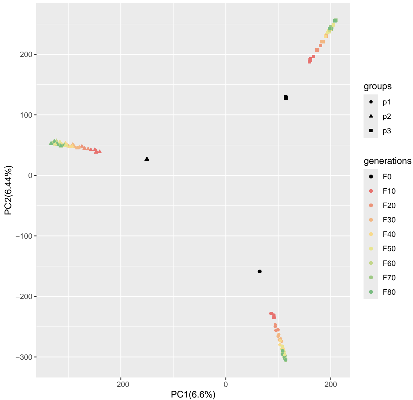
Run3_popsizel250_n400_1000loci_s50
