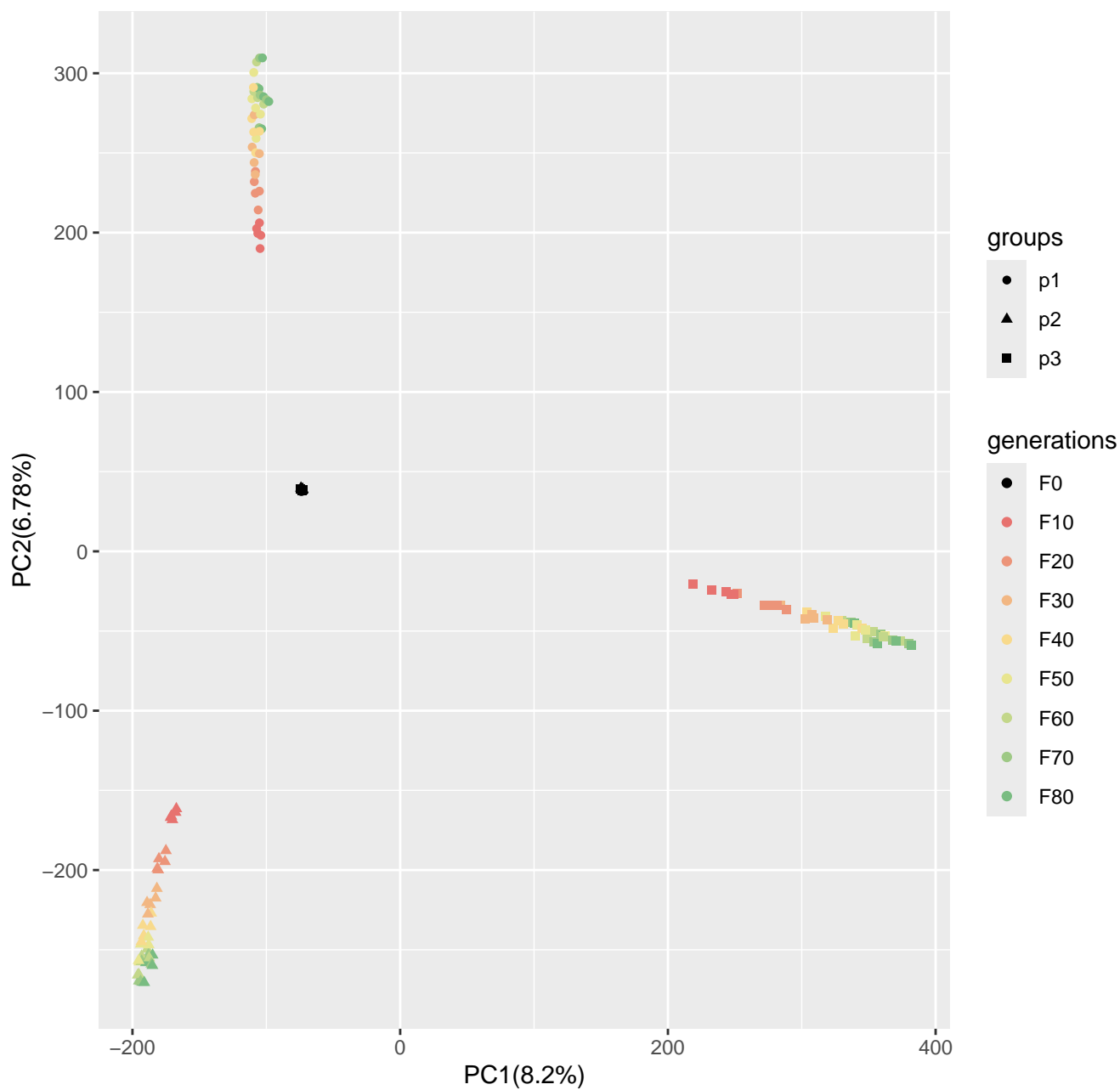
Run10_popsizel250_n400_1000loci_s100
