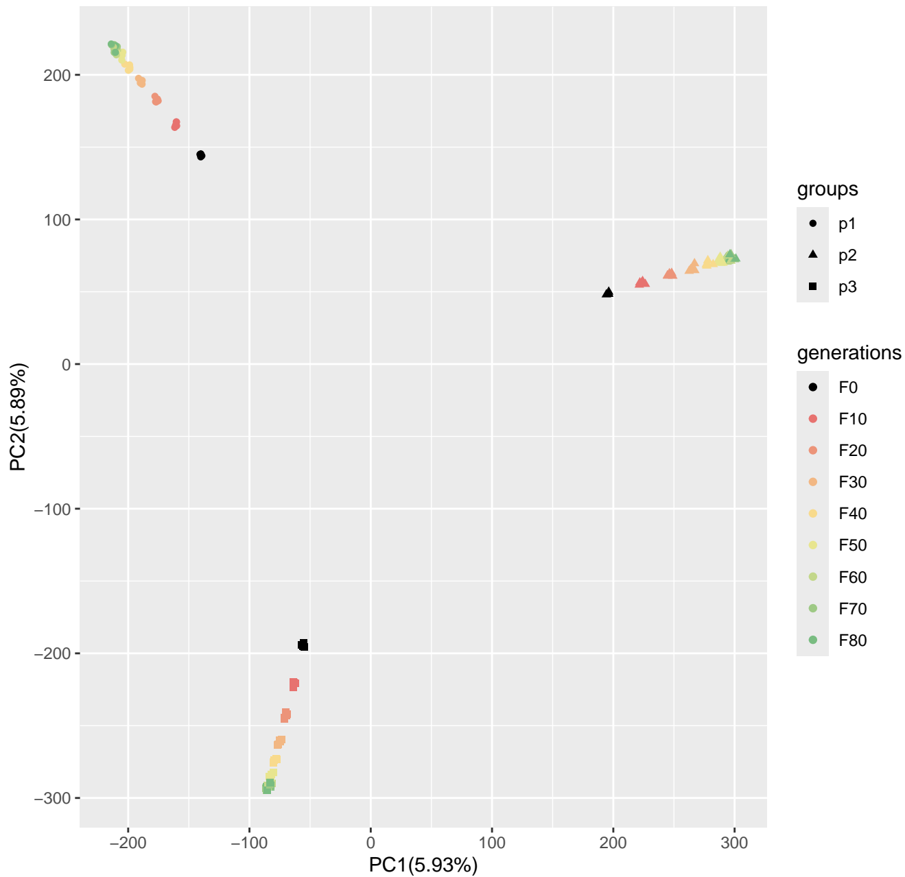
Run4_popsizel250_n400_5000loci_s10
