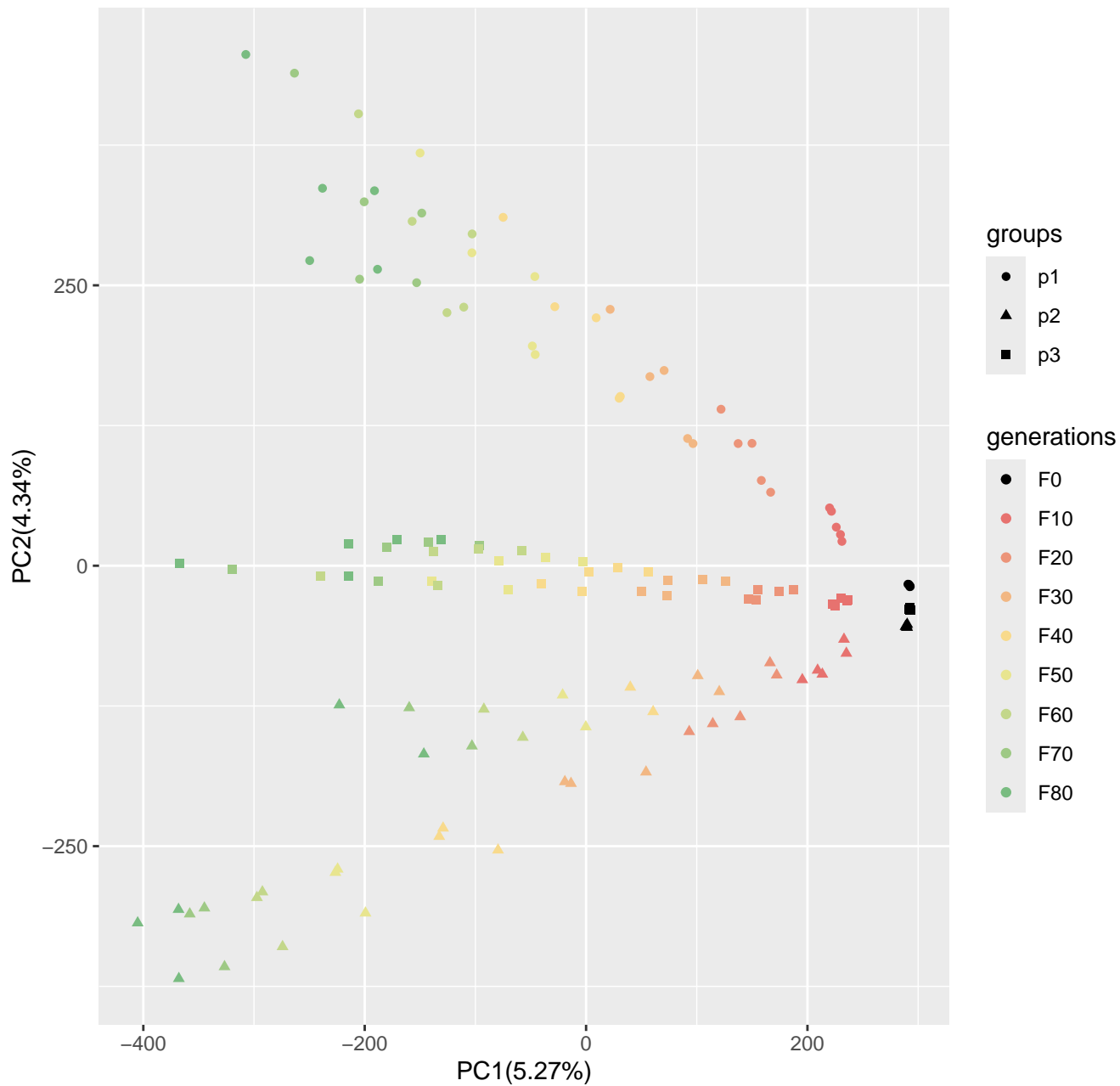
Run8_popsizel2500_n2500_100loci_s10
