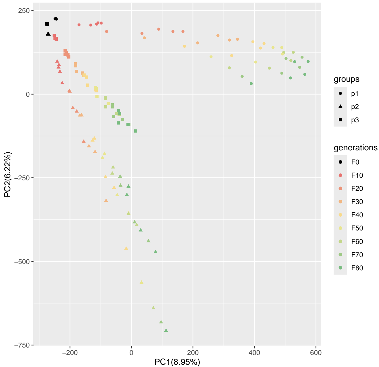
Run3_popsizel250_n1200_100loci_s10
