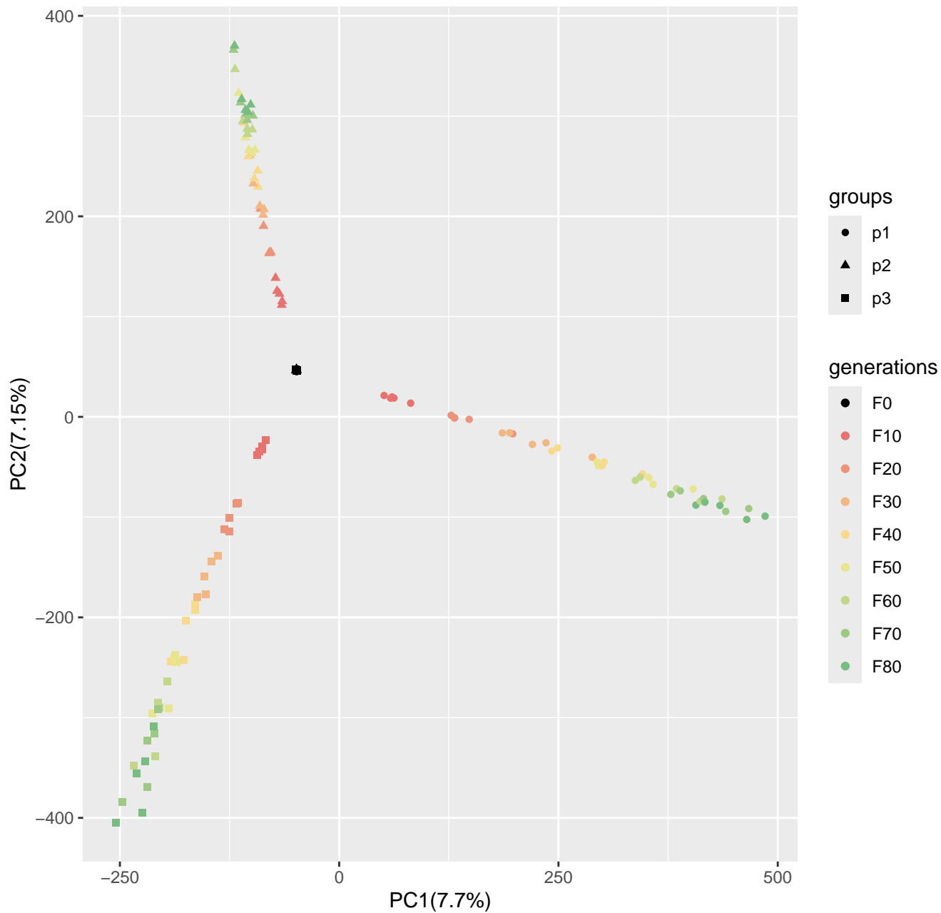
Run7_popsizel250_n400_5000loci_s50
