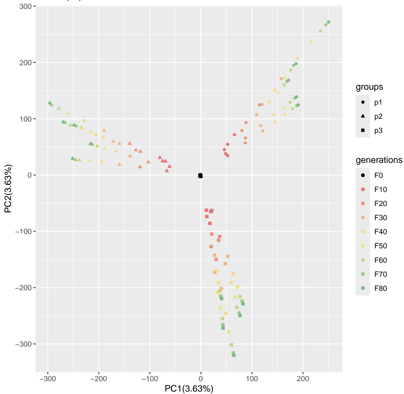
Run1_popsizel250_n400_10000loci_s50
