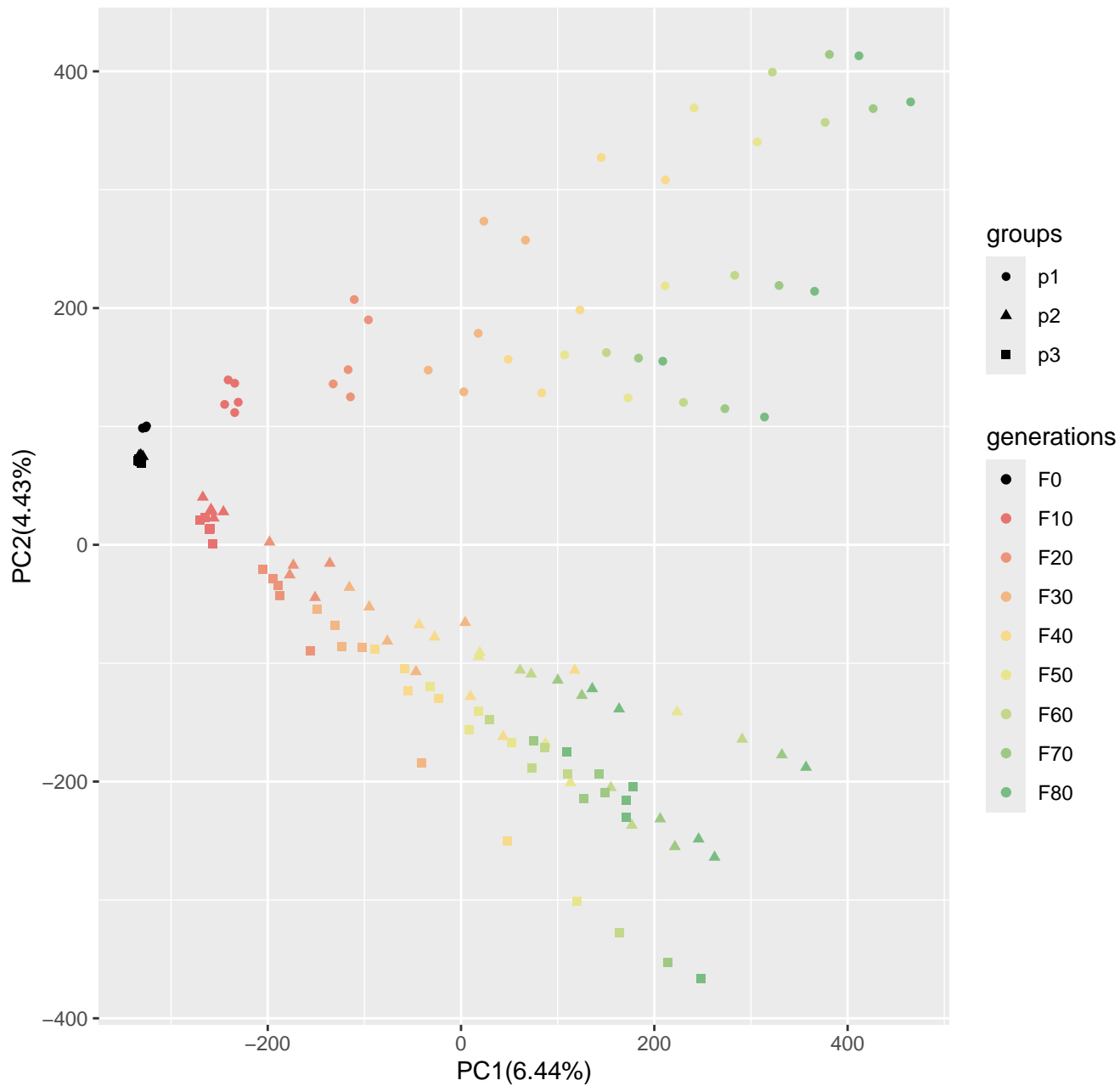
Run2_popsizel250_n2500_100loci_s10
