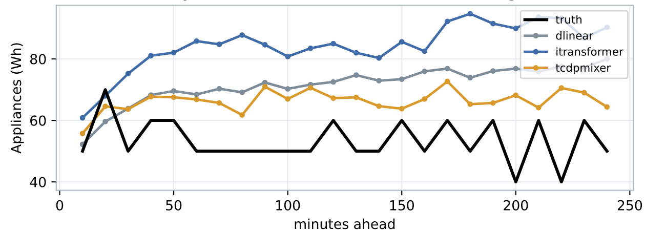
Best day: 2016-05-17 · forecast start noon 12:00
