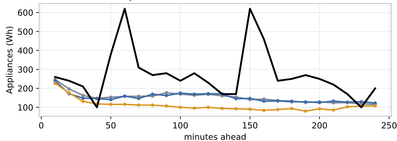
Worst day: 2016-05-13 · forecast start evening 18:00
