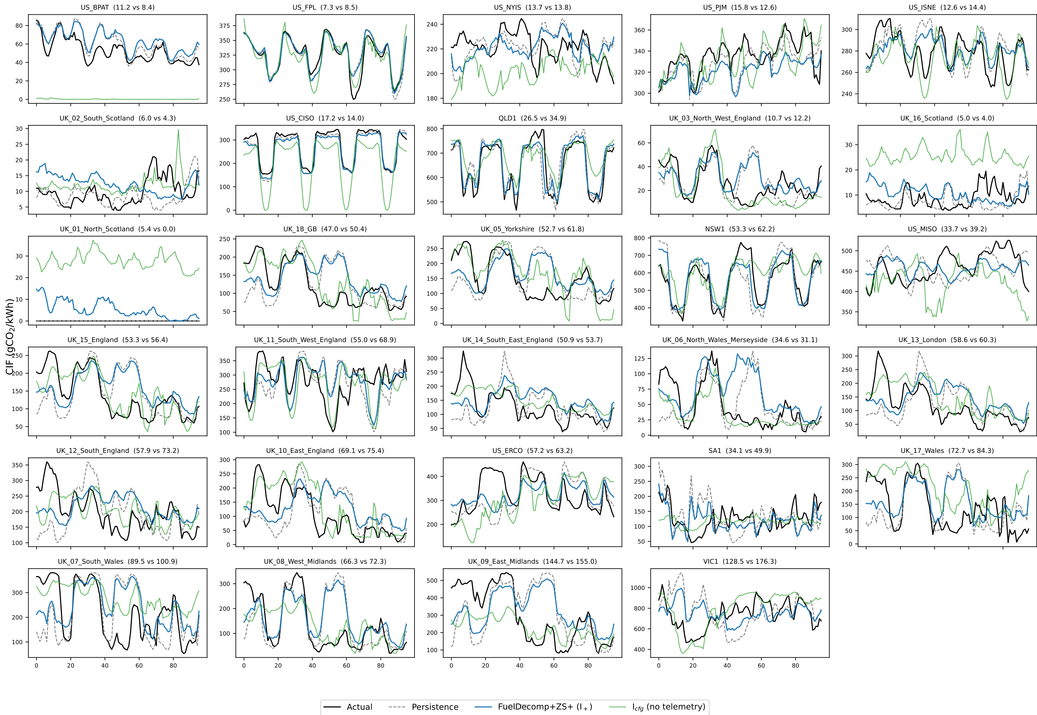
Day-ahead CIF, 29 regions (96 h spliced from 4 origins, seed 0) — panel title: model vs persistence MAE
