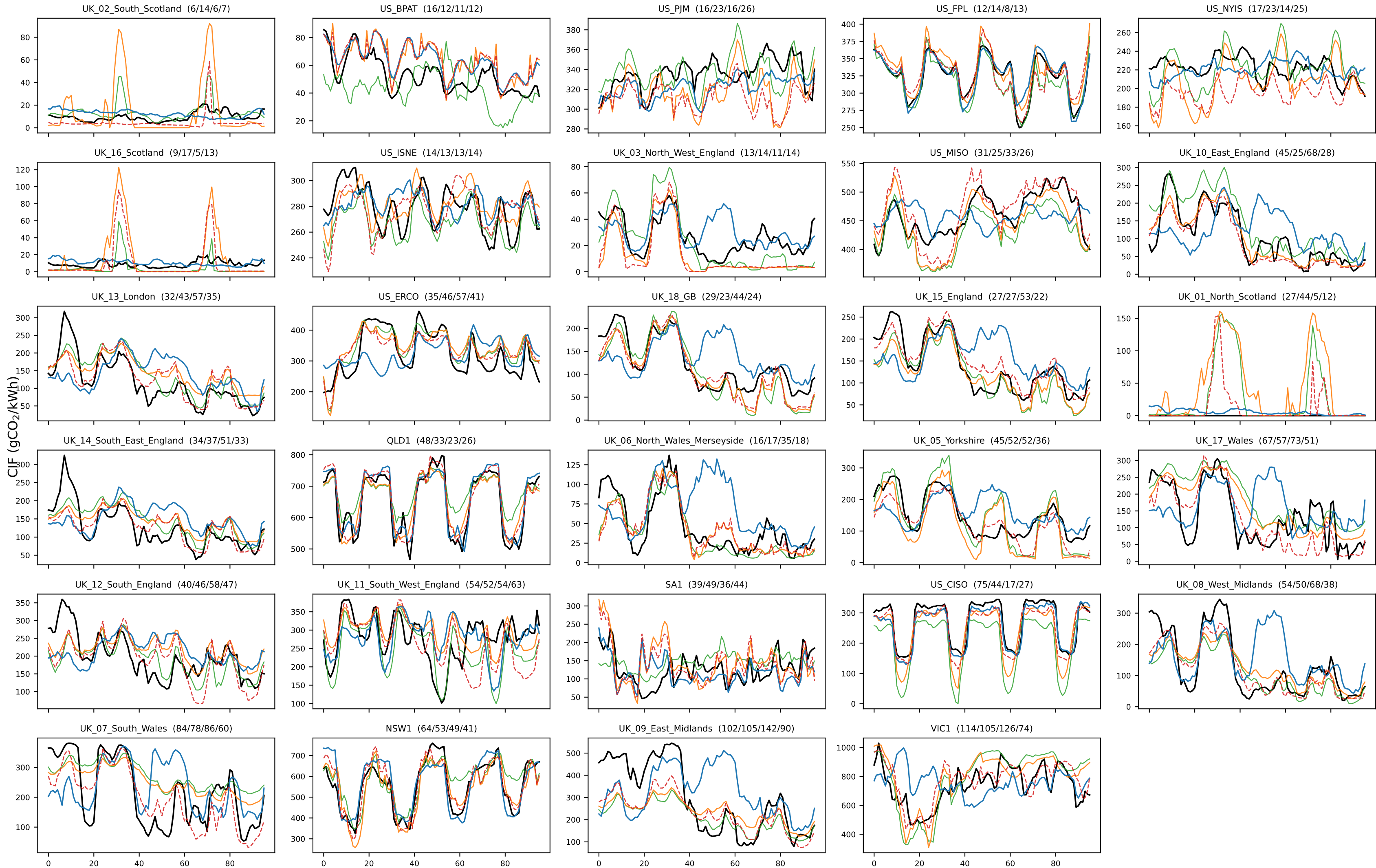
Day-ahead CIF, 29 regions — the information ladder (96 h spliced from 4 origins, seed 0) panel title: I_{cfg} / I_0 / I_+ / I_S MAE over the plotted 96 h; panels sorted by I_{cfg}
