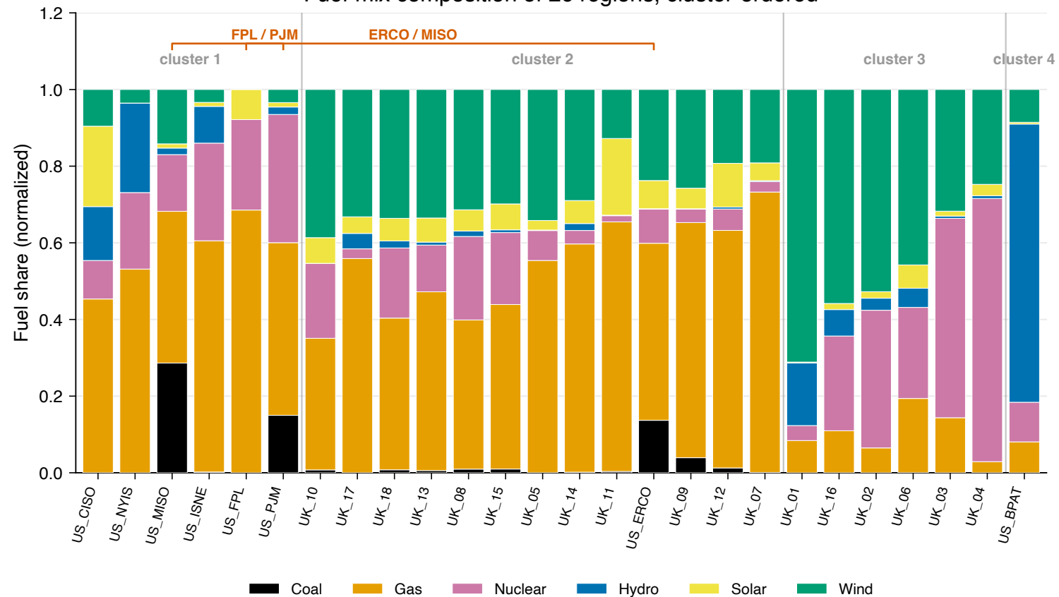
Fuel-mix composition of 26 regions, cluster-ordered
