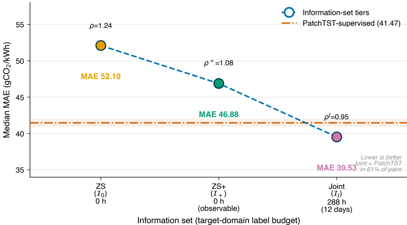
Performance ladder by information-set tier (29-region LORO)
