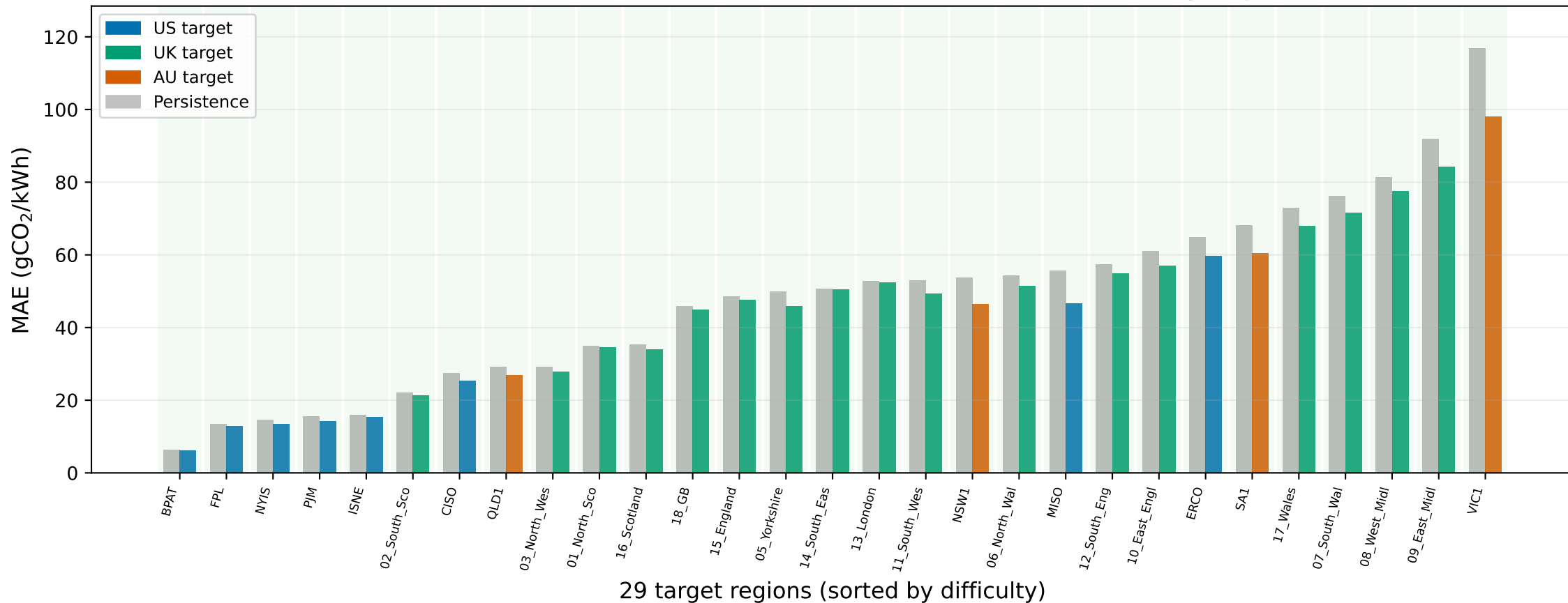
Cross-domain transfer: TransCIF ZS+ vs persistence on every region
