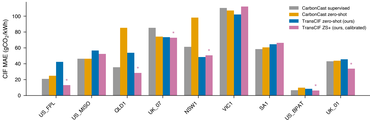
CarbonCast under domain shift: TransCIF ZS+ wins 6/9 zero-shot
